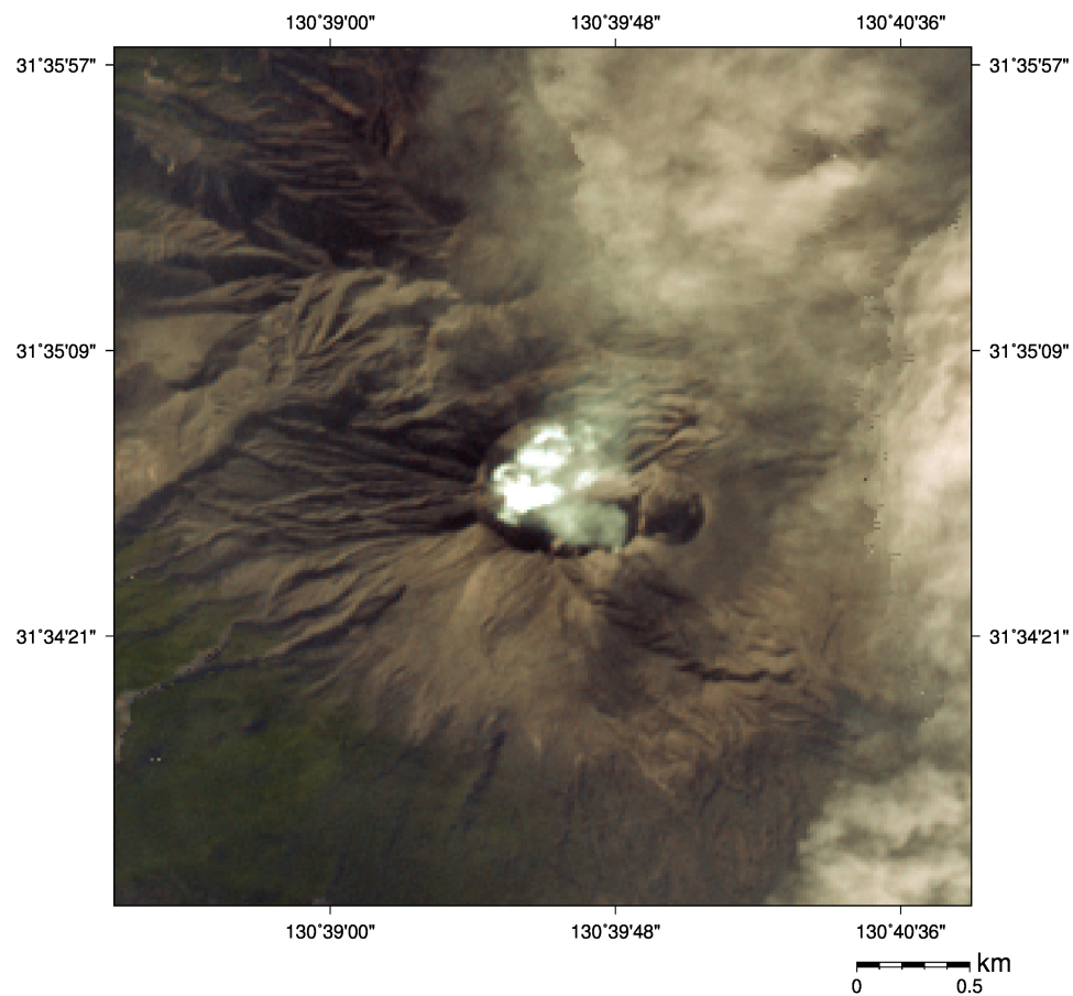
Mt. Sakurajima captured by ASTER VNIR on Feb 11, 2020 (UTC 02:11, Visible image (15m resolution))
