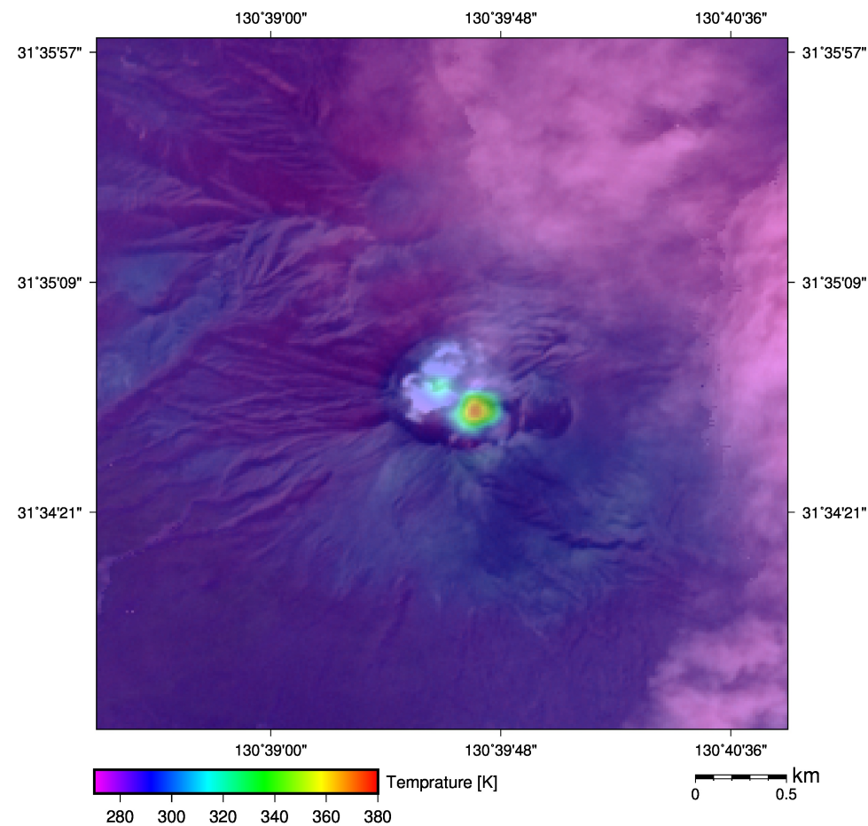
Mt. Sakurajima captured by ASTER TIR on Feb 11, 2020 (UTC 02:11, Thermal image (90m resolution) overlaid on the visible image)
