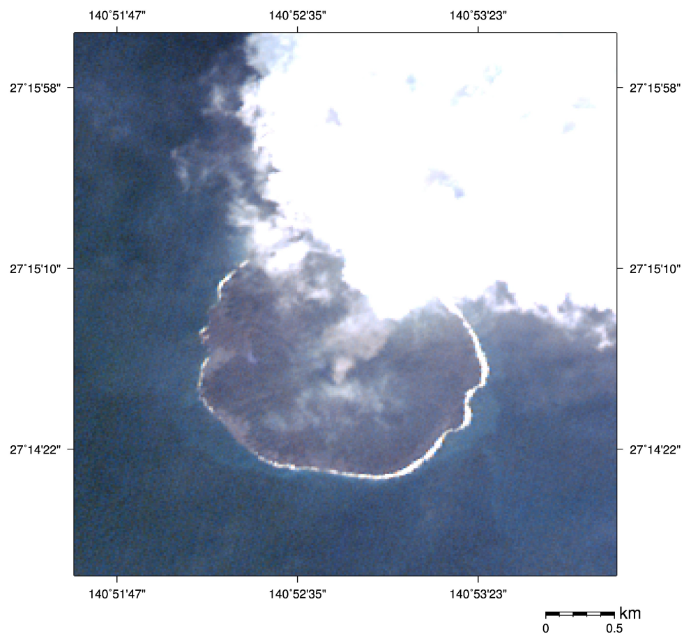
Nishinoshima captured by ASTER VNIR on Dec 17, 2019 (UTC 01:23, Visible image (15m resolution))
