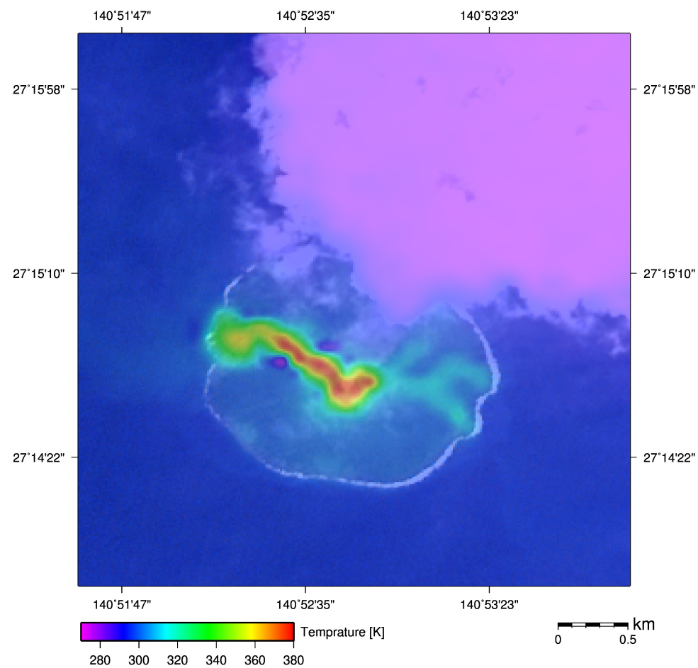
Nishinoshima captured by ASTER TIR on Dec 17, 2019 (UTC 01:23, Thermal image (90m resolution) overlaid on the visible image)
