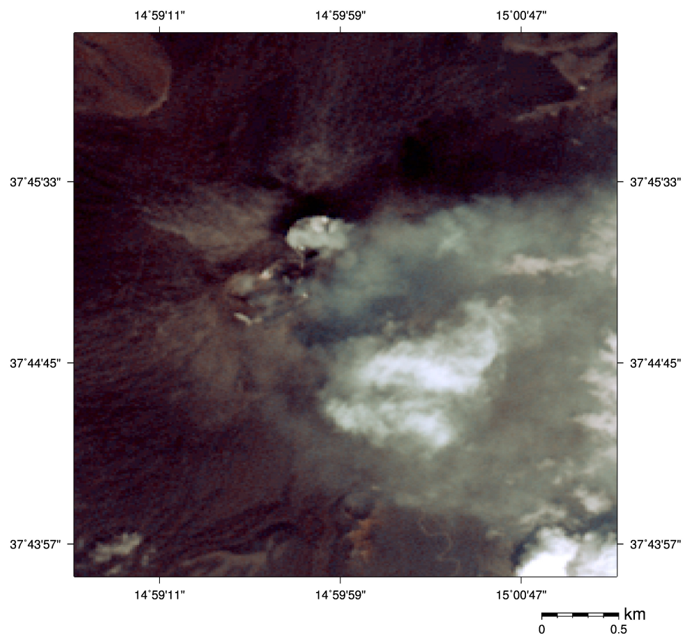
Mount Etna captured by ASTER VNIR on Sep 17, 2019 (UTC 09:53, Visible image (15m resolution))
