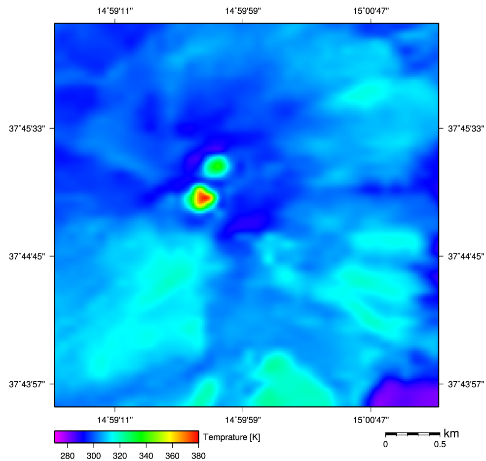
Mount Etna captured by ASTER TIR on Sep 17, 2019 (UTC 09:53, Thermal image (90m resolution))
