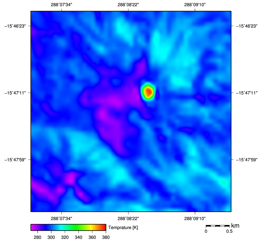
Sabancaya volcano captured by ASTER TIR on Sep 01, 2019 (UTC 15:04, Thermal image (90m resolution))
