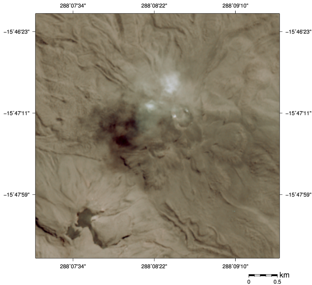
Sabancaya volcano captured by ASTER VNIR on Sep 01, 2019 (UTC 15:04, Visible image (15m resolution))
