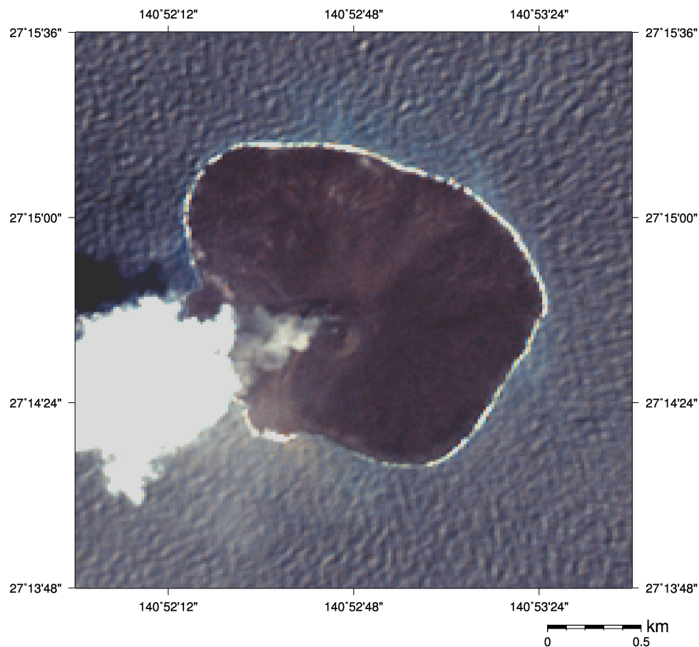
Nishinoshima captured by ASTER VNIR on May 01, 2017 (UTC 01:23, Visible image (15m resolution))
