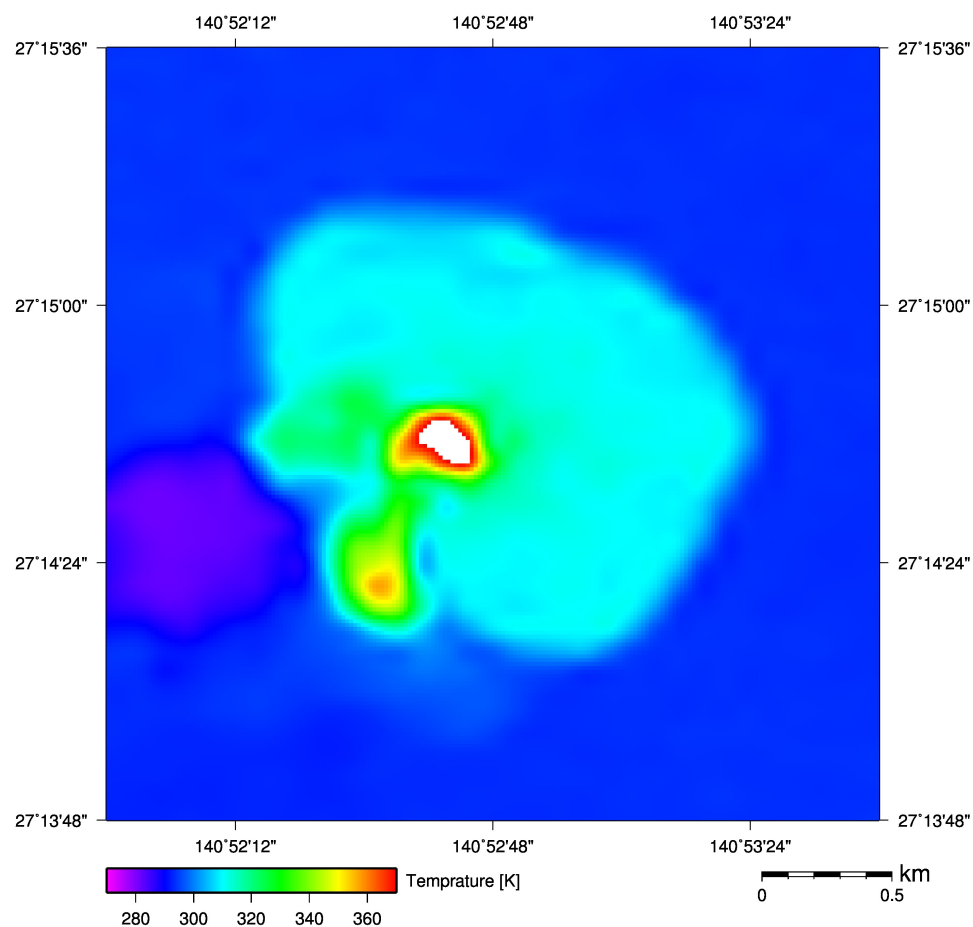
Nishinoshima captured by ASTER TIR on May 01, 2017 (UTC 01:23, Thermal image (90m resolution))
