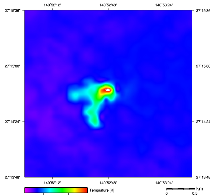
Nishinoshima captured by ASTER TIR on Apr 27, 2017 (UTC 12:46, Thermal image (90m resolution))
