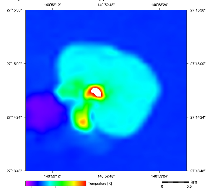
Nishinoshima captured by ASTER TIR on May 01, 2017 (UTC 01:23, Thermal image (90m resolution))
