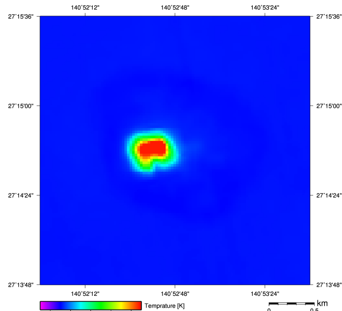
Nishinoshima captured by Landsat-8 TIRS on Apr 19, 2017 (UTC 12:27, Thermal image (100m resolution))
