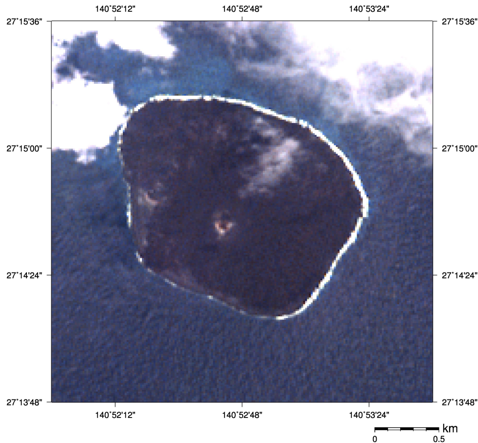
Nishinoshima captured by ASTER VNIR on Apr 15, 2017 (UTC 01:23, Visible image (15m resolution))
