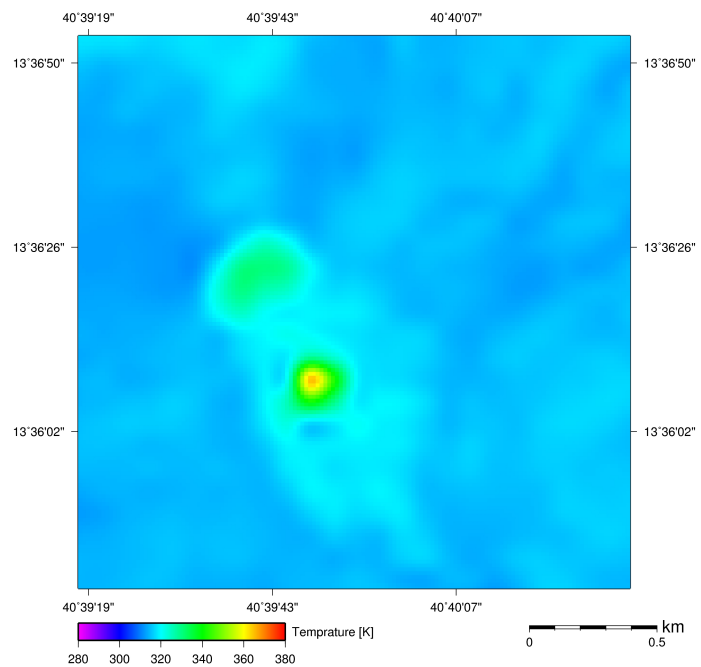
ASTER TIR on Jan 02, 2017 (UTC 07:56)
