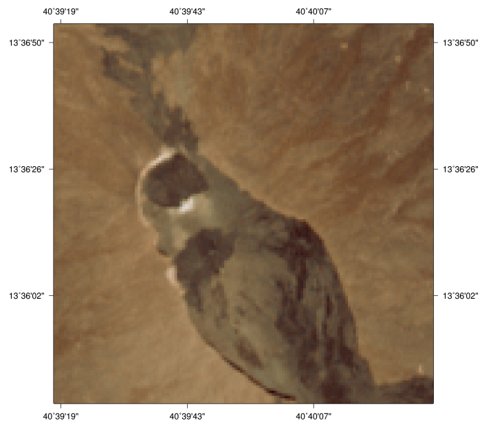
ASTER VNIR on Jan 02, 2017 (UTC 07:56)
