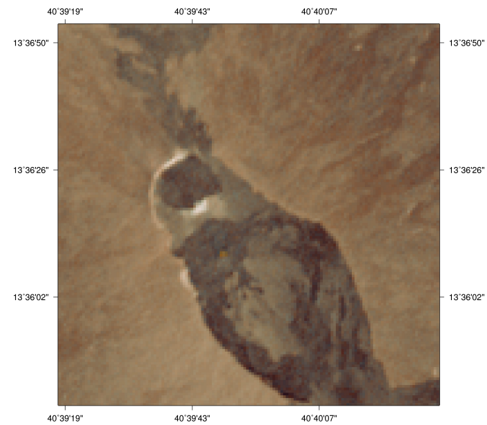
ASTER VNIR on Jan 18, 2017 (UTC 07:56)
