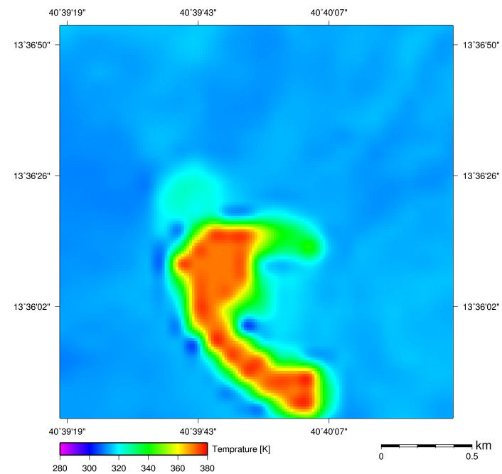
ASTER TIR on Jan 18, 2017 (UTC 07:56)
