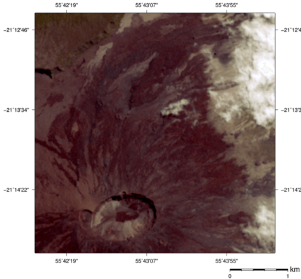
Piton de la Fournaise Volcano captured by ASTER VNIR on Sep 19, 2016 (UTC 06:33, Visible image (15m resolution))
