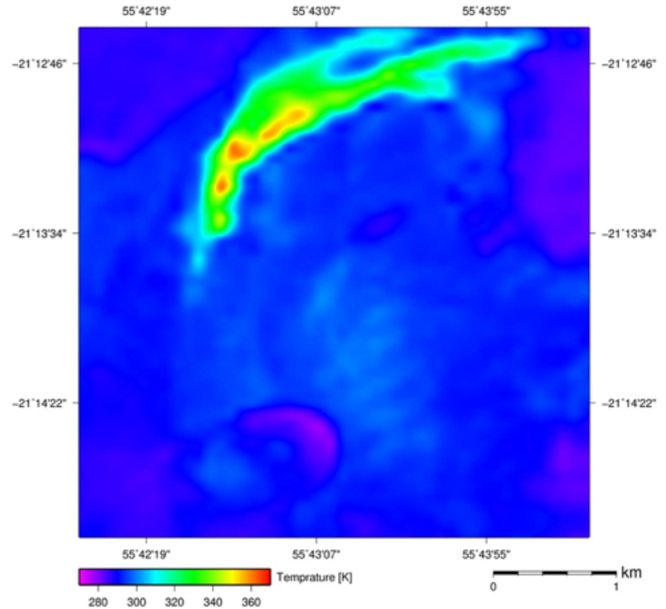
Piton de la Fournaise Volcano captured by ASTER TIR on Sep 19, 2016 (UTC 06:33, Thermal image (90m resolution))
