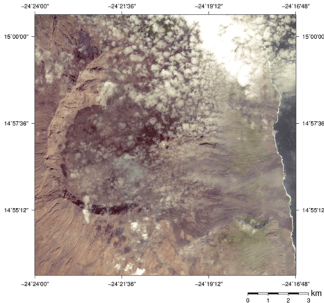
Fogo volcano in República de Cabo Verde captured by Terra ASTER on Dec 18, 2014 (UTC 12:15, Visible image (15m resolution))
