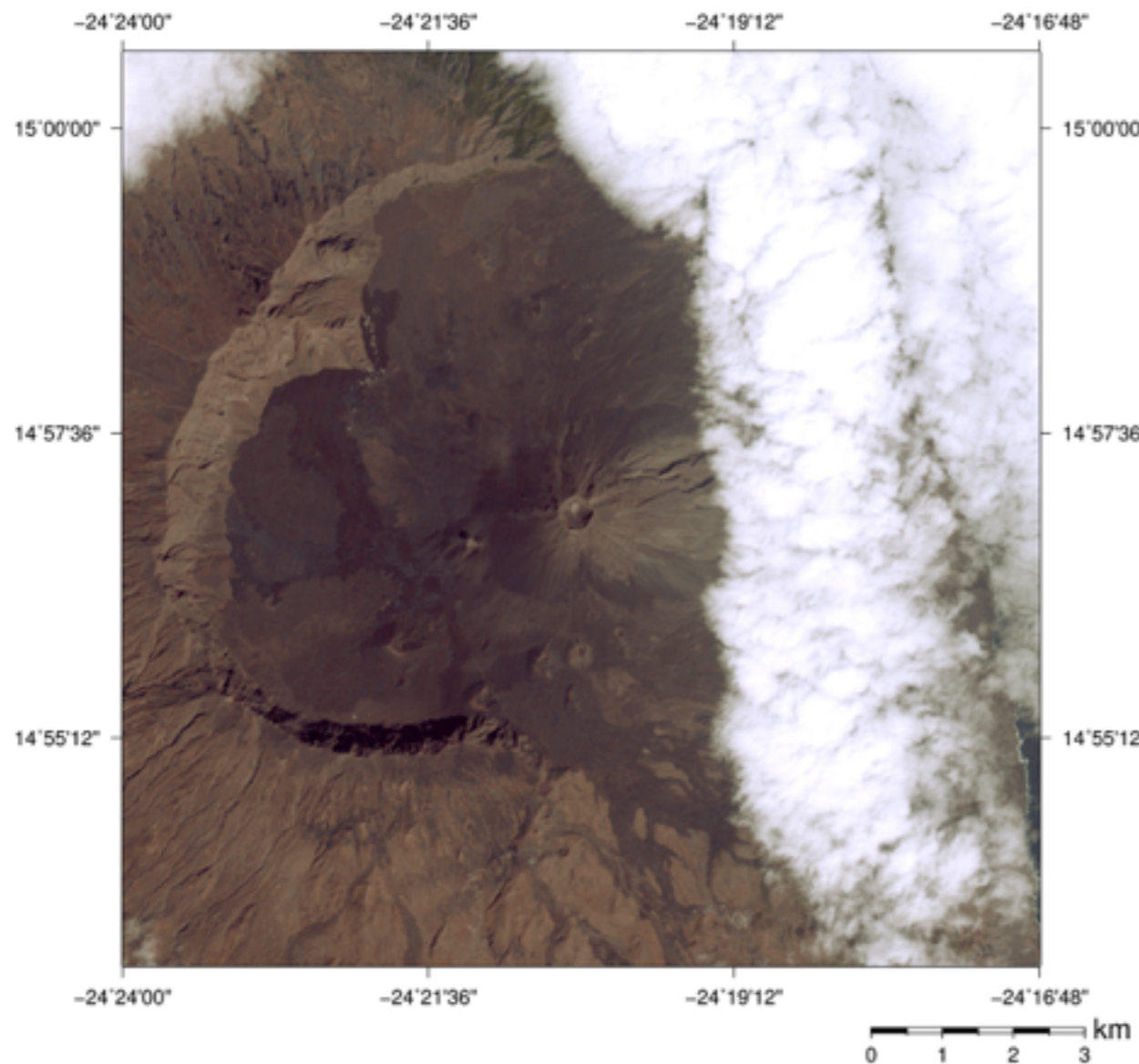
Fogo volcano in República de Cabo Verde captured by Terra ASTER on Feb 4, 2015 (UTC 12:15, Visible image (15m resolution))
