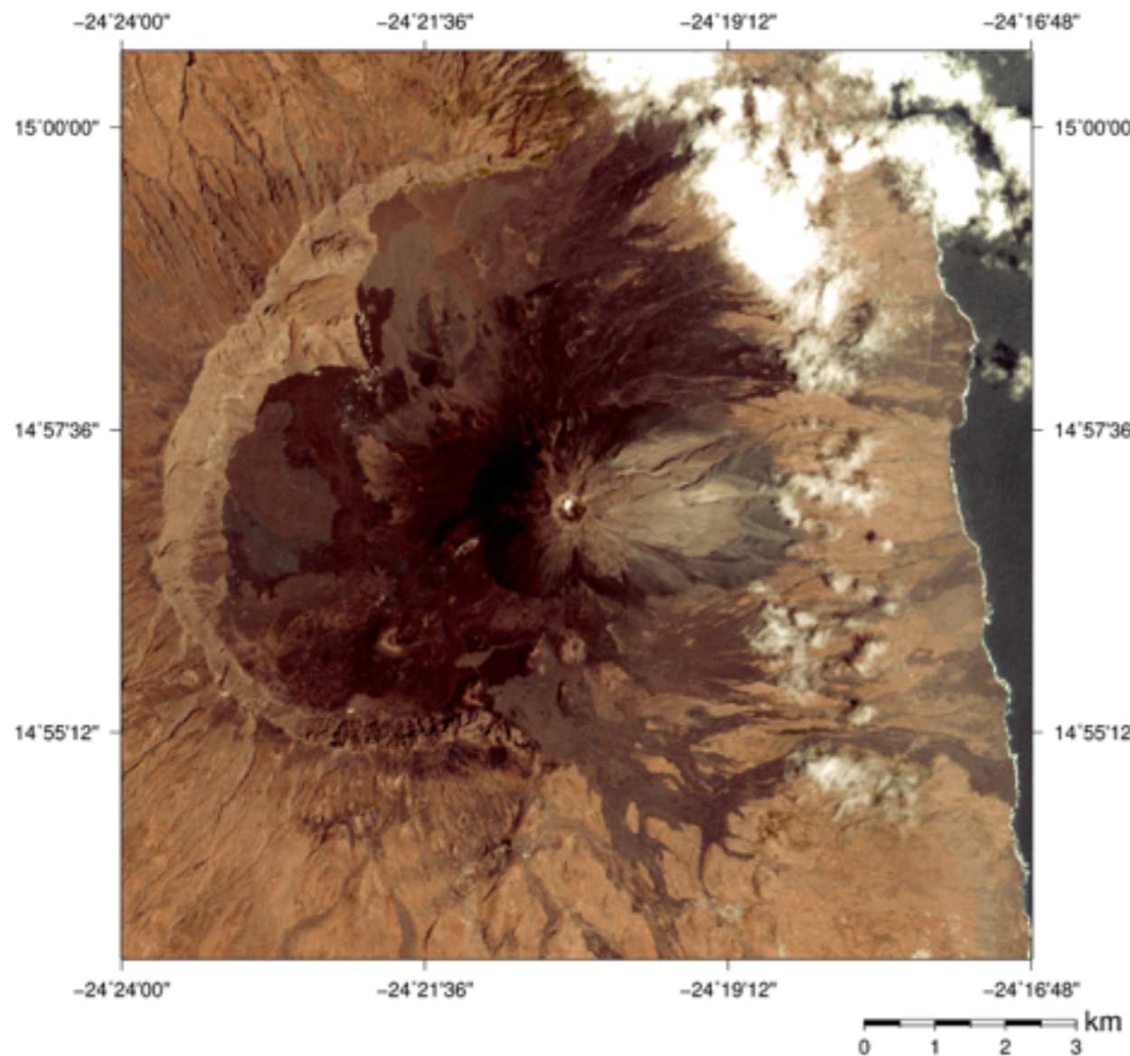
Fogo volcano in República de Cabo Verde captured by Terra ASTER on Mar 26, 2016 (UTC 12:15, Visible image (15m resolution))
