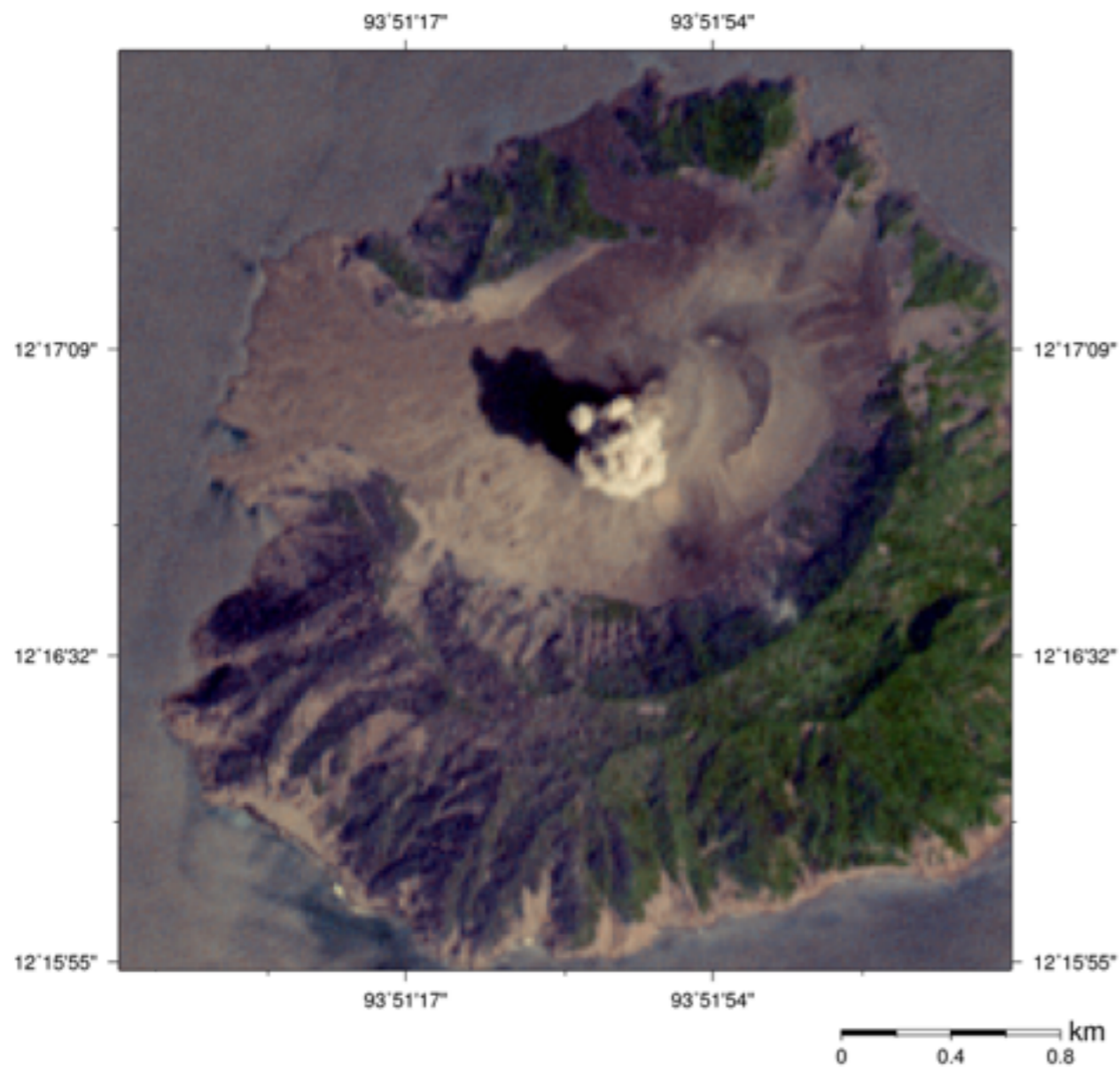
Barren island volcano in India captured by Terra ASTER on Mar 6, 2016 (UTC 4:26, Visible image (15m resolution))
