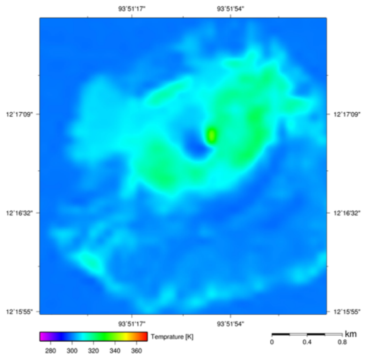
Barren island volcano in India captured by Terra ASTER on Mar 6, 2016 (UTC 4:26, Thermal image (90m resolution))
