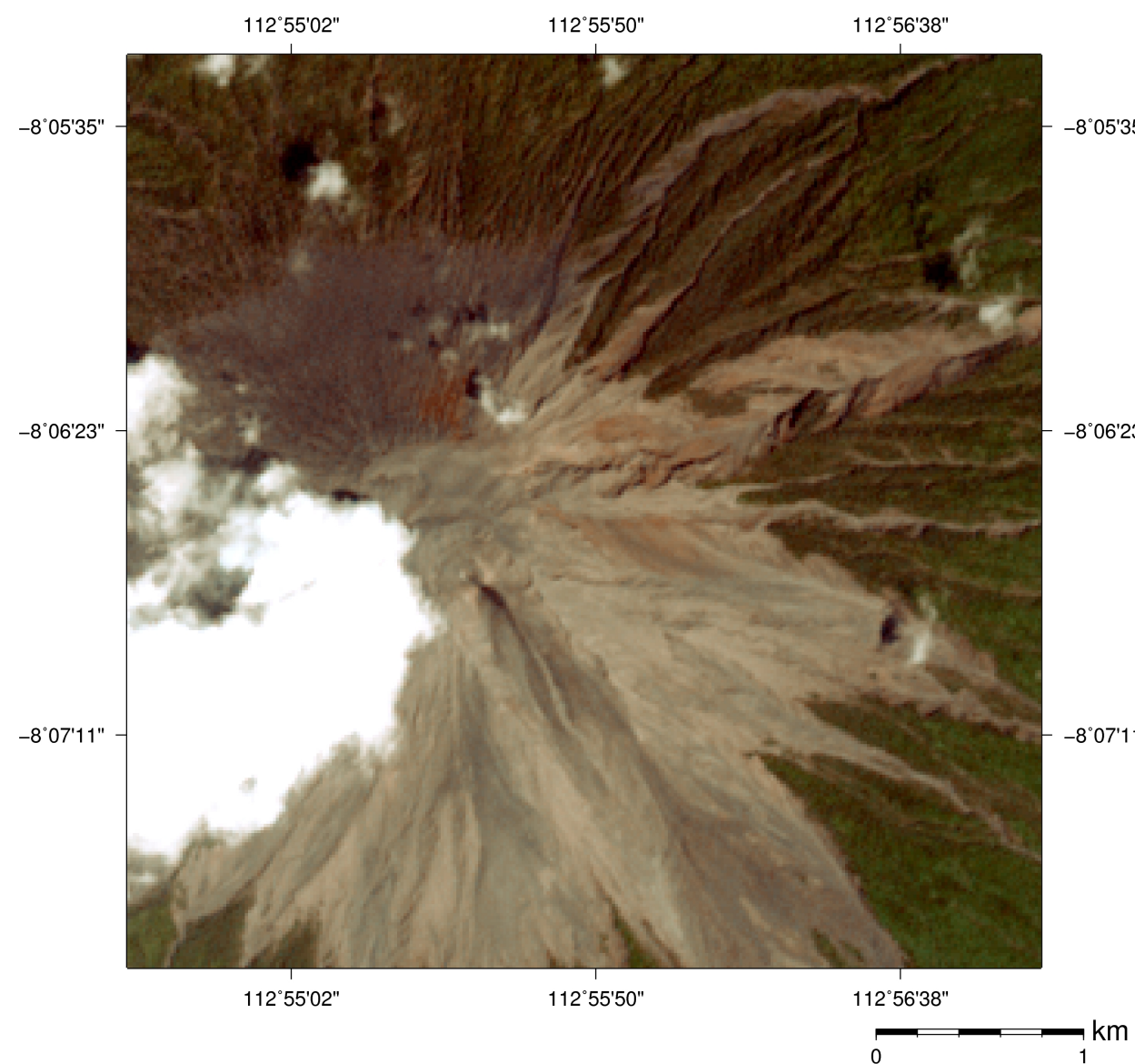
Mt. Semeru in Indonesia captured by Terra ASTER on Dec 1, 2015 (UTC 2:53, visible image (15m resolution))
