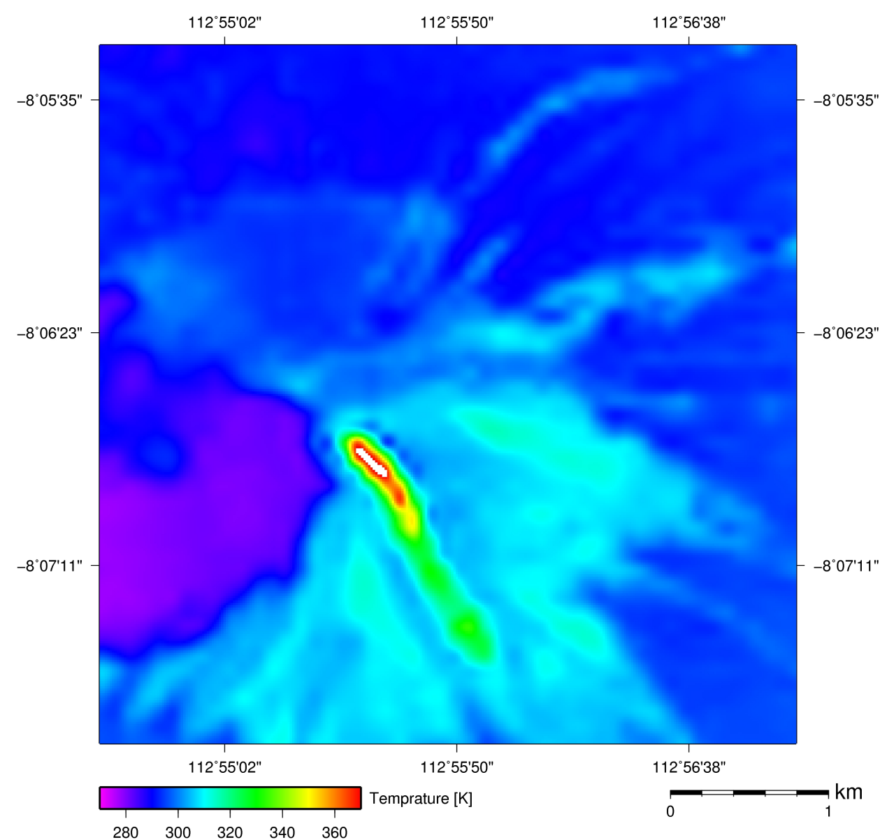
Mt. Semeru in Indonesia captured by Terra ASTER on Dec 1, 2015 (UTC 2:53, Thermal image (90m resolution))
