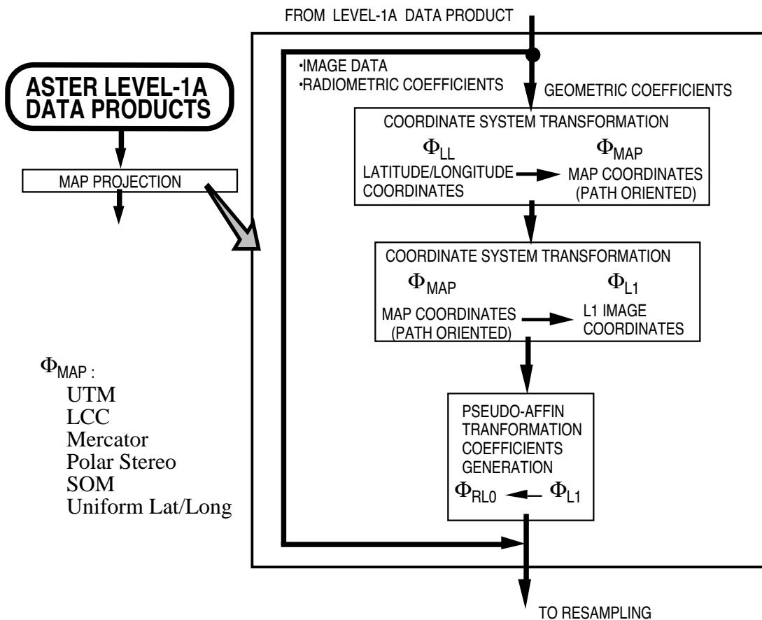
Figure 3-21 Map Projection
