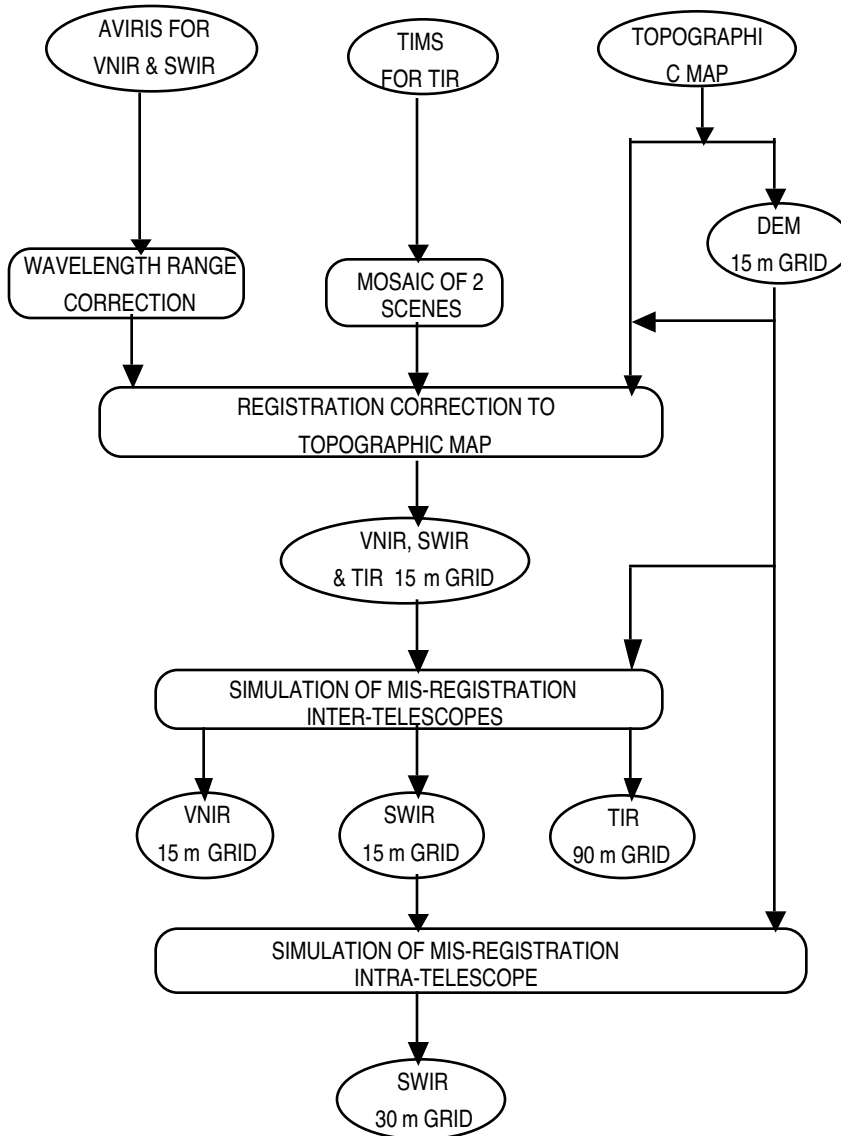
Figure 7-1 Data Processing Flow of Simulation Images
