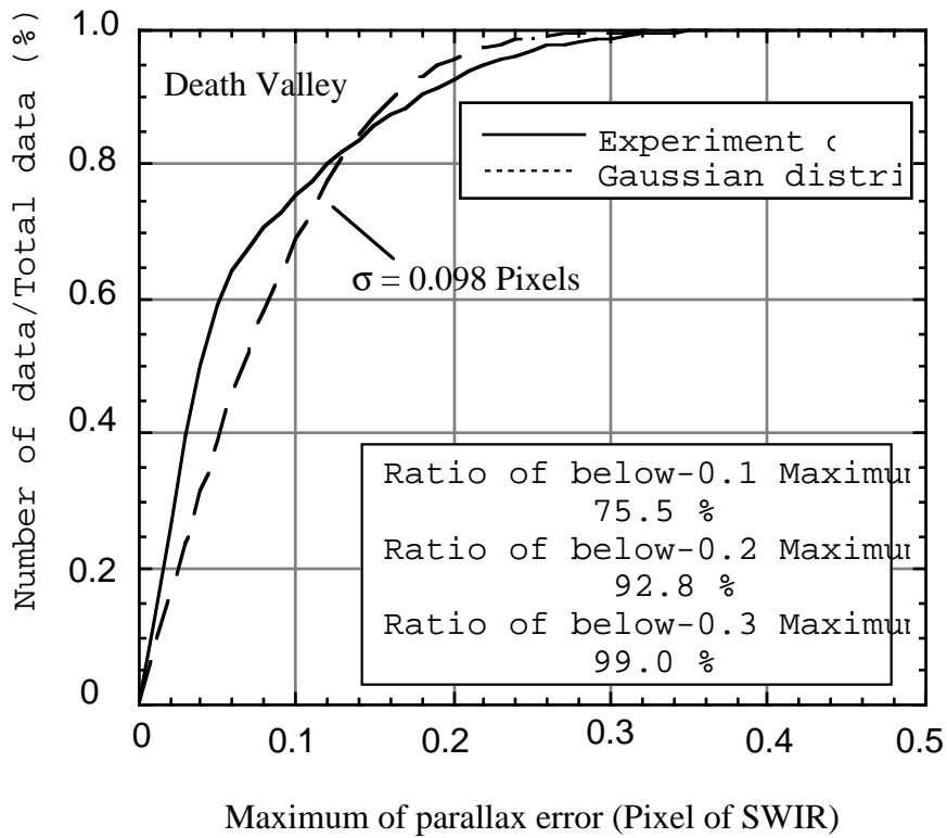
Figure 7-8 SWIR Parallax Correction Error Distribution for Death Valley Image
