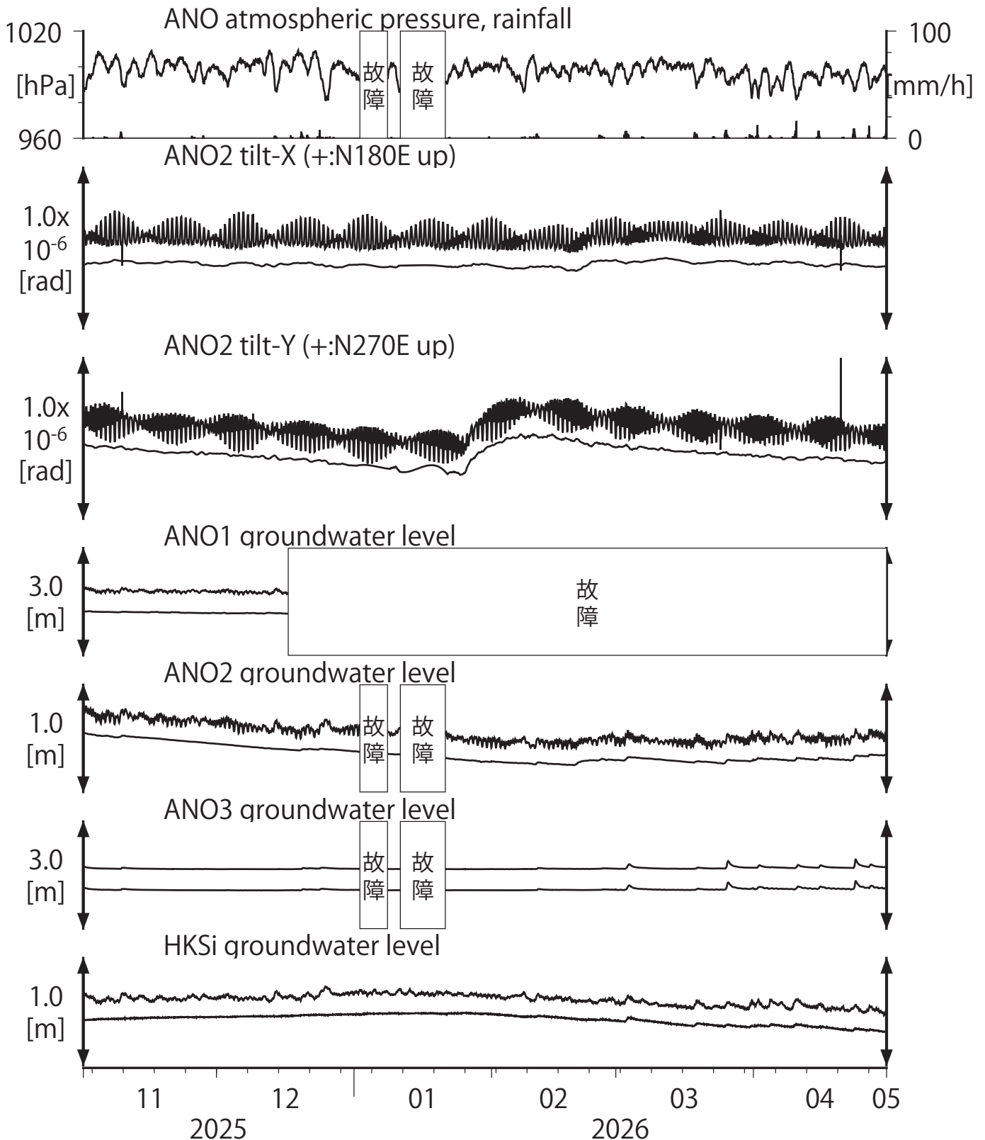
第9図 Tilt and groundwater level at ANO and HKS (時間値) (2025/11/01 00:00 - 2026/05/01 00:00 (JST))
