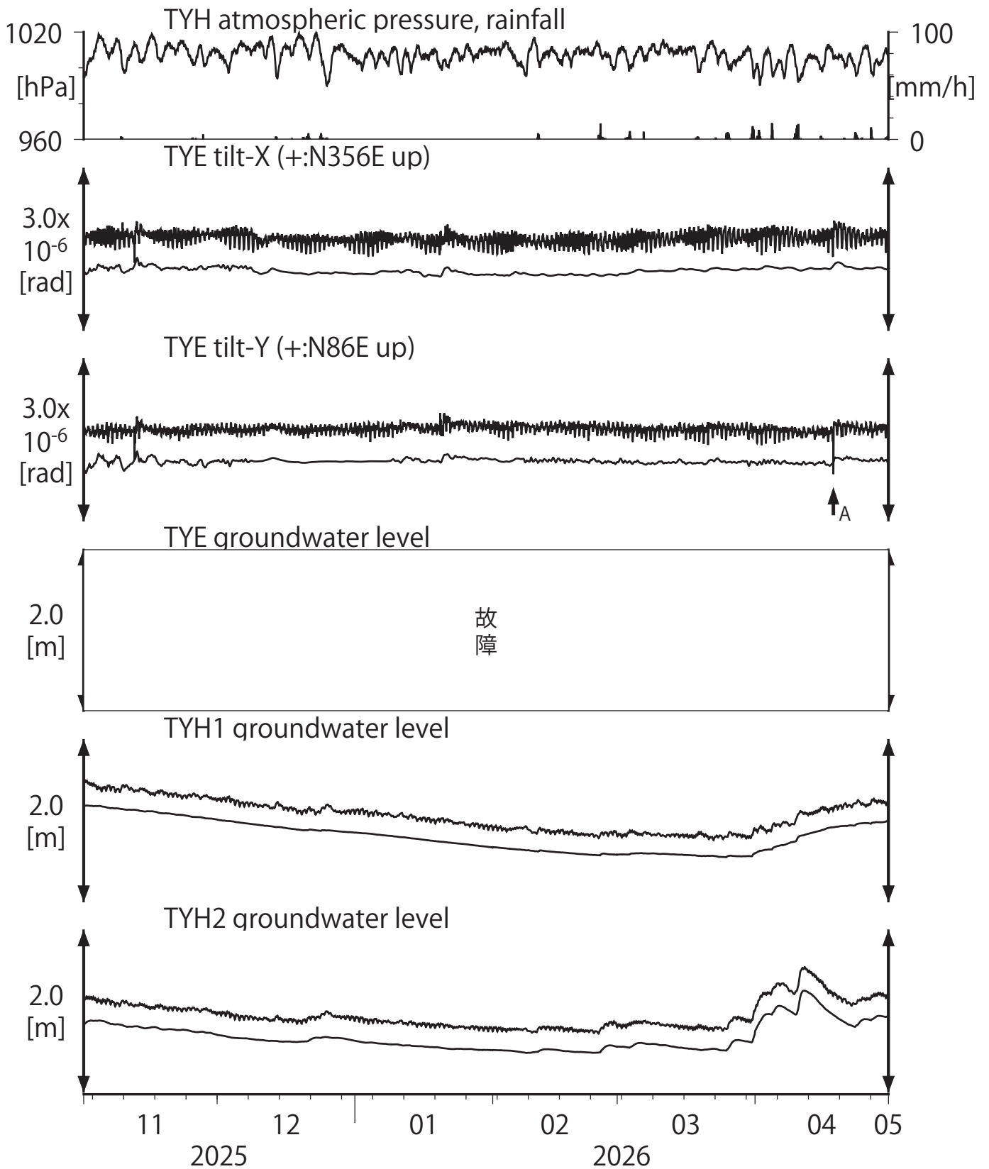
第7図 Tilt and groundwater level at TYE and TYH (時間値) (2025/11/01 00:00 - 2026/05/01 00:00 (JST))
