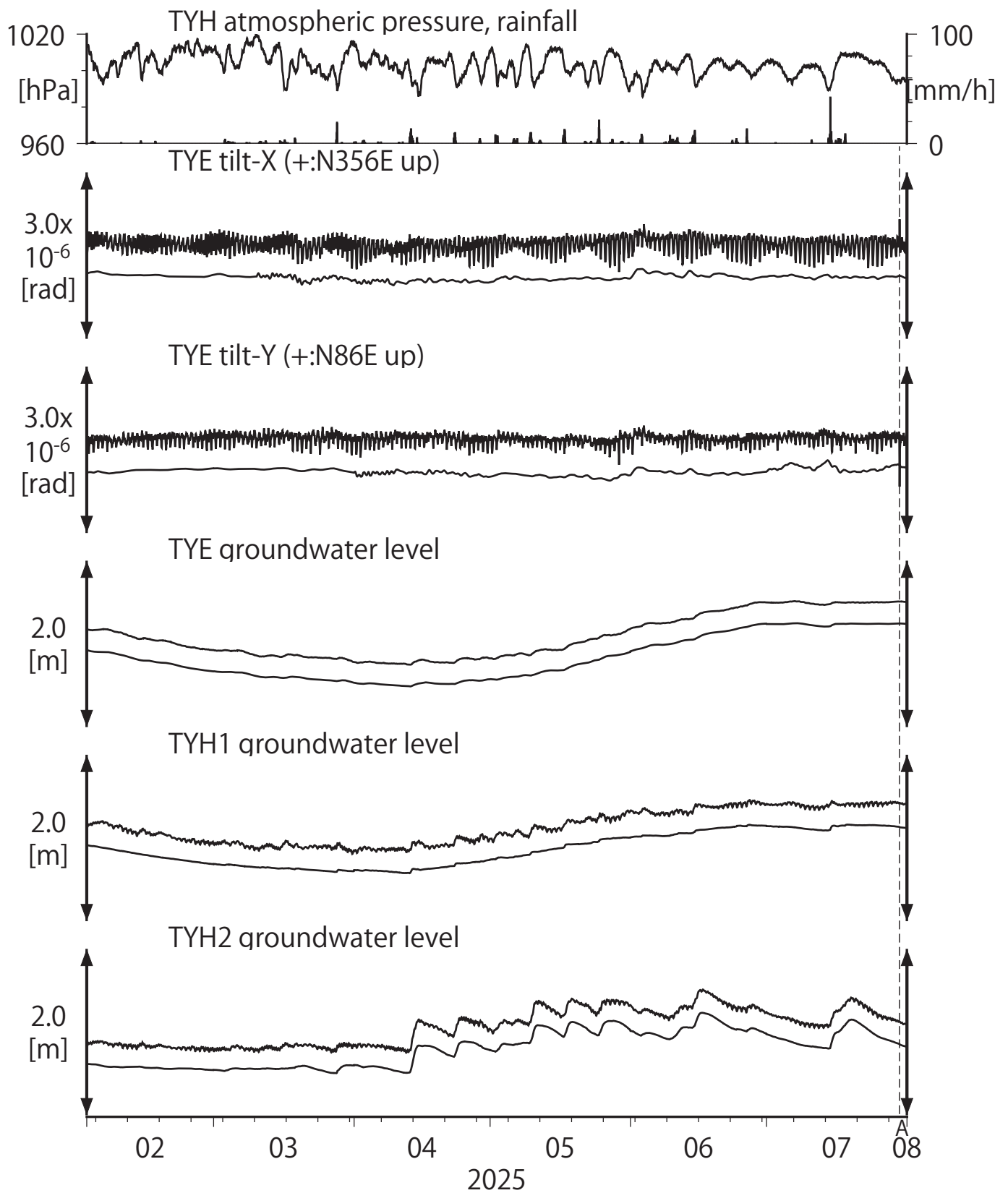
第7図 Tilt and groundwater level at TYE and TYH (時間値) (2025/02/01 00:00 - 2025/08/01 00:00 (JST))
