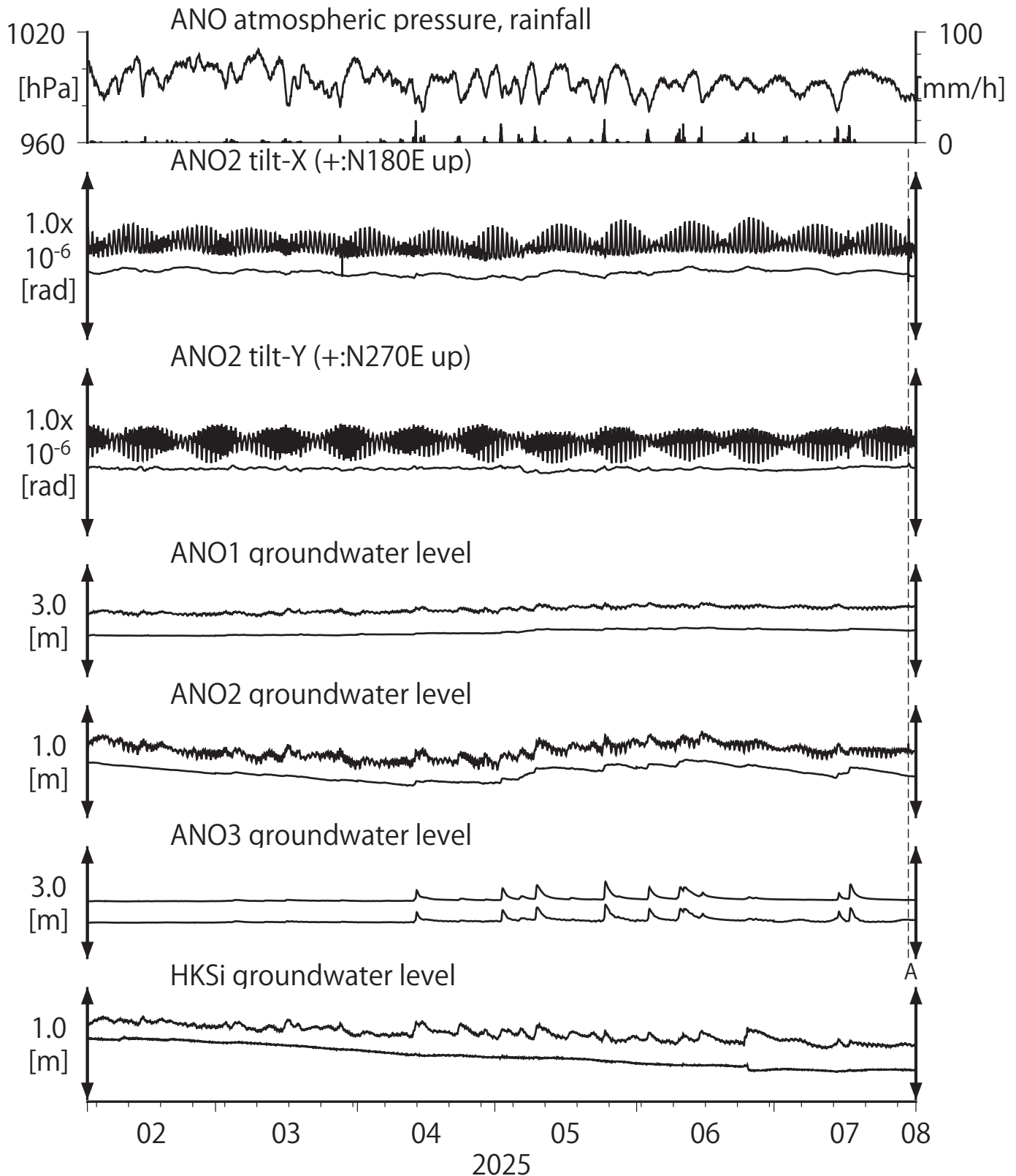
第9図 Tilt and groundwater level at ANO and HKS (時間値) (2025/02/01 00:00 - 2025/08/01 00:00 (JST))
