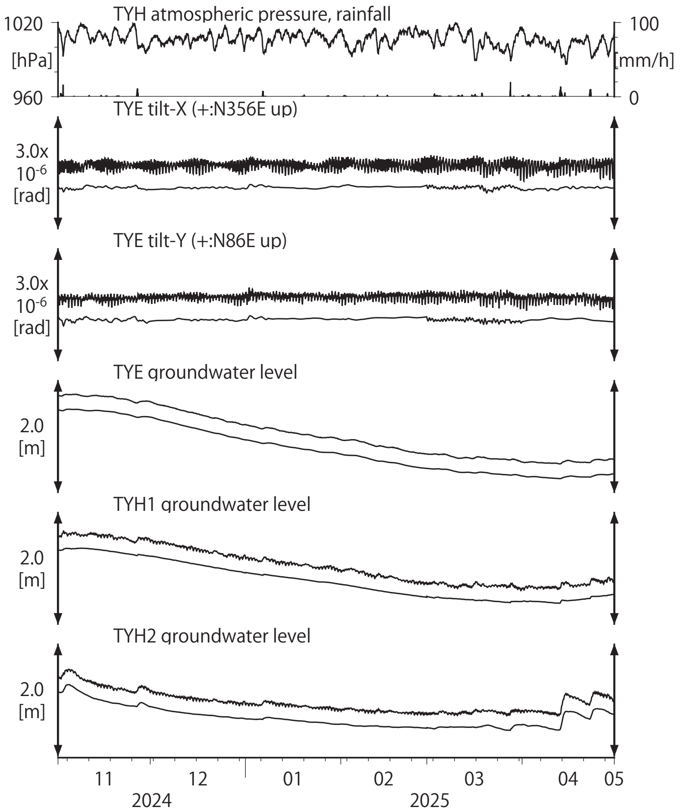
第7図 Tilt and groundwater level at TYE and TYH (時間値) (2024/11/01 00:00 - 2025/05/01 00:00 (JST))
