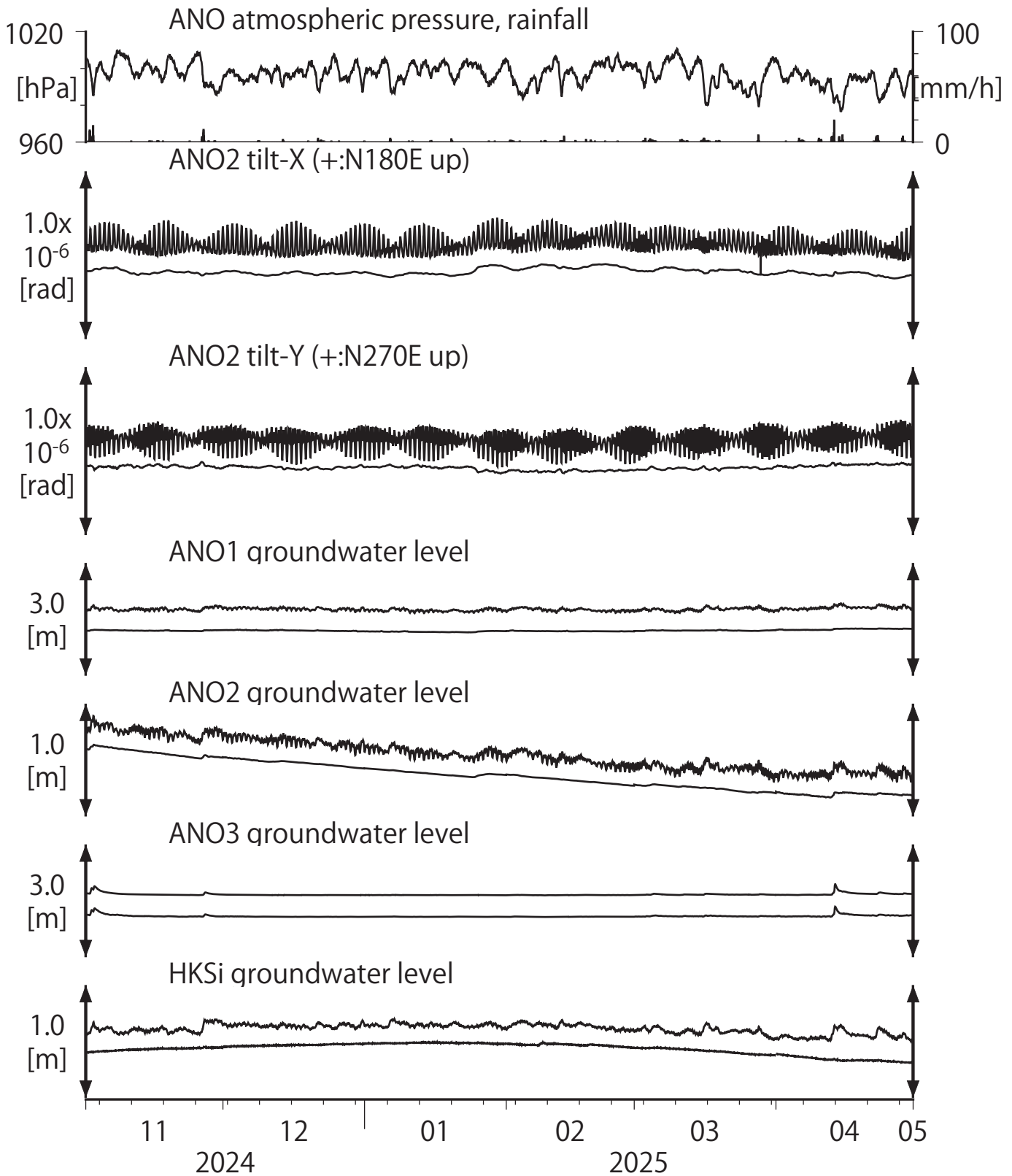
第9図 Tilt and groundwater level at ANO and HKS (時間値) (2024/11/01 00:00 - 2025/05/01 00:00 (JST))
