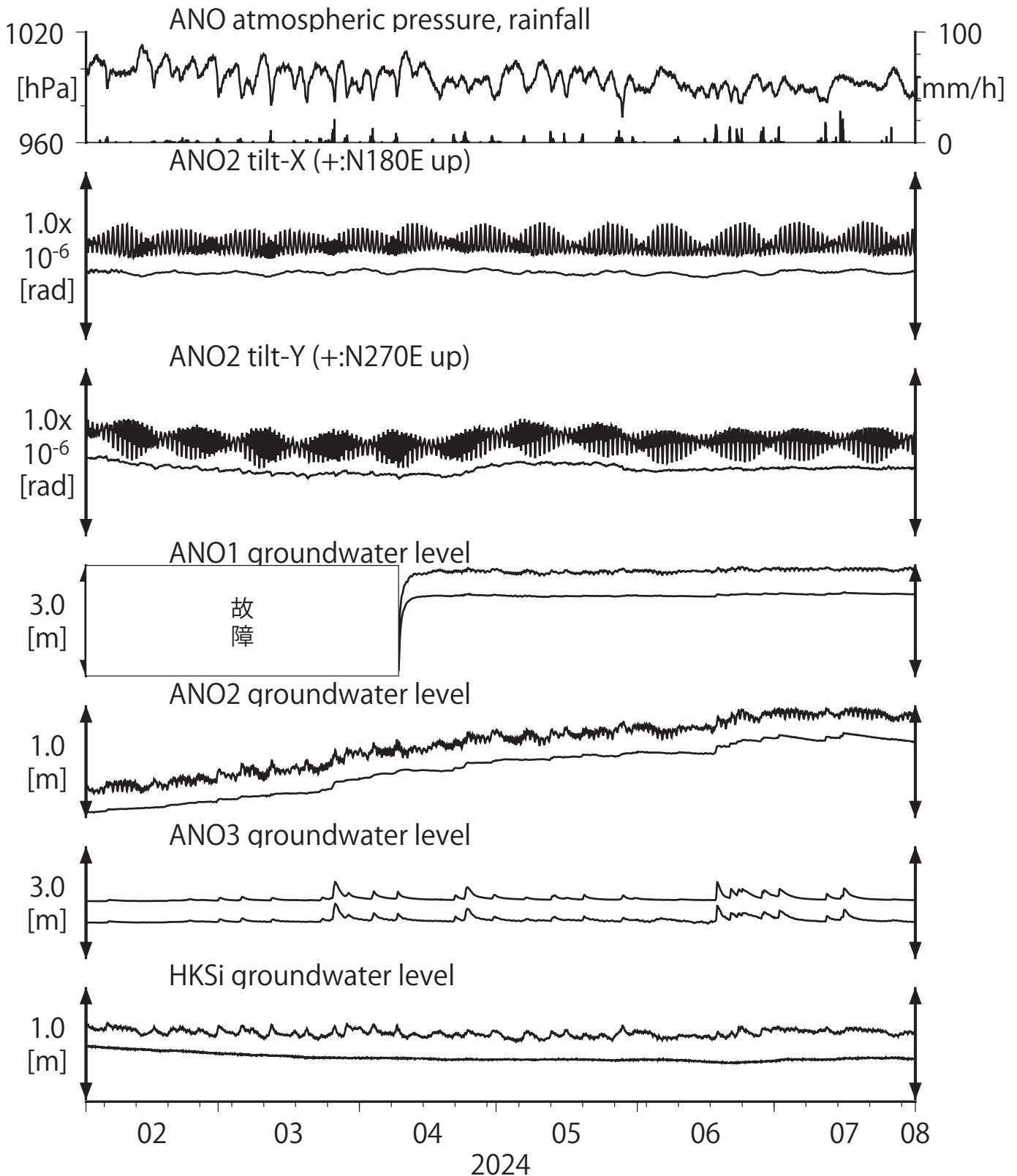
第9図 Tilt and groundwater level at ANO and HKS (時間値) (2024/02/01 00:00 - 2024/08/01 00:00 (JST))
