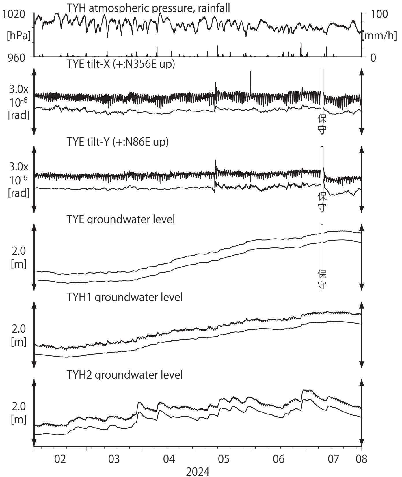
第7図 Tilt and groundwater level at TYE and TYH (時間値) (2024/02/01 00:00 - 2024/08/01 00:00 (JST))
