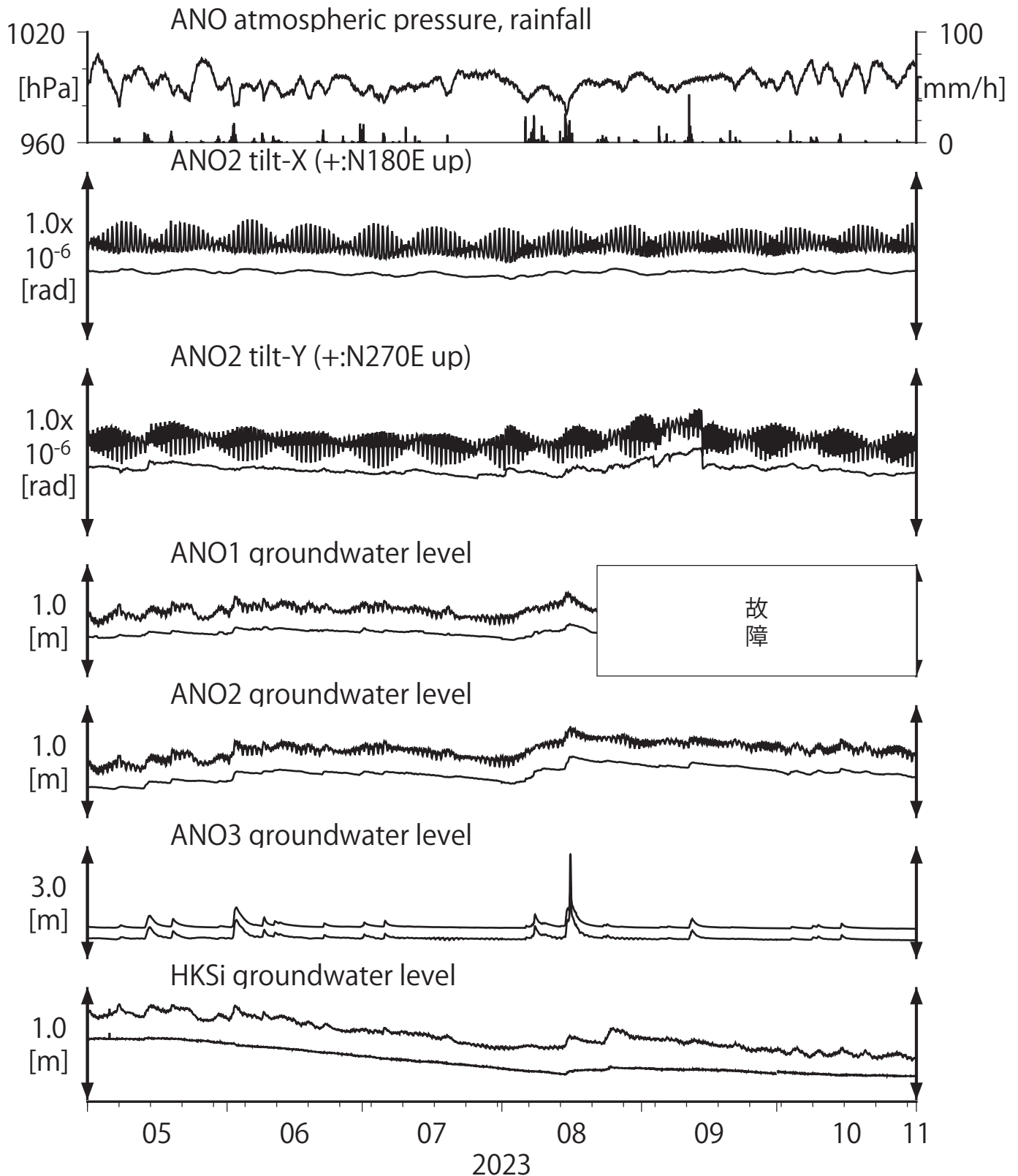
第9図 Tilt and groundwater level at ANO and HKS (時間値) (2023/05/01 00:00 - 2023/11/01 00:00 (JST))
