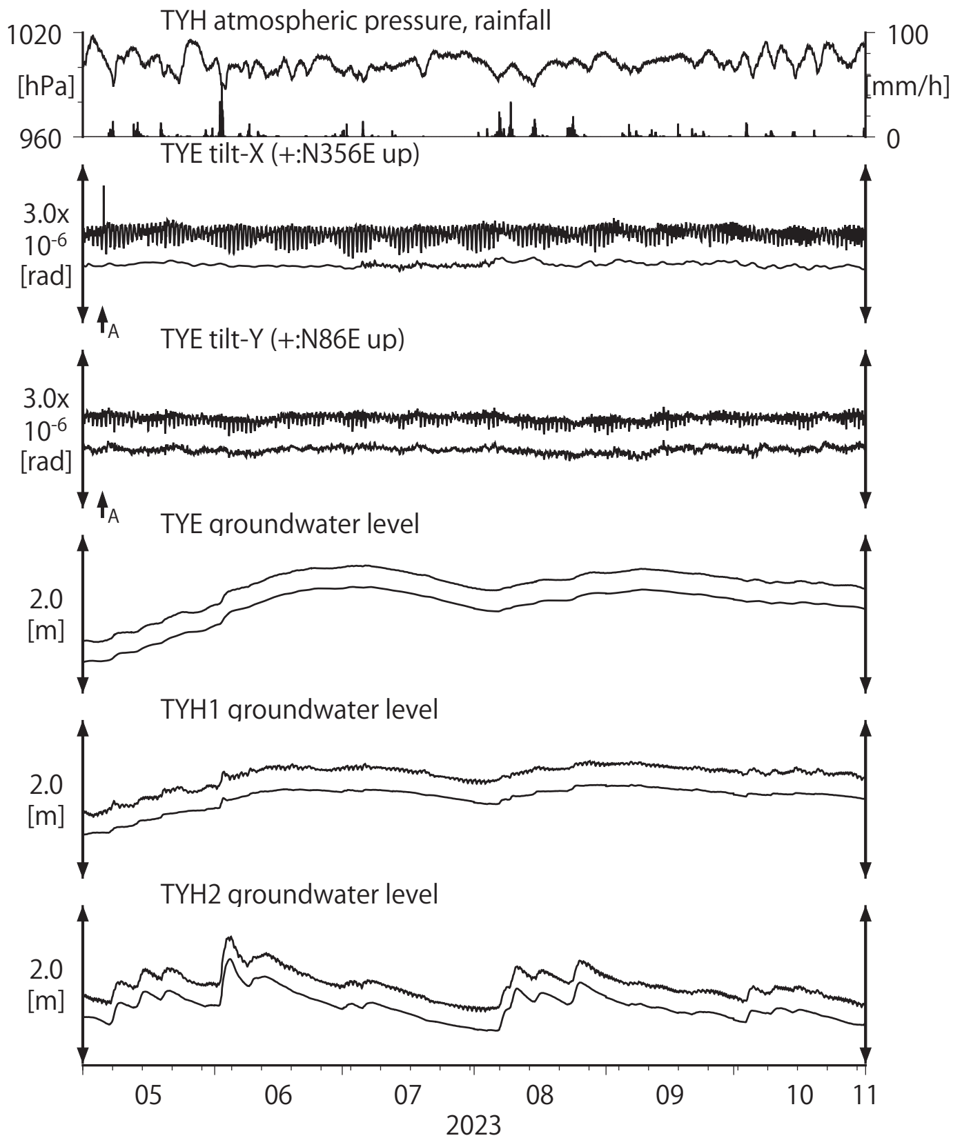
第7図 Tilt and groundwater level at TYE and TYH (時間値) (2023/05/01 00:00 - 2023/11/01 00:00 (JST))
