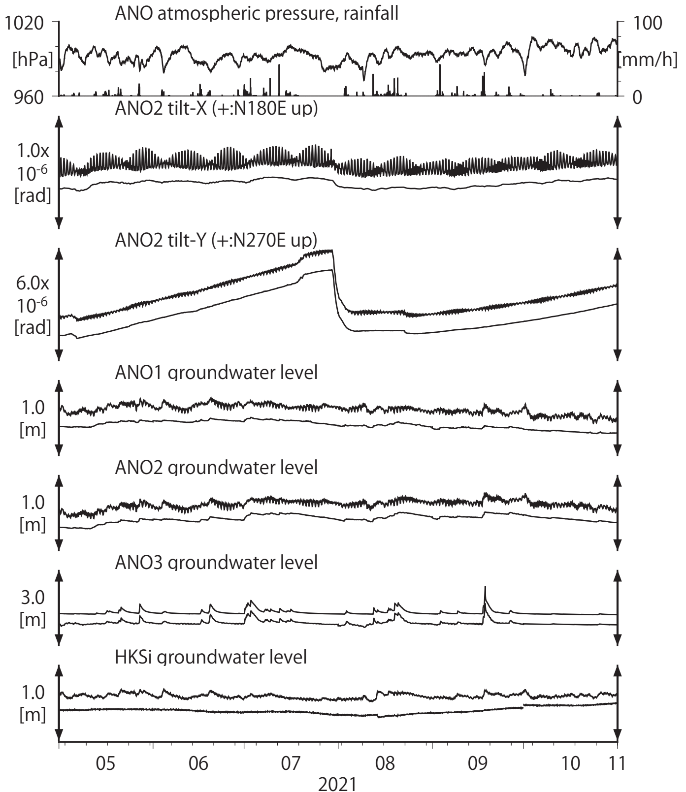
第9図 Tilt and groundwater level at ANO and HKS (時間値) (2021/05/01 00:00 - 2021/11/01 00:00 (JST))
