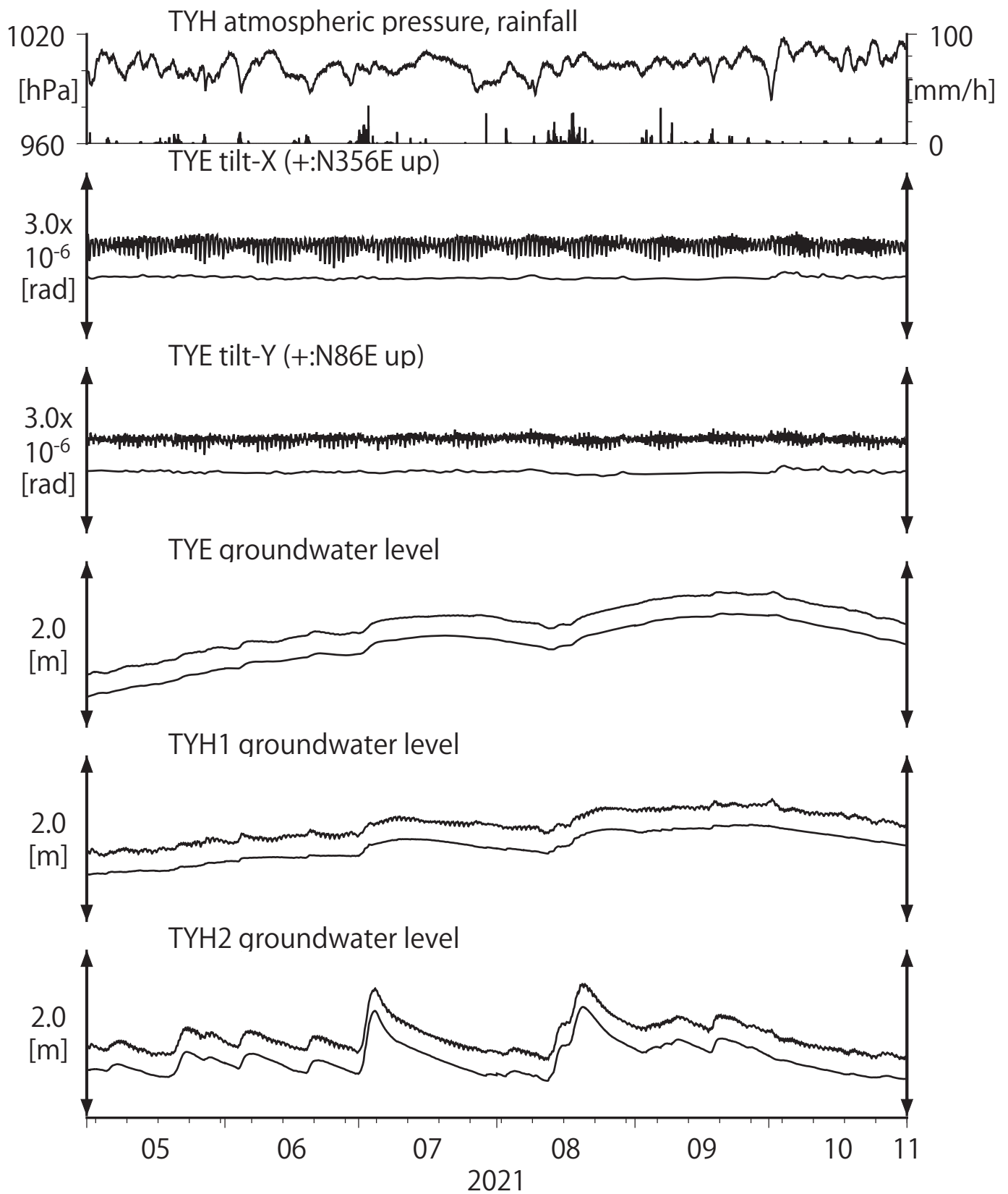
第7図 Tilt and groundwater level at TYE and TYH (時間値) (2021/05/01 00:00 - 2021/11/01 00:00 (JST))
