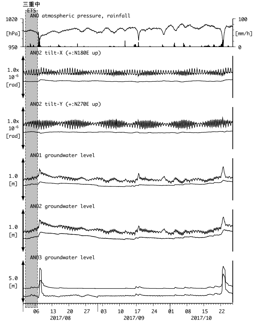
図10: Tilt and groundwater level changes at ANO 津安濃 (時間値) (2017/08/01 00:00 - 2017/10/27 00:00 (JST))
