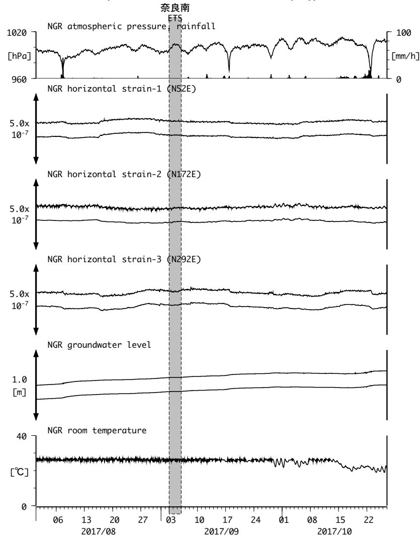
図21: Crustal strain and groundwater level changes at 岩出東坂本 (時間値) (2017/08/01 00:00 - 2017/10/27 00:00 (JST))
