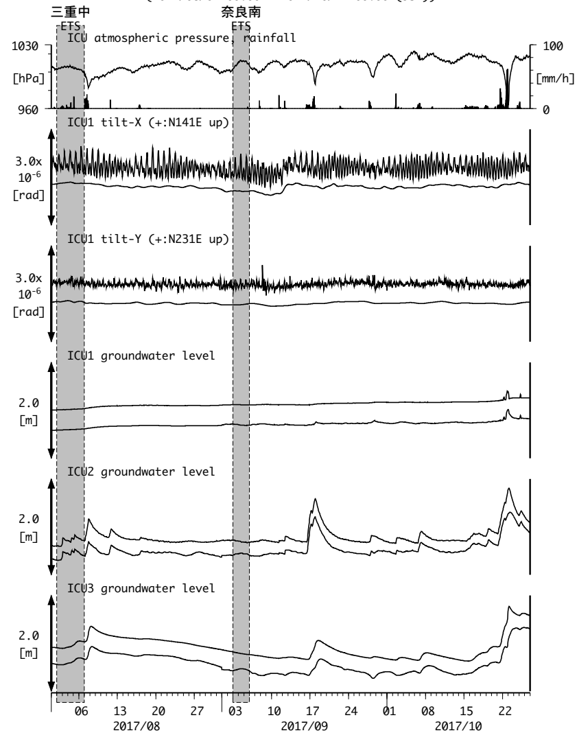
図16: Tilt and groundwater level changes at ICU 熊野磯崎 (時間値) (2017/08/01 00:00 - 2017/10/27 00:00 (JST))
