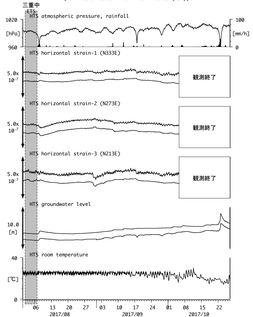
図8: Crustal strain and groundwater level changes at HTS 愛荘香之庄 (2017/08/01 00:00 - 2017/10/27 00:00 (JST))
