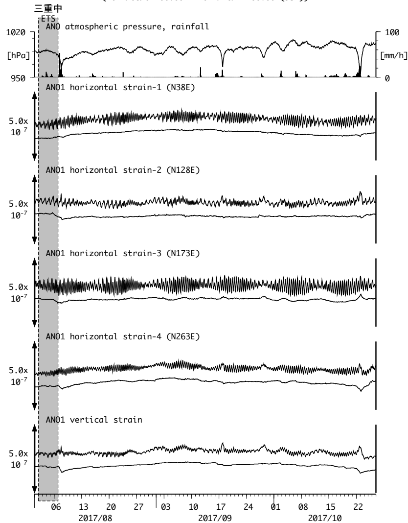
図9: Crustal strains changes at ANO 津安濃 (時間値) (2017/08/01 00:00 - 2017/10/27 00:00 (JST))
