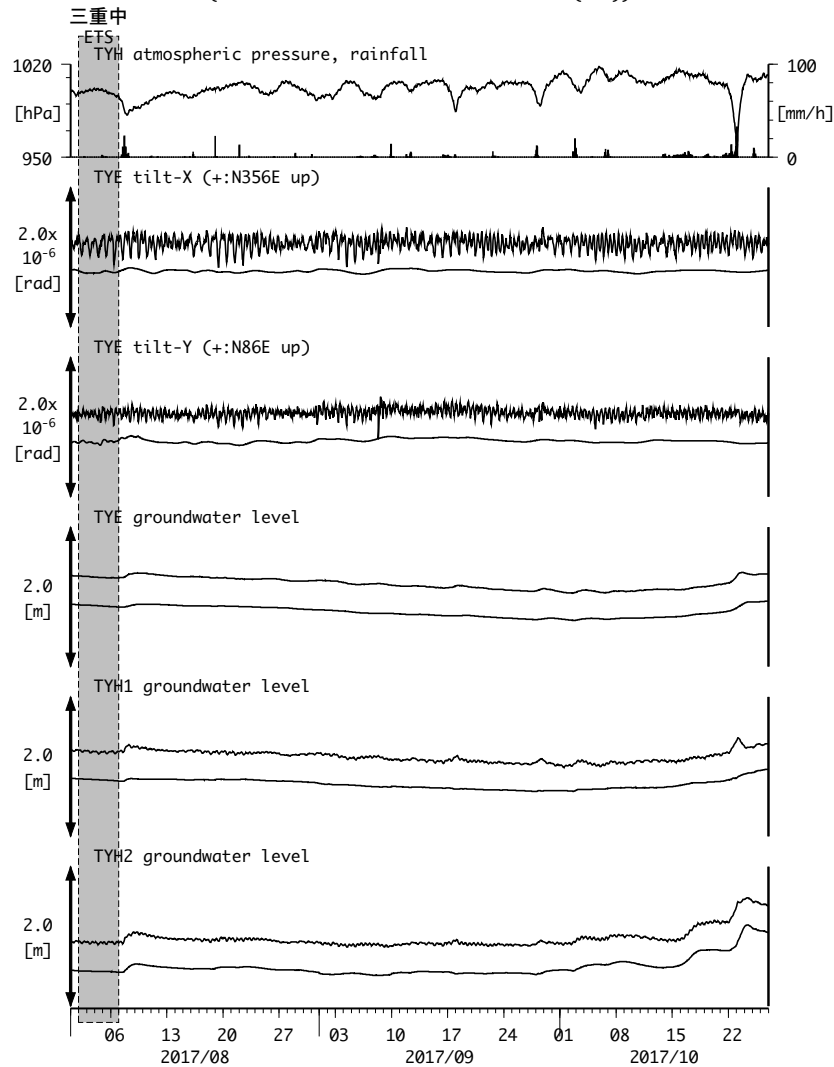
図7: Tilt and groundwater level changes at TYE and TYH 豊橋多米・豊橋 (2017/08/01 00:00 - 2017/10/27 00:00 (JST))
