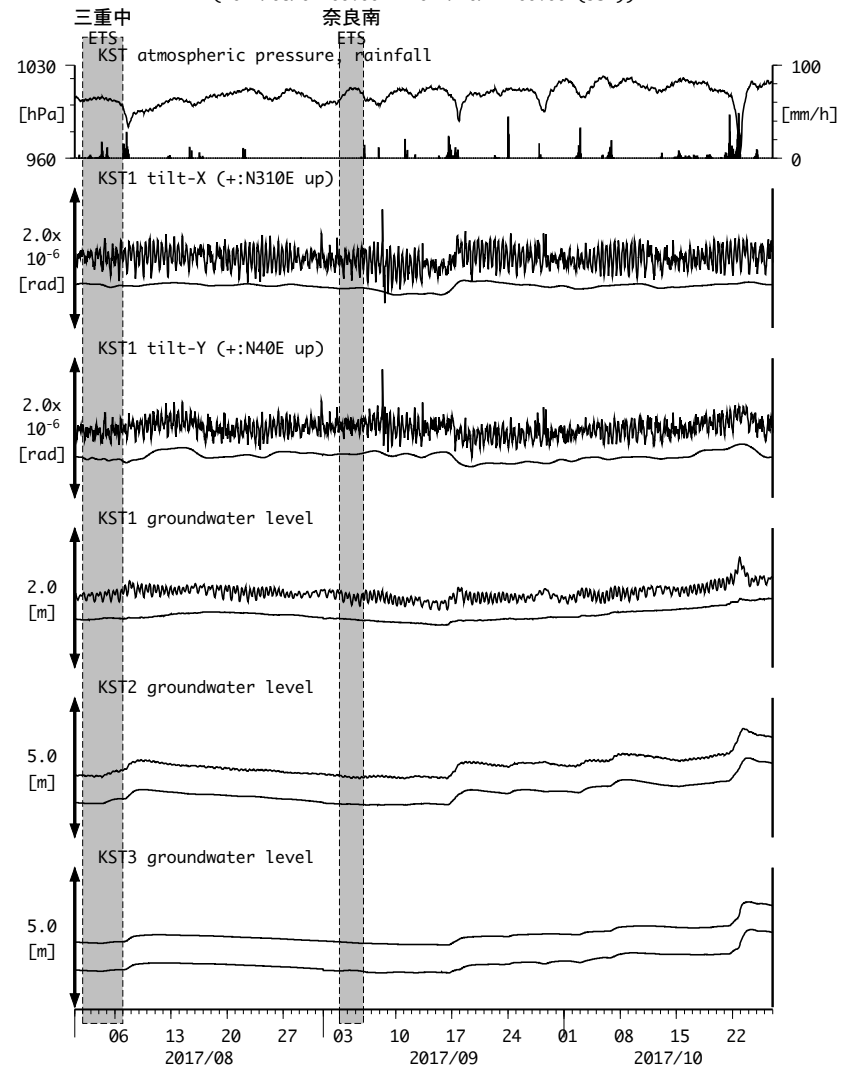
図20: Tilt and groundwater level changes at KST 串本津荷 (時間値) (2017/08/01 00:00 - 2017/10/27 00:00 (JST))
