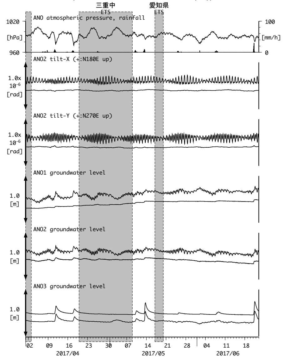
図10: Tilt and groundwater level changes at ANO 津安濃 (時間値) (2017/04/01 00:00 - 2017/06/23 00:00 (JST))
