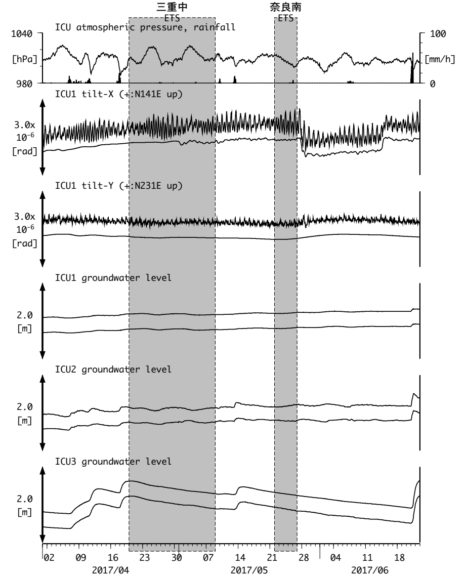
図16: Tilt and groundwater level changes at ICU 熊野磯崎 (時間値) (2017/04/01 00:00 - 2017/06/23 00:00 (JST))
