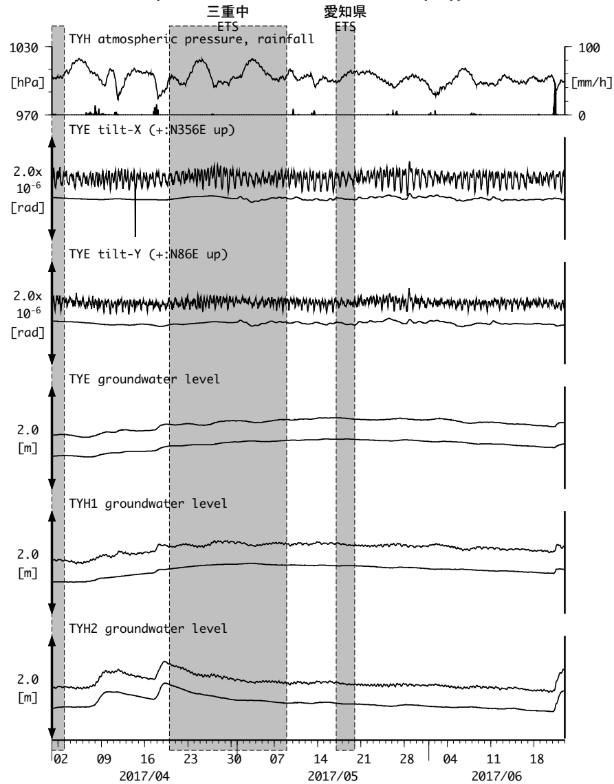
図7: Tilt and groundwater level changes at TYE and TYH 豊橋多米・豊橋 (2017/04/01 00:00 - 2017/06/23 00:00 (JST))
