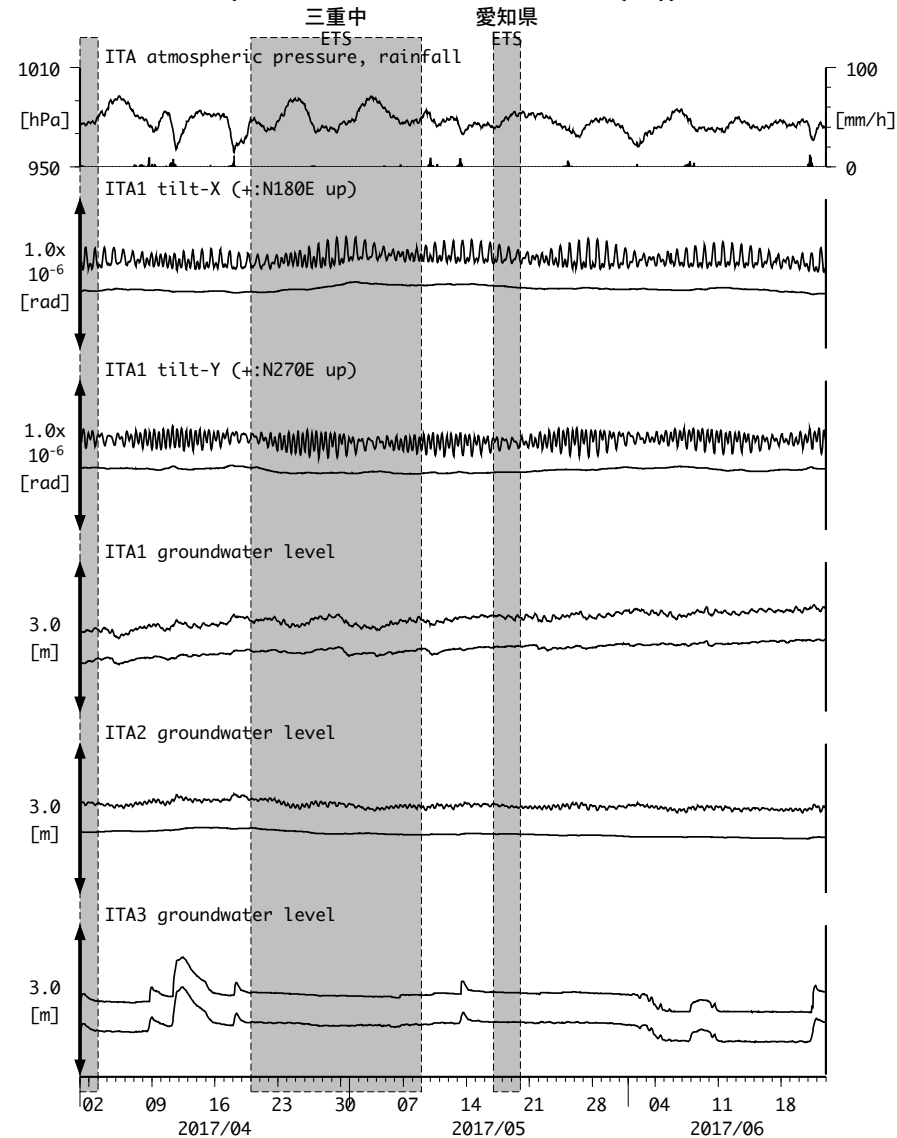
図12: Tilt and groundwater level changes at ITA 松阪飯高 (時間値) (2017/04/01 00:00 - 2017/06/23 00:00 (JST))
