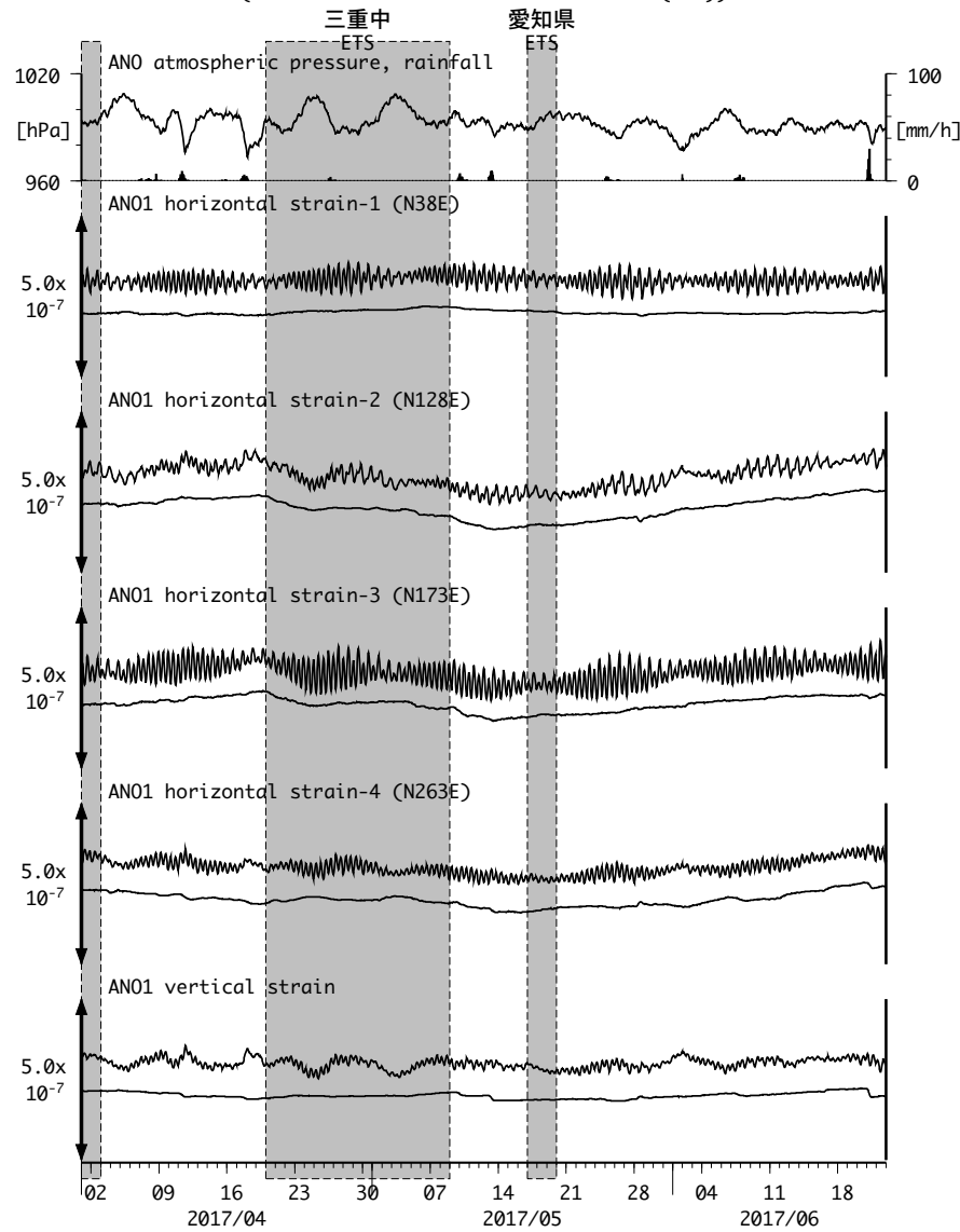
図9: Crustal strains changes at ANO 津安濃 (時間値) (2017/04/01 00:00 - 2017/06/23 00:00 (JST))
