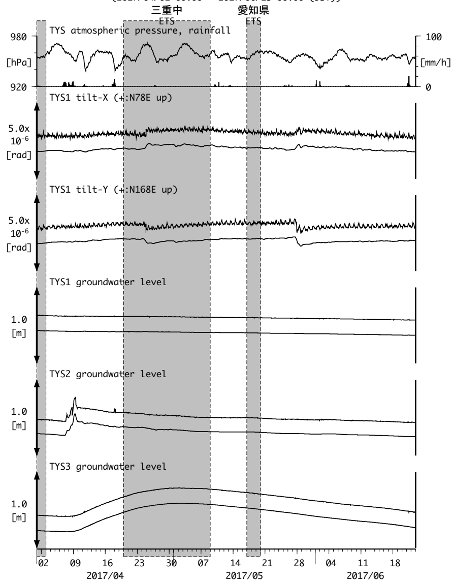
図3: Tilt and groundwater level changes at TYS 豊田神殿 (時間値) (2017/04/01 00:00 - 2017/06/23 00:00 (JST))
