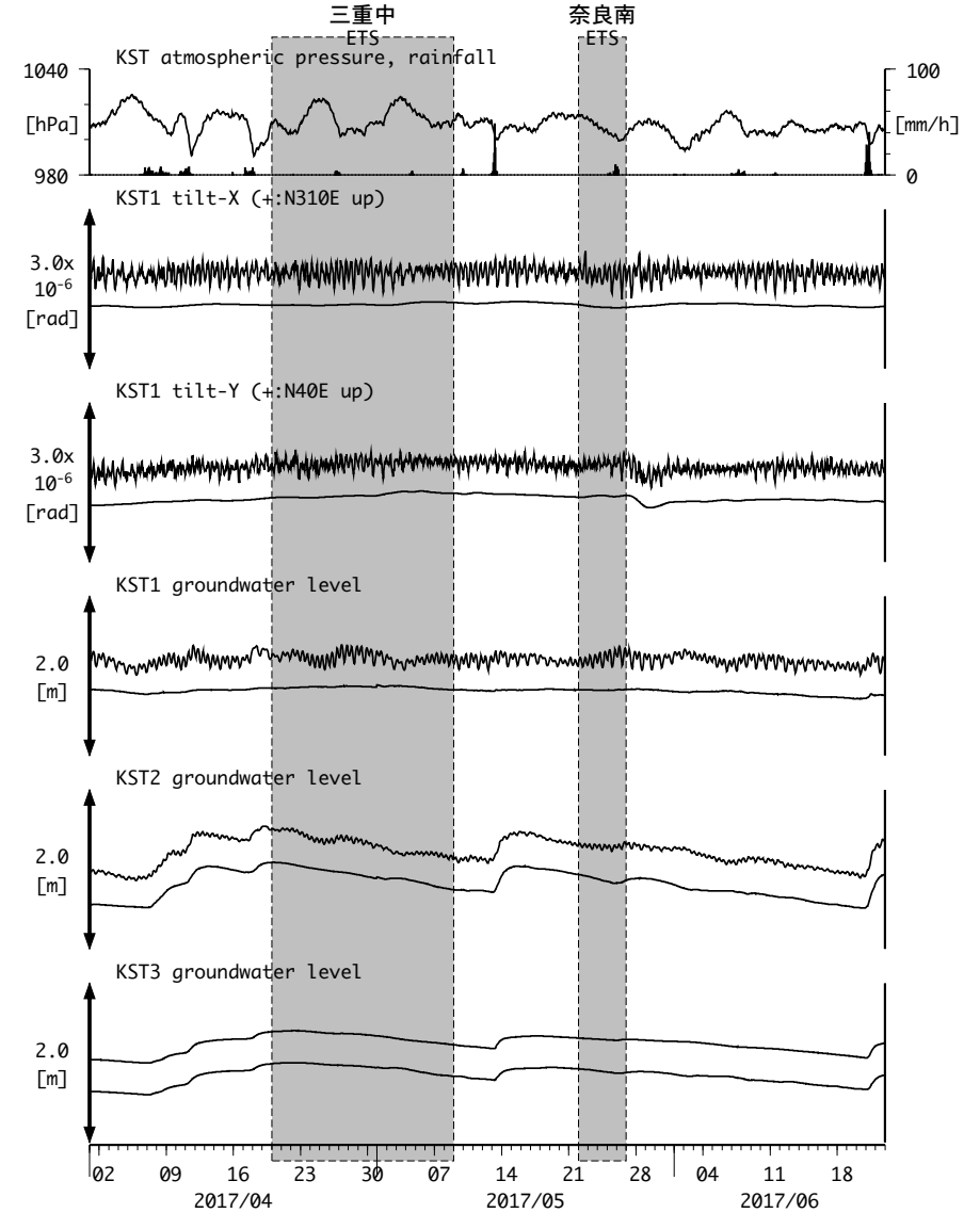
図20: Tilt and groundwater level changes at KST 串本津荷 (時間値) (2017/04/01 00:00 - 2017/06/23 00:00 (JST))
