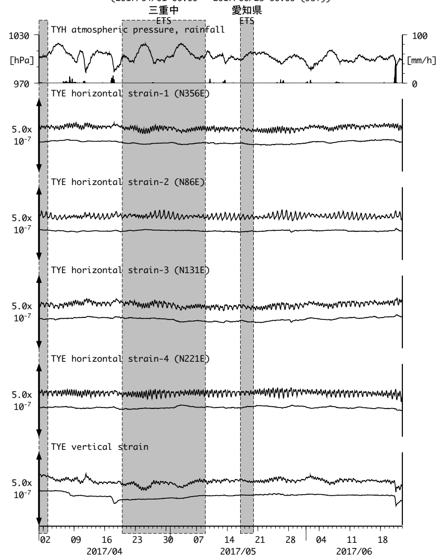
図6: Crustal strain changes at TYE 豊橋多米 (時間値) (2017/04/01 00:00 - 2017/06/23 00:00 (JST))
