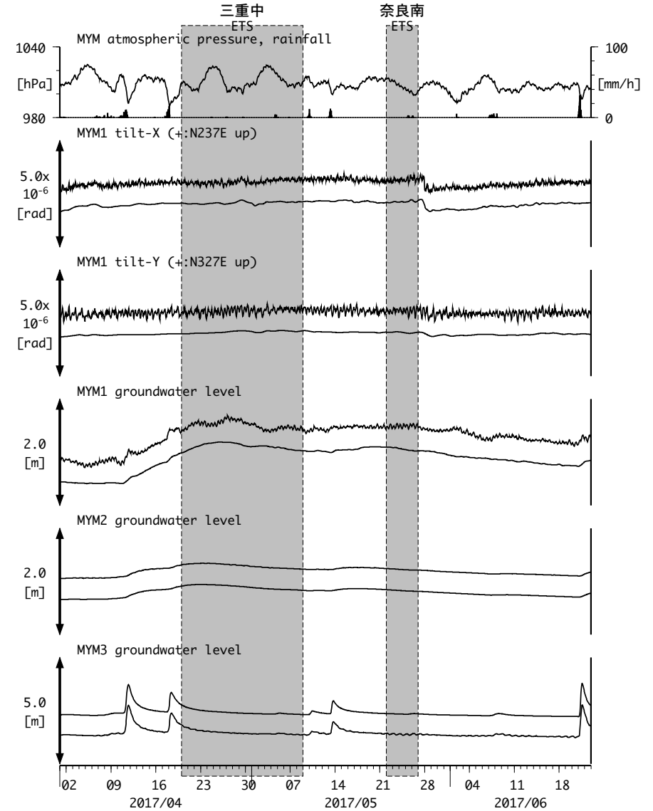
図14: Tilt and groundwater level changes at MYM 紀北海山 (時間値) (2017/04/01 00:00 - 2017/06/23 00:00 (JST))
