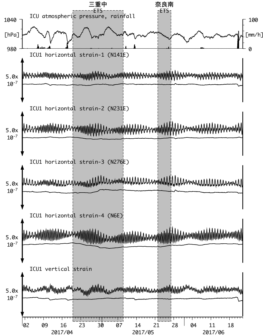
図15: Crustal strain changes at ICU 熊野磯崎 (時間値) (2017/04/01 00:00 - 2017/06/23 00:00 (JST))
