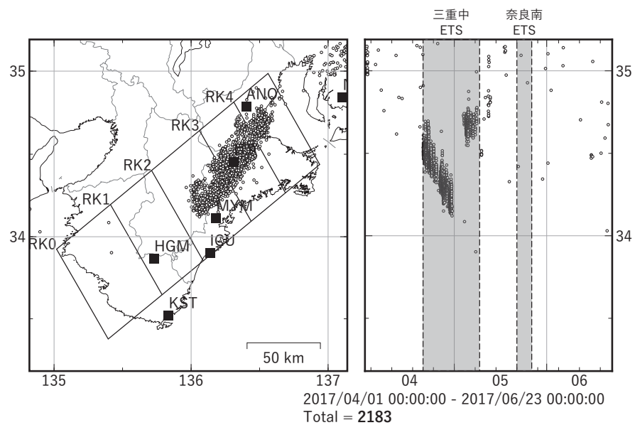
Deep low-frequency tremor activities in Kii Peninsula (日値) (2017/04/01 00:00 - 2017/06/23 00:00 (JST))
