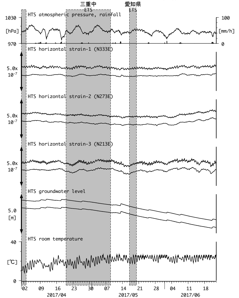
図8: Crustal strain and groundwater level changes at HTS 愛荘香之庄 (2017/04/01 00:00 - 2017/06/23 00:00 (JST))
