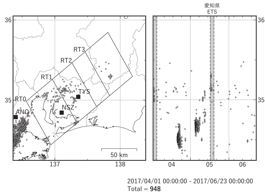
Deep low-frequency tremors in Tokai (日値) (2017/04/01 00:00 - 2017/06/23 00:00 (JST))
