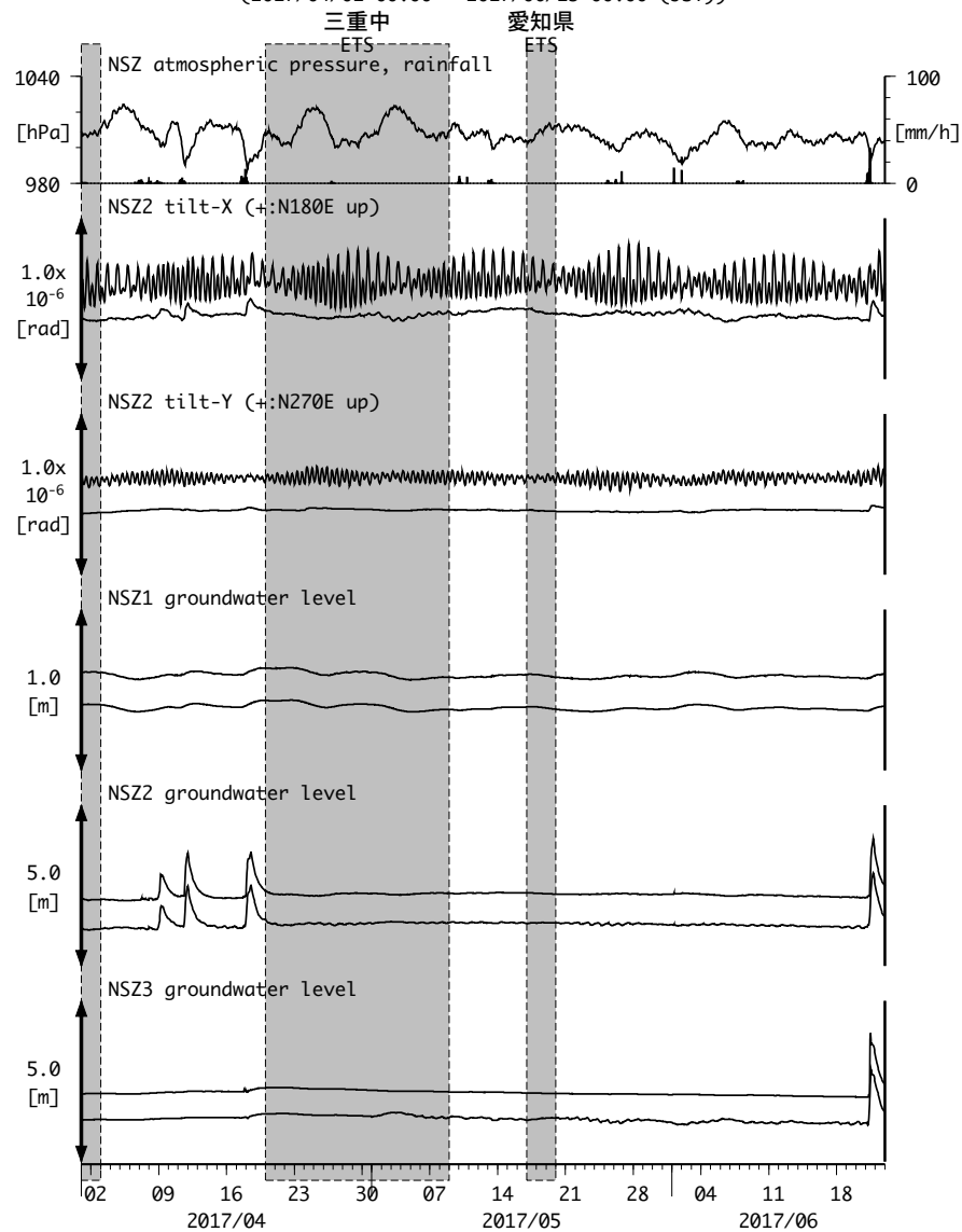
図5: Tilt and groundwater level changes at NSZ 西尾善明 (時間値) (2017/04/01 00:00 - 2017/06/23 00:00 (JST))
