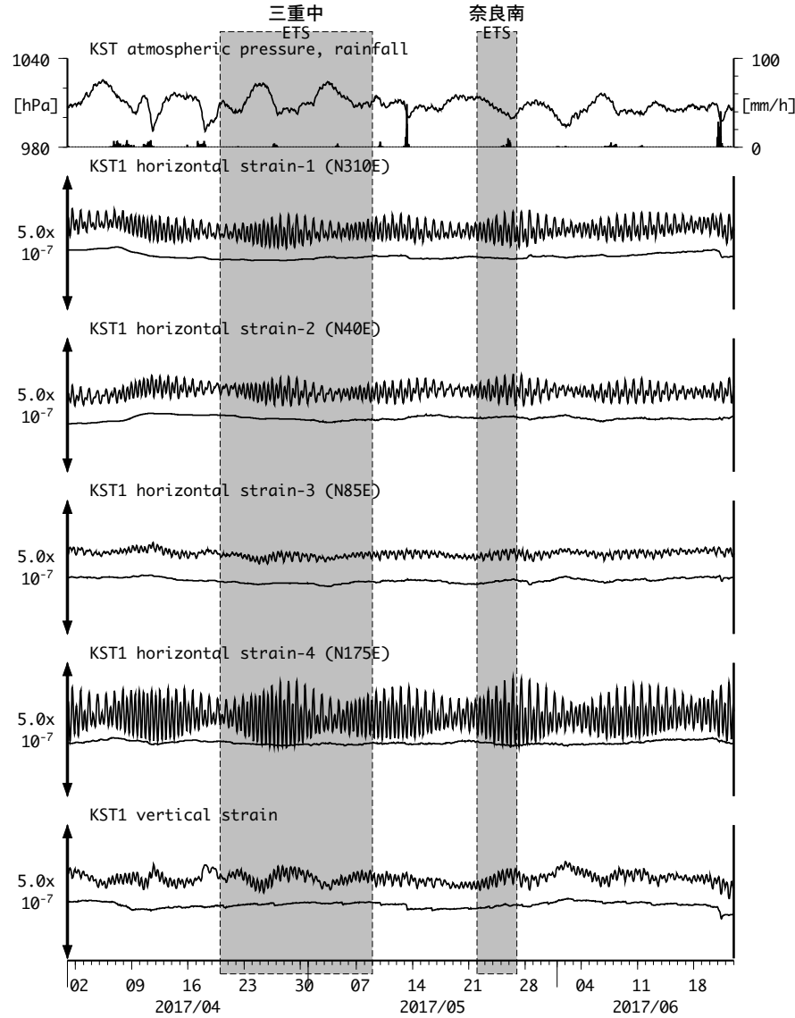
図19: Crustal strain changes at KST 串本津荷 (時間値) (2017/04/01 00:00 - 2017/06/23 00:00 (JST))
