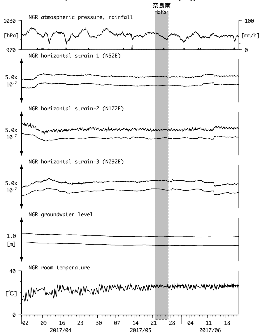
図21: Crustal strain and groundwater level changes at 岩出東坂本 (時間値) (2017/04/01 00:00 - 2017/06/23 00:00 (JST))
