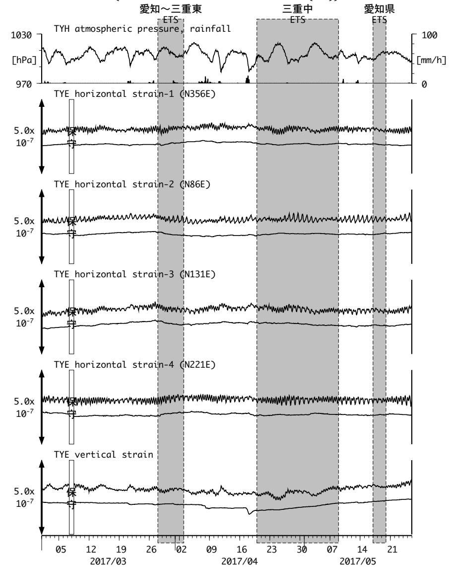
図6: Crustal strain changes at TYE 豊橋多米 (時間値) (2017/03/01 00:00 - 2017/05/26 00:00 (JST))
