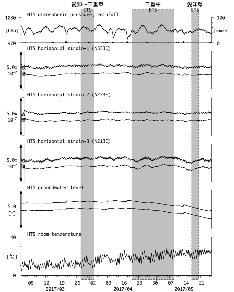
図8: Crustal strain and groundwater level changes at HTS 愛荘香之庄 (2017/03/01 00:00 - 2017/05/26 00:00 (JST))
