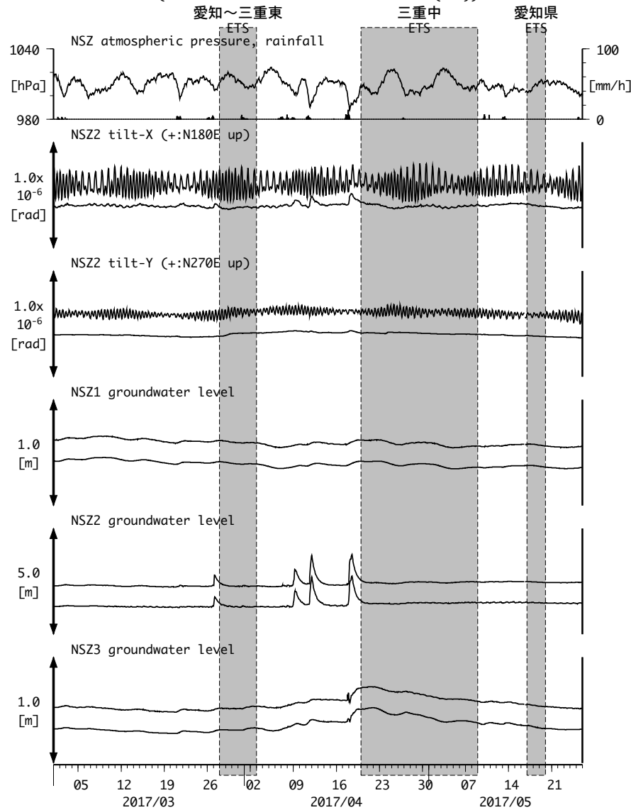
図5: Tilt and groundwater level changes at NSZ 西尾善明 (時間値) (2017/03/01 00:00 - 2017/05/26 00:00 (JST))
