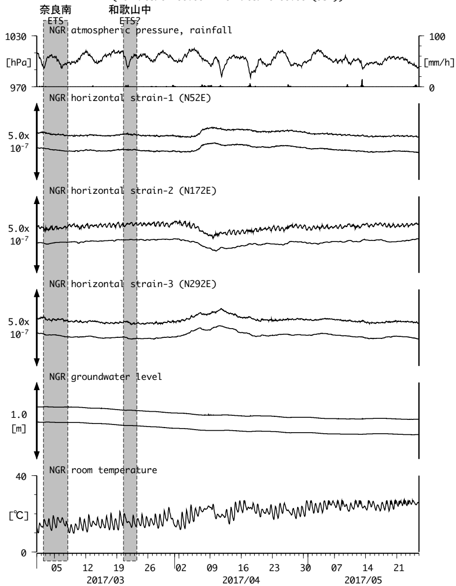
図21: Crustal strain and groundwater level changes at 岩出東坂本 (時間値) (2017/03/01 00:00 - 2017/05/26 00:00 (JST))
