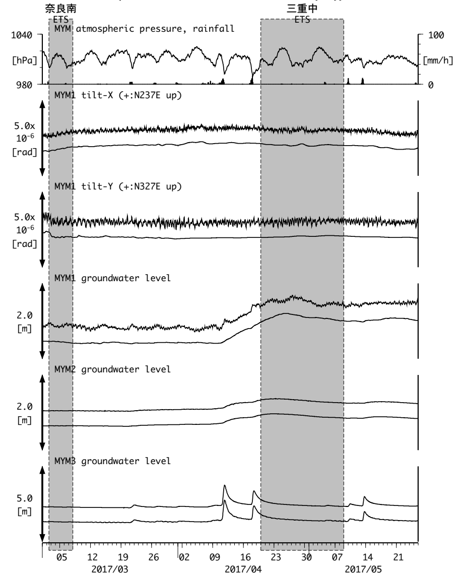
図14: Tilt and groundwater level changes at MYM 紀北海山 (時間値) (2017/03/01 00:00 - 2017/05/26 00:00 (JST))
