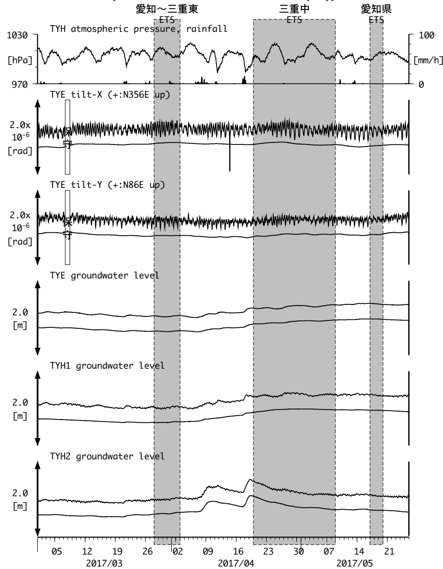
図7: Tilt and groundwater level changes at TYE and TYH 豊橋多米・豊橋 (2017/03/01 00:00 - 2017/05/26 00:00 (JST))
