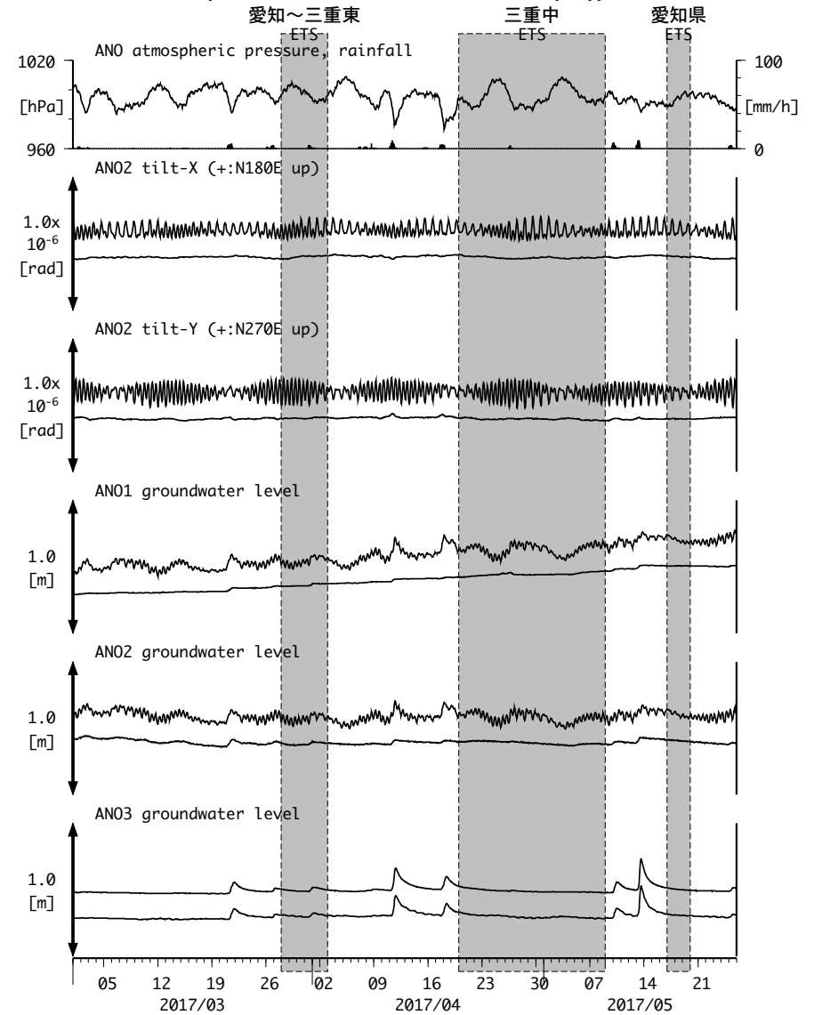
図10: Tilt and groundwater level changes at ANO 津安濃 (時間値) (2017/03/01 00:00 - 2017/05/26 00:00 (JST))
