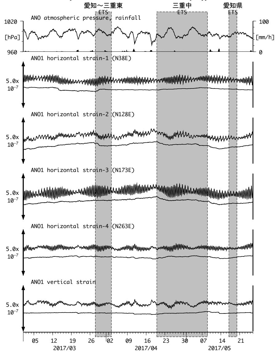
図9: Crustal strains changes at ANO 津安濃 (時間値) (2017/03/01 00:00 - 2017/05/26 00:00 (JST))
