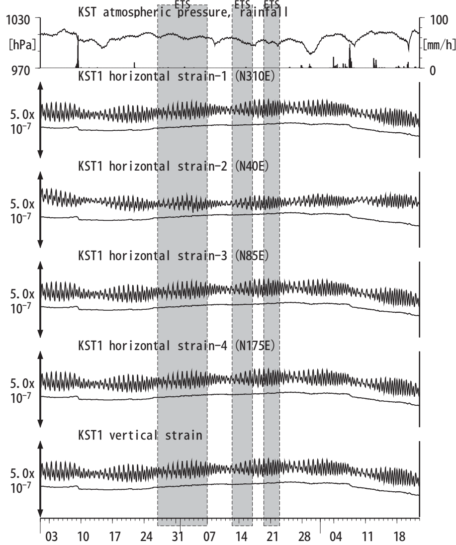
図19: Crustal strain changes at KST 串本津荷 (時間値) (2016/07/01 00:00 - 2016/09/23 00:00 (JST))
