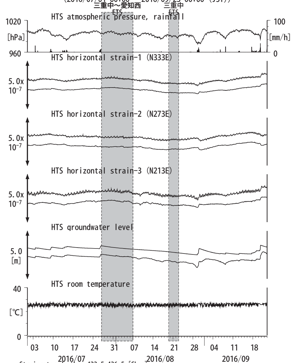
図8: Crustal strain and groundwater level changes at HTS 愛荘香之庄 (2016/07/01 00:00 - 2016/09/23 00:00 (JST))
