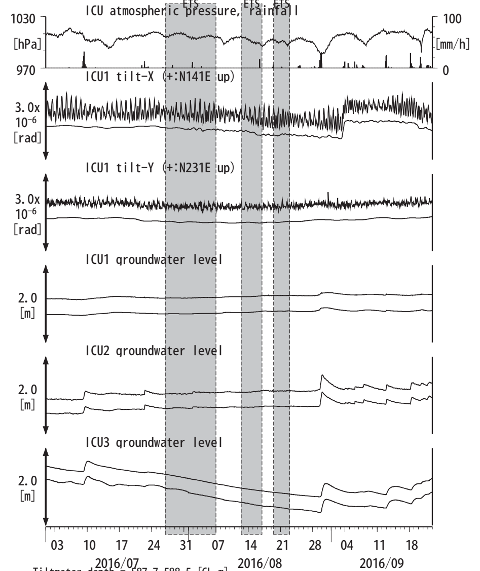
図16: Tilt and groundwater level changes at ICU 熊野磯崎 (時間値) (2016/07/01 00:00 - 2016/09/23 00:00 (JST))
