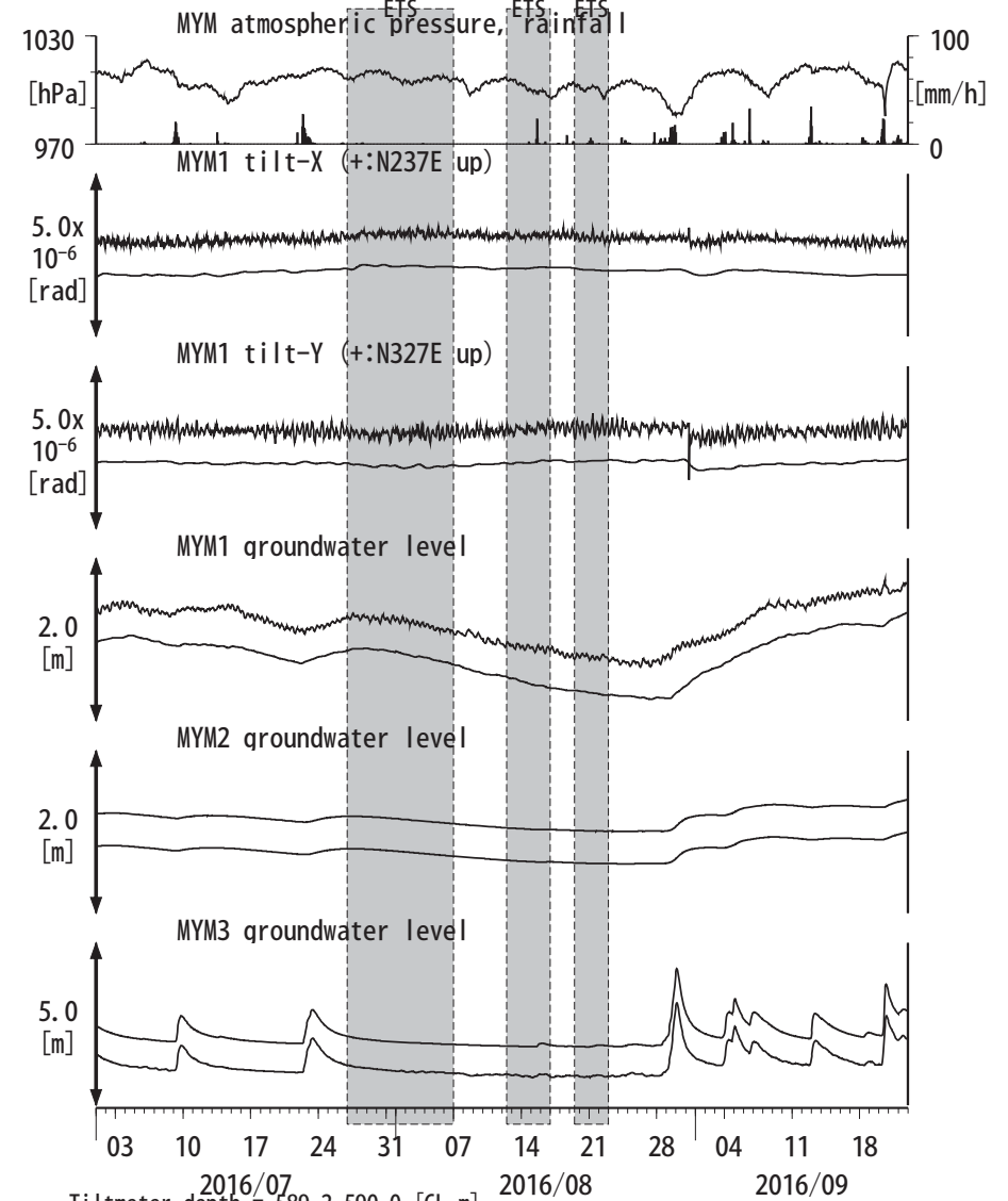
図14: Tilt and groundwater level changes at MYM 紀北海山 (時間値) (2016/07/01 00:00 - 2016/09/23 00:00 (JST))
