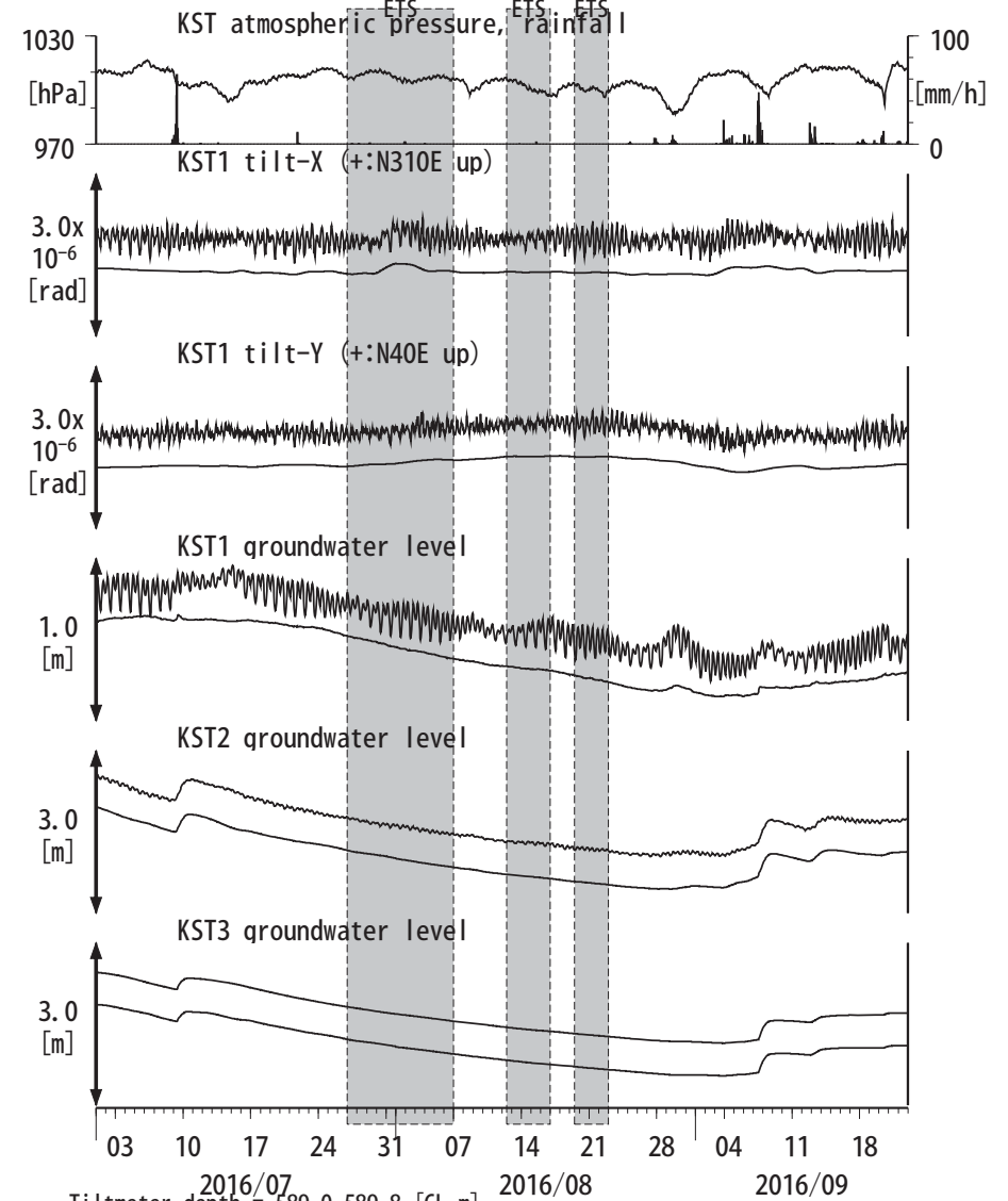
図20: Tilt and groundwater level changes at KST 串本津荷 (時間値) (2016/07/01 00:00 - 2016/09/23 00:00 (JST))
