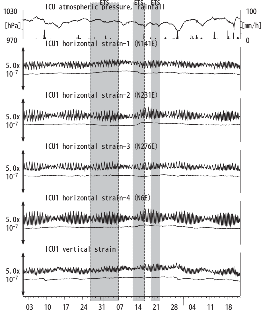
図15: Crustal strain changes at ICU 熊野磯崎 (時間値) (2016/07/01 00:00 - 2016/09/23 00:00 (JST))
