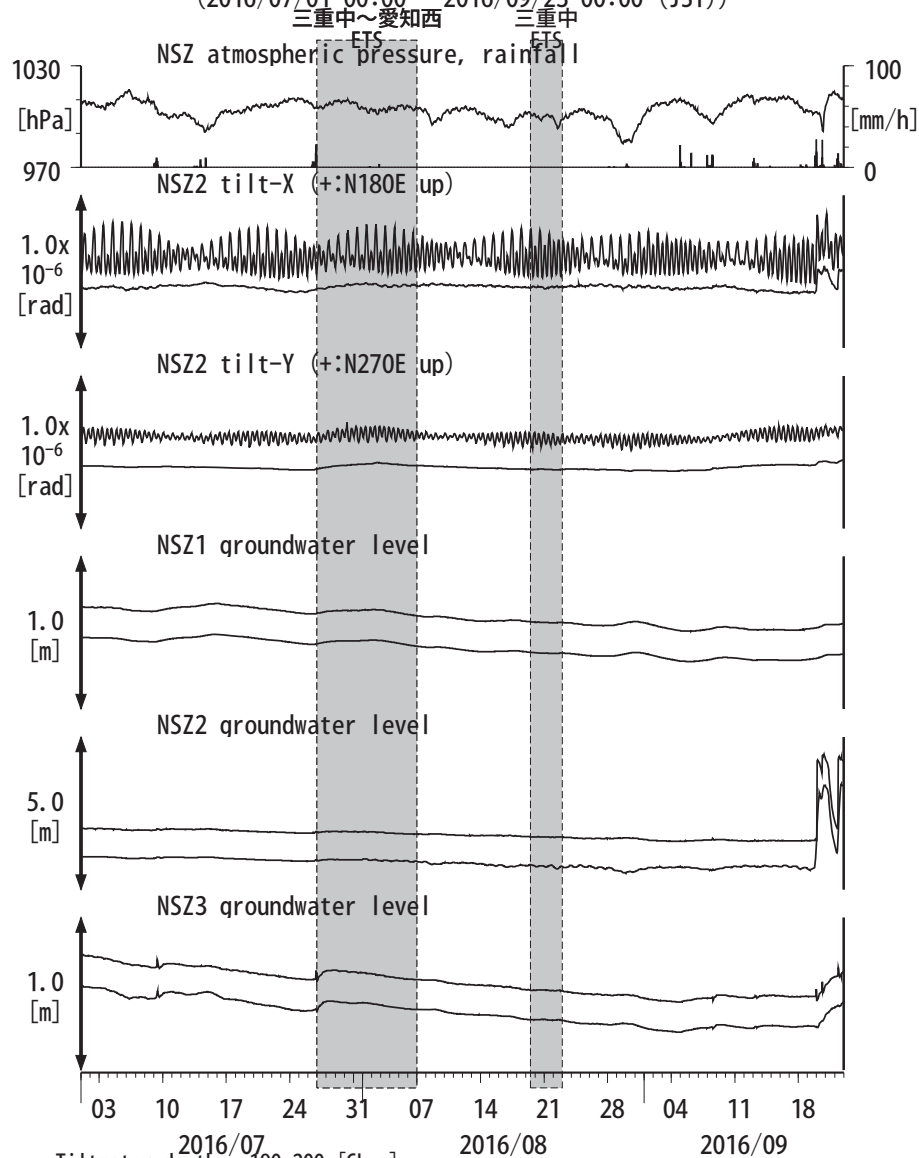
図5: Tilt and groundwater level changes at NSZ 西尾善明 (時間値) (2016/07/01 00:00 - 2016/09/23 00:00 (JST))
