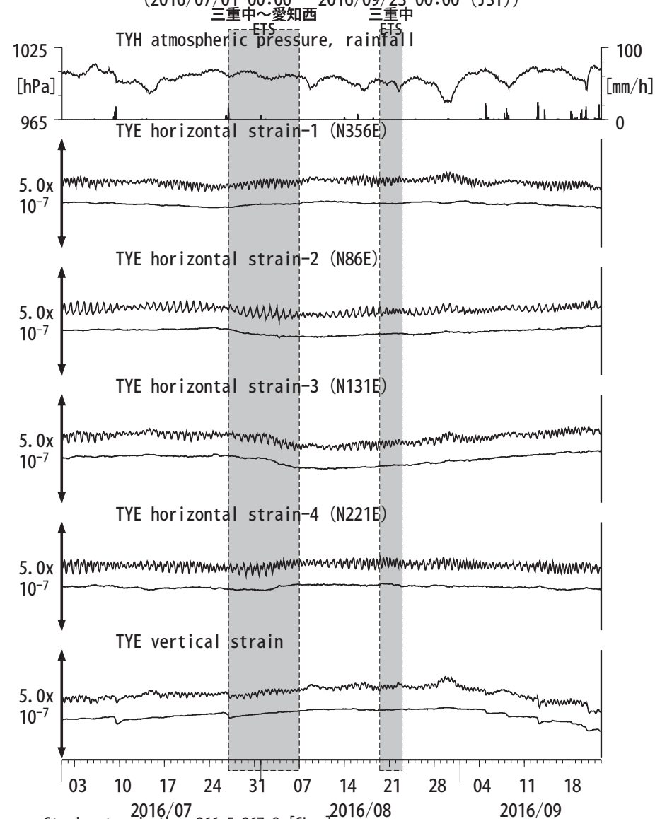
図6: Crustal strain changes at TYE 豊橋多米 (時間値) (2016/07/01 00:00 - 2016/09/23 00:00 (JST))
