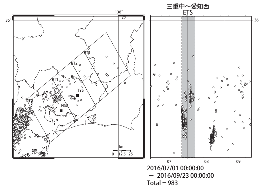
Deep low-frequency tremors in Tokai (日値) (2016/07/01 00:00 - 2016/09/23 00:00 (JST))
