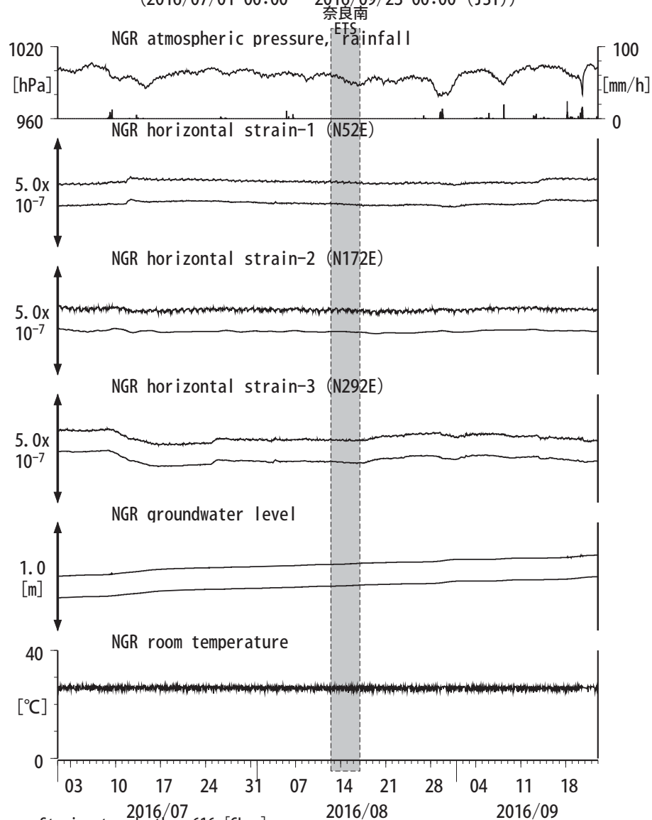
図21: Crustal strain and groundwater level changes at 岩出東坂本 (時間値) (2016/07/01 00:00 - 2016/09/23 00:00 (JST))
