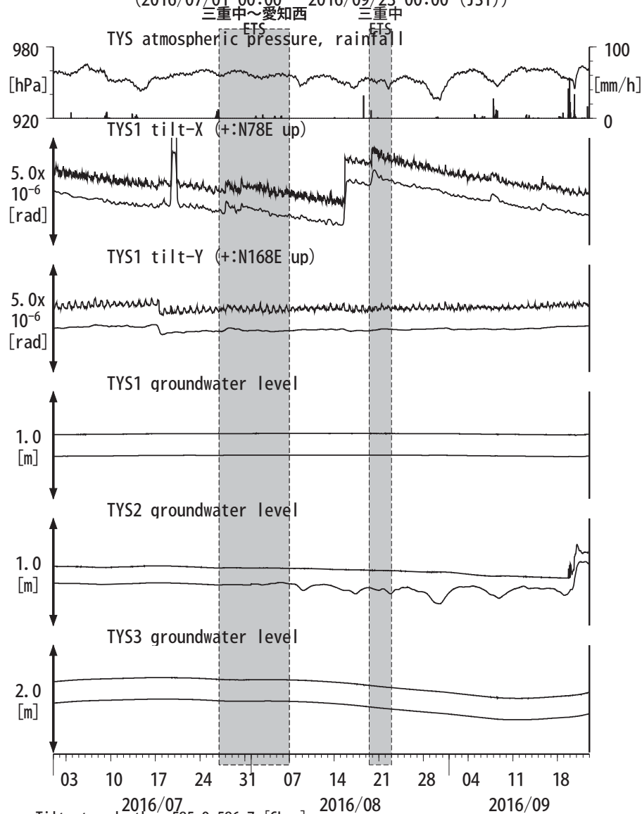
図3: Tilt and groundwater level changes at TYS 豊田神殿 (時間値) (2016/07/01 00:00 - 2016/09/23 00:00 (JST))
