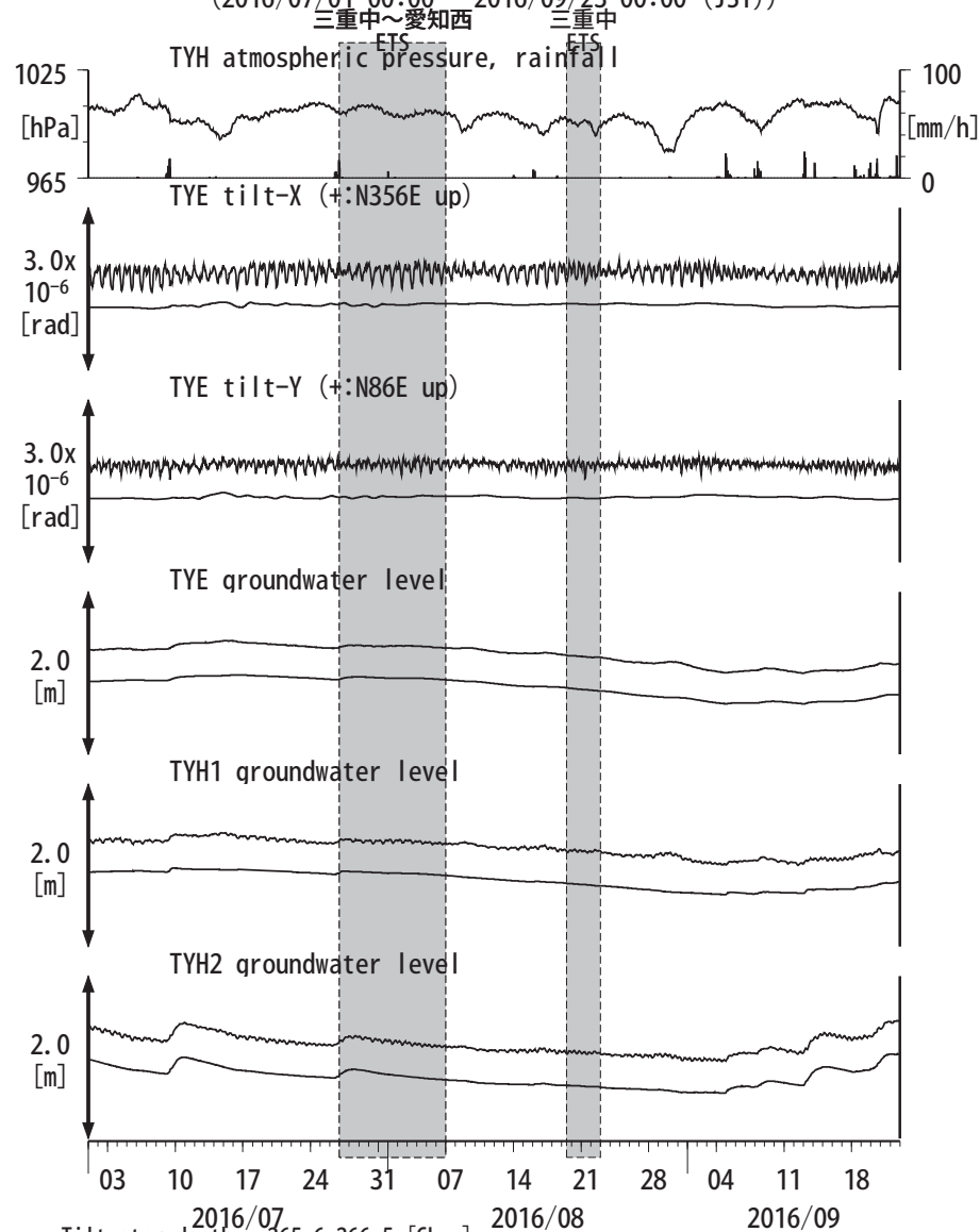
図7: Tilt and groundwater level changes at TYE and TYH 豊橋多米・豊橋 (2016/07/01 00:00 - 2016/09/23 00:00 (JST))
