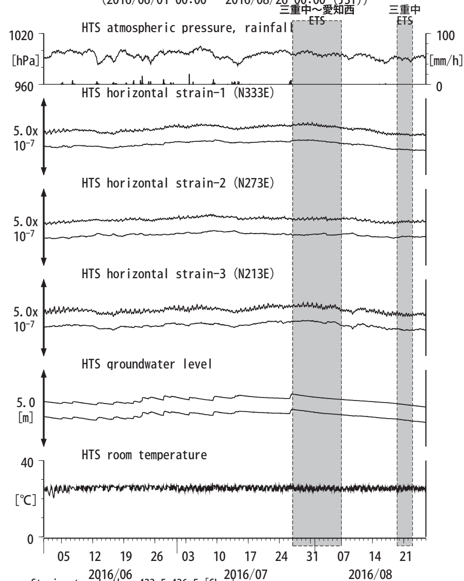
図8: Crustal strain and groundwater level changes at HTS 愛荘香之庄 (2016/06/01 00:00 - 2016/08/26 00:00 (JST))
