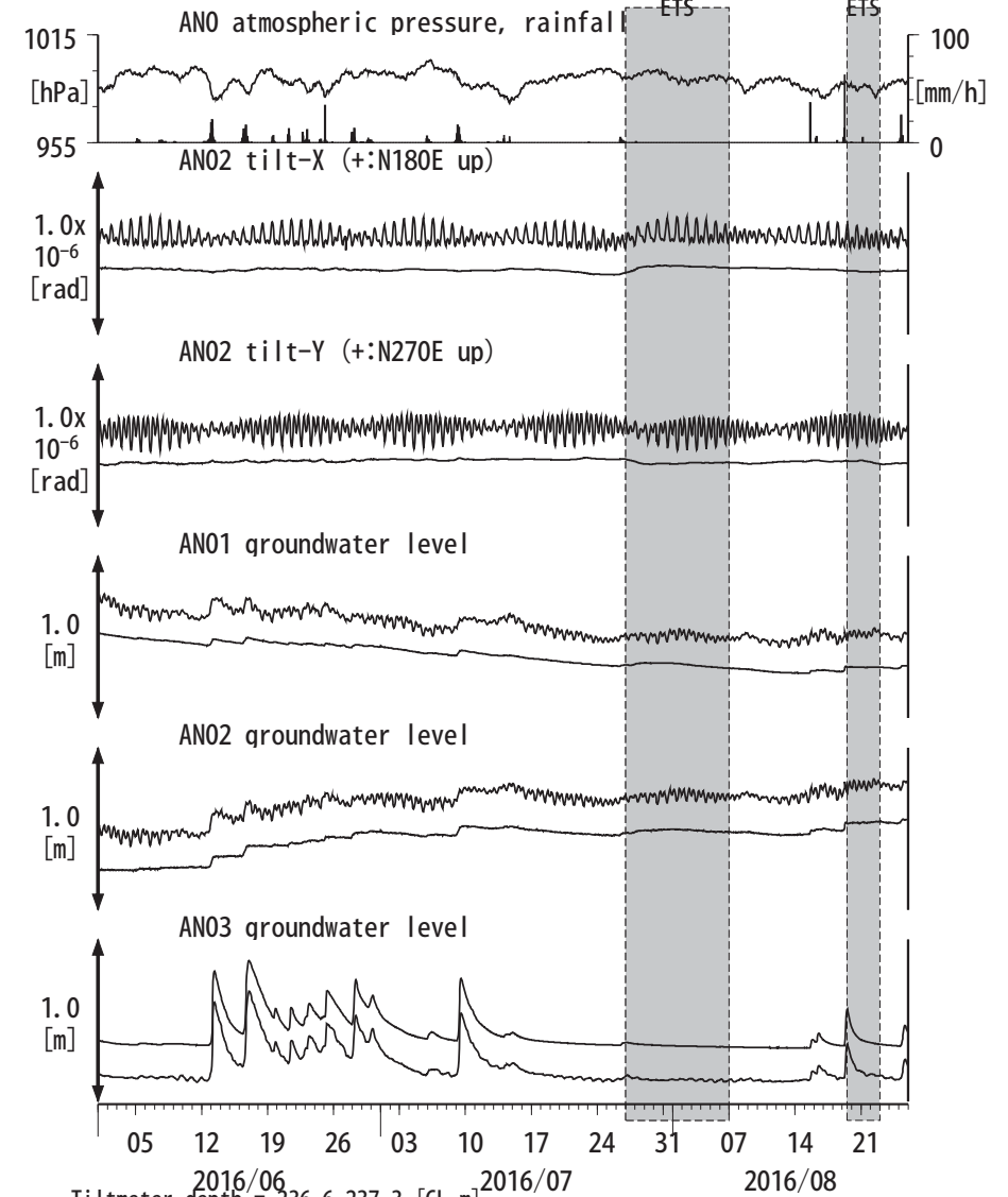
図10: Tilt and groundwater level changes at AN0 津安濃 (時間値) (2016/06/01 00:00 - 2016/08/26 00:00 (JST))
