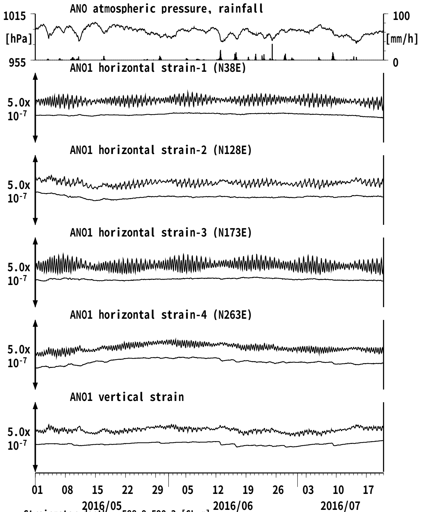
図9: Crustal strains changes at ANO 津安濃 (時間値) (2016/05/01 00:00 - 2016/07/21 00:00 (JST))
