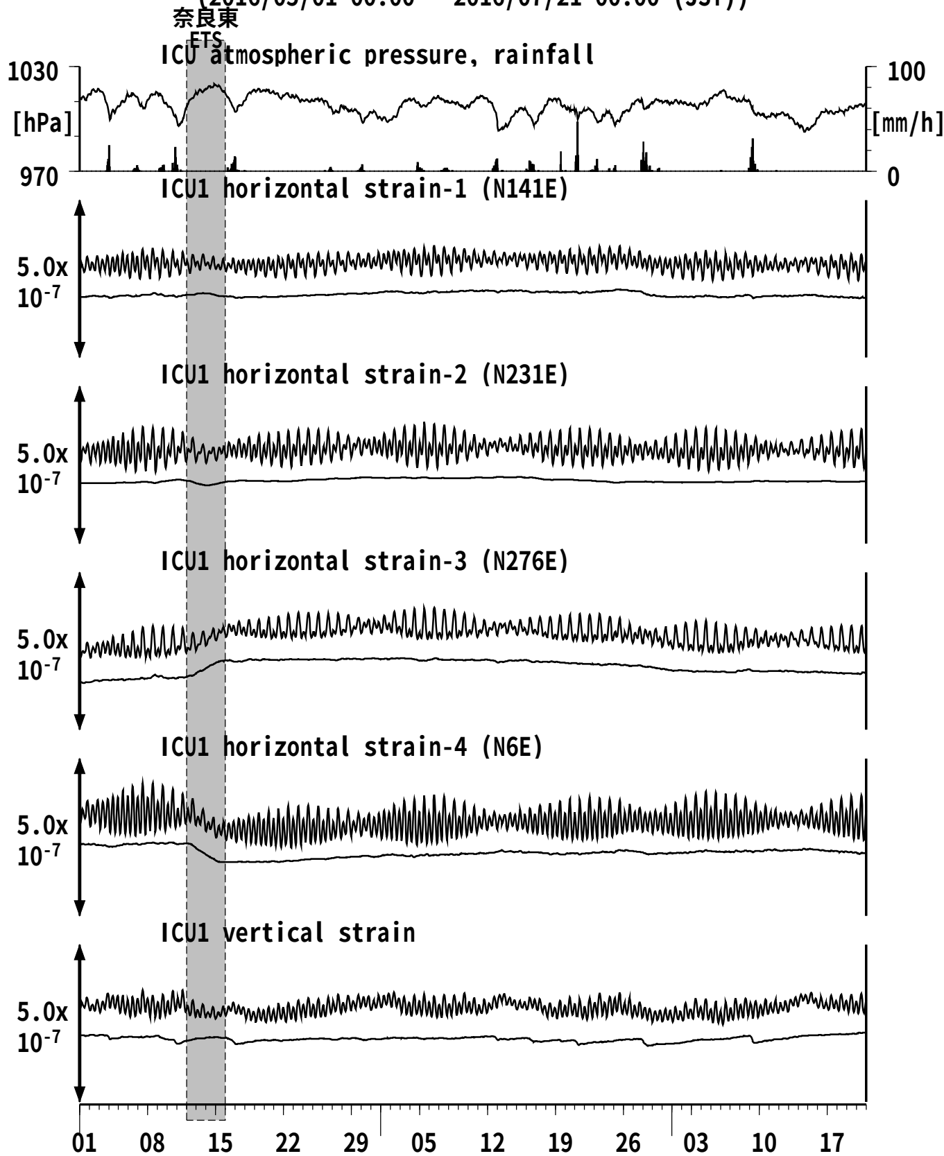
図15: Crustal strain changes at ICU 熊野磯崎 (時間値) (2016/05/01 00:00 - 2016/07/21 00:00 (JST))
