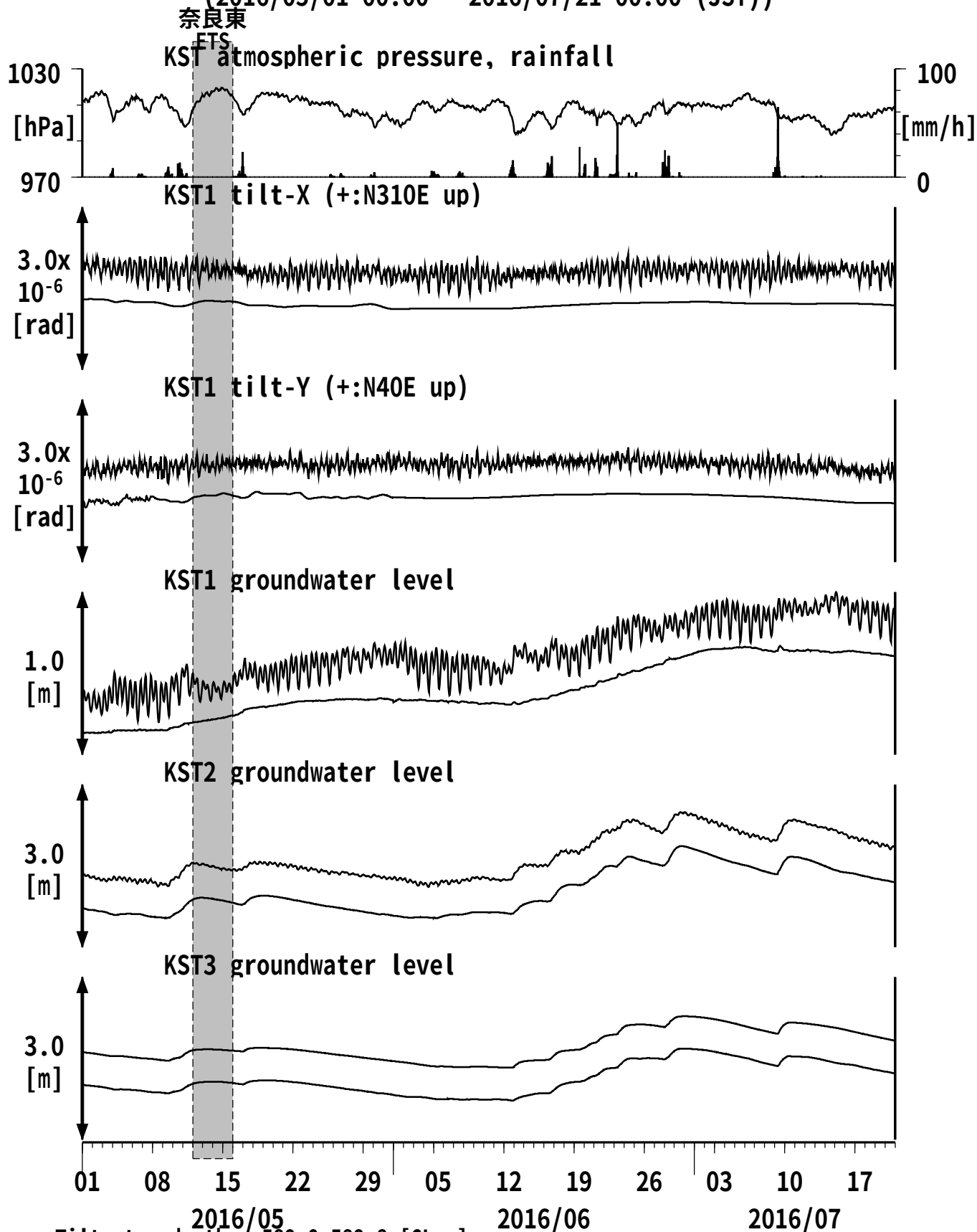
図20: Tilt and groundwater level changes at KST 串本津荷 (時間値) (2016/05/01 00:00 - 2016/07/21 00:00 (JST))
