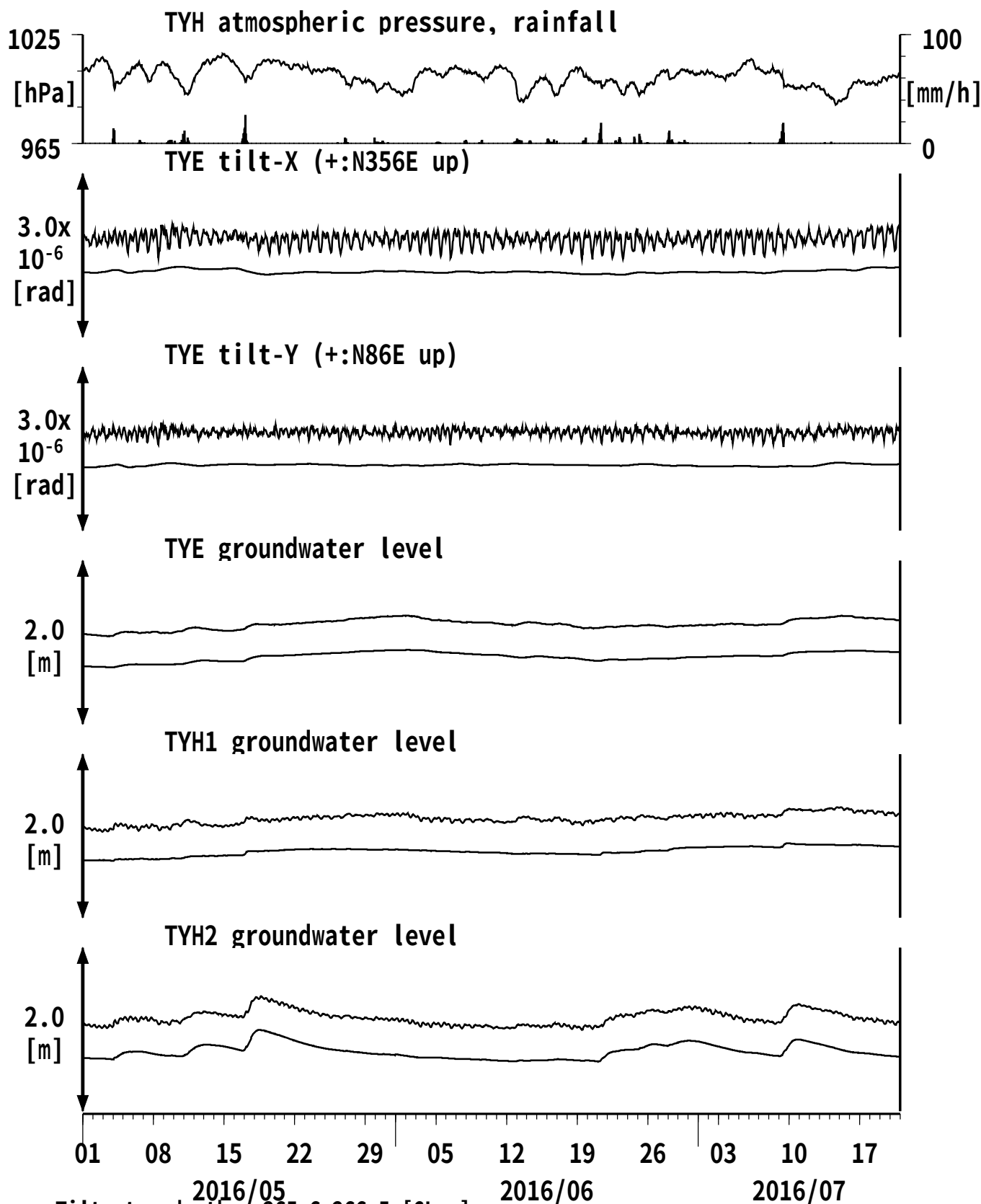
図7: Tilt and groundwater level changes at TYE and TYH 豊橋多米・豊橋 (2016/05/01 00:00 - 2016/07/21 00:00 (JST))
