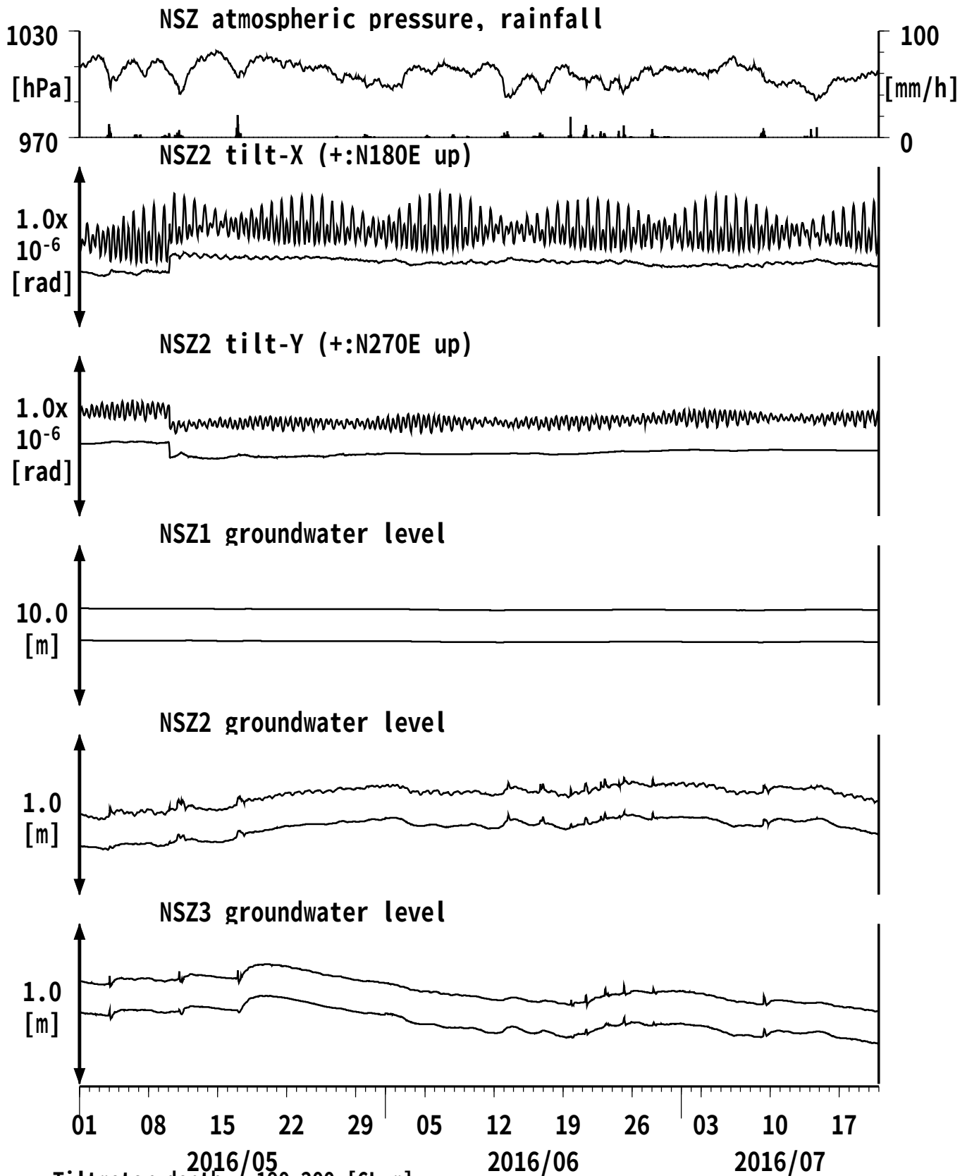
図5: Tilt and groundwater level changes at NSZ 西尾善明 (時間値) (2016/05/01 00:00 - 2016/07/21 00:00 (JST))
