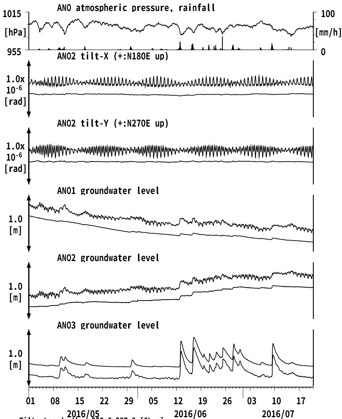
図10: Tilt and groundwater level changes at ANO 津安濃 (時間値) (2016/05/01 00:00 - 2016/07/21 00:00 (JST))
