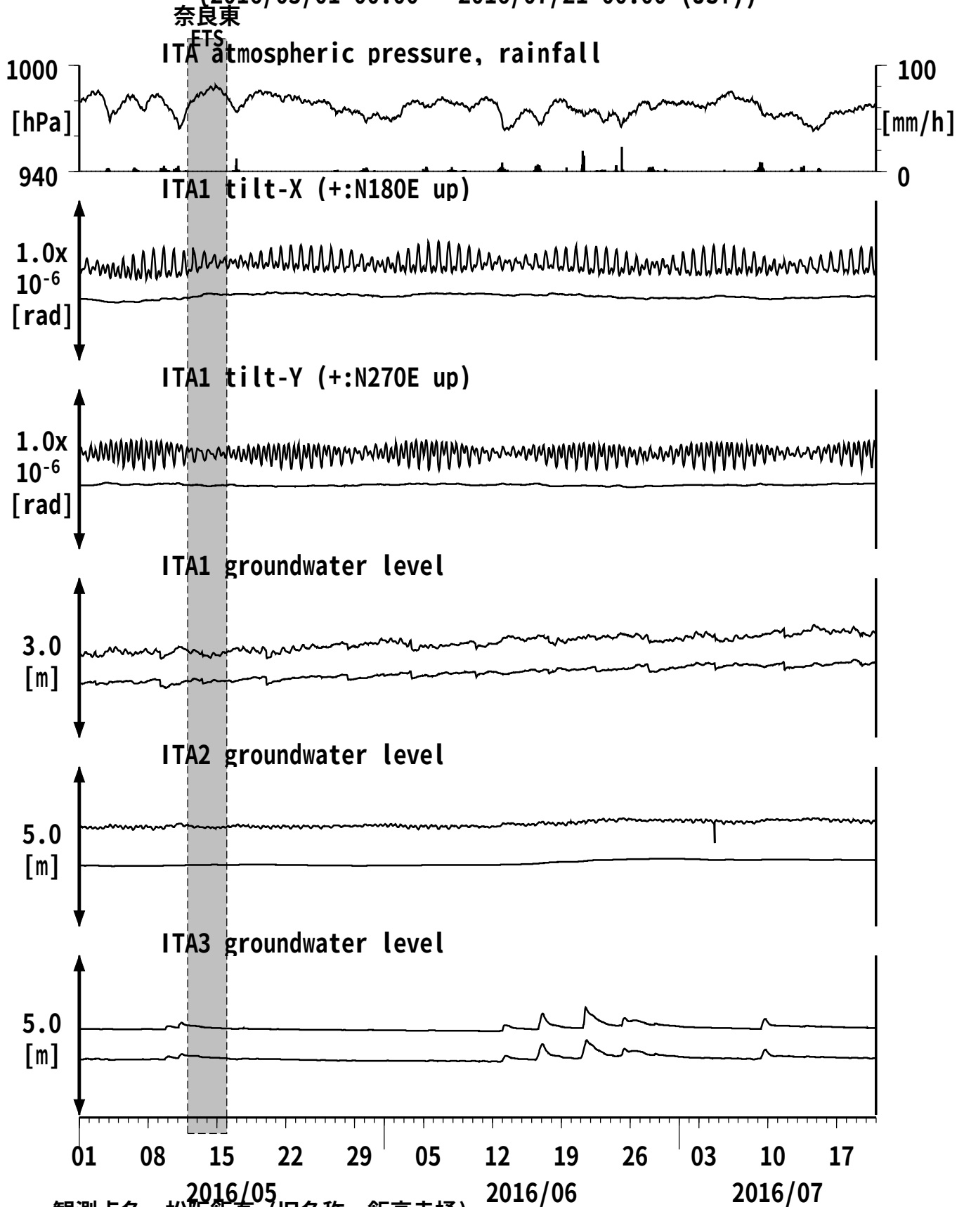
図12: Tilt and groundwater level changes at ITA 松阪飯高 (時間値) (2016/05/01 00:00 - 2016/07/21 00:00 (JST))
