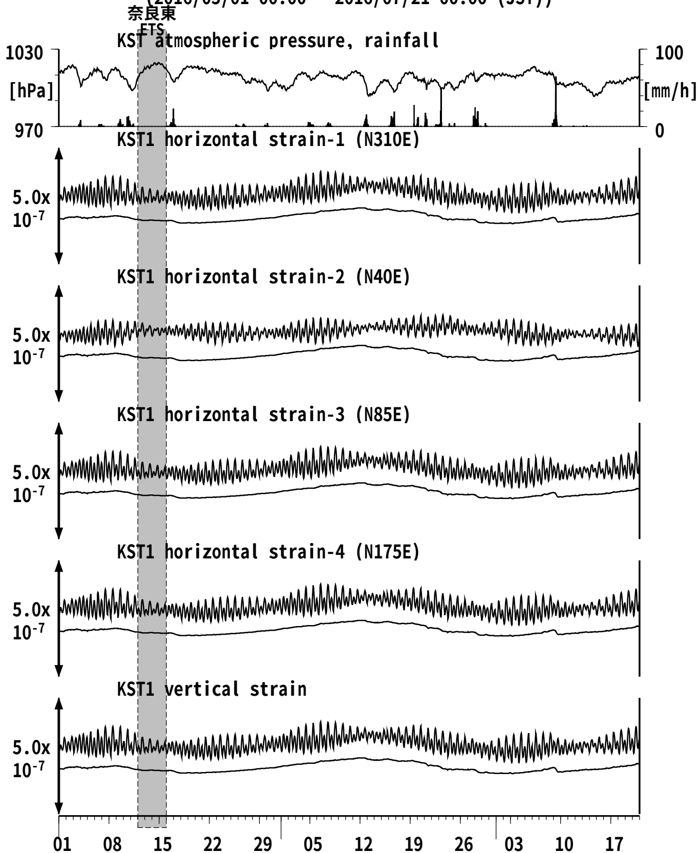
図19: Crustal strain changes at KST 串本津荷 (時間値) (2016/05/01 00:00 - 2016/07/21 00:00 (JST))
