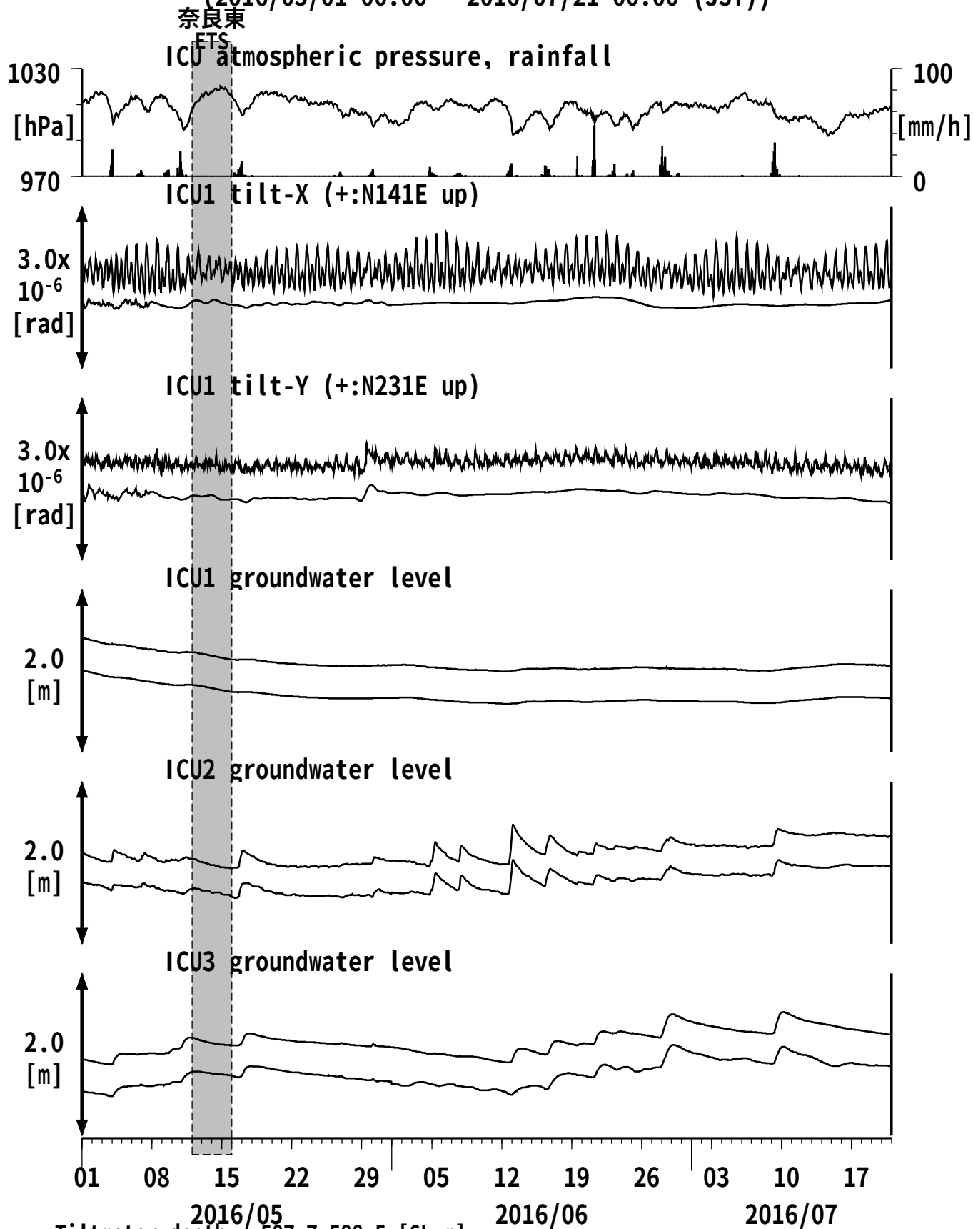
図16: Tilt and groundwater level changes at ICU 熊野磯崎 (時間値) (2016/05/01 00:00 - 2016/07/21 00:00 (JST))
