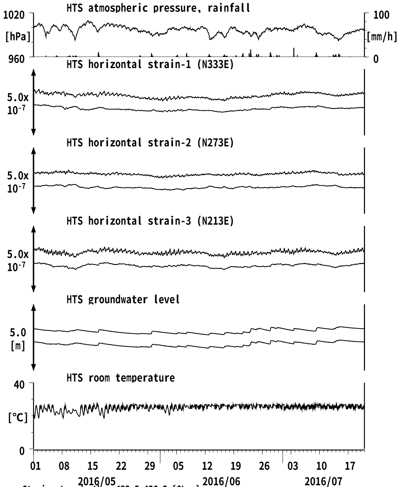
図8: Crustal strain and groundwater level changes at HTS 愛荘香之庄 (2016/05/01 00:00 - 2016/07/21 00:00 (JST))
