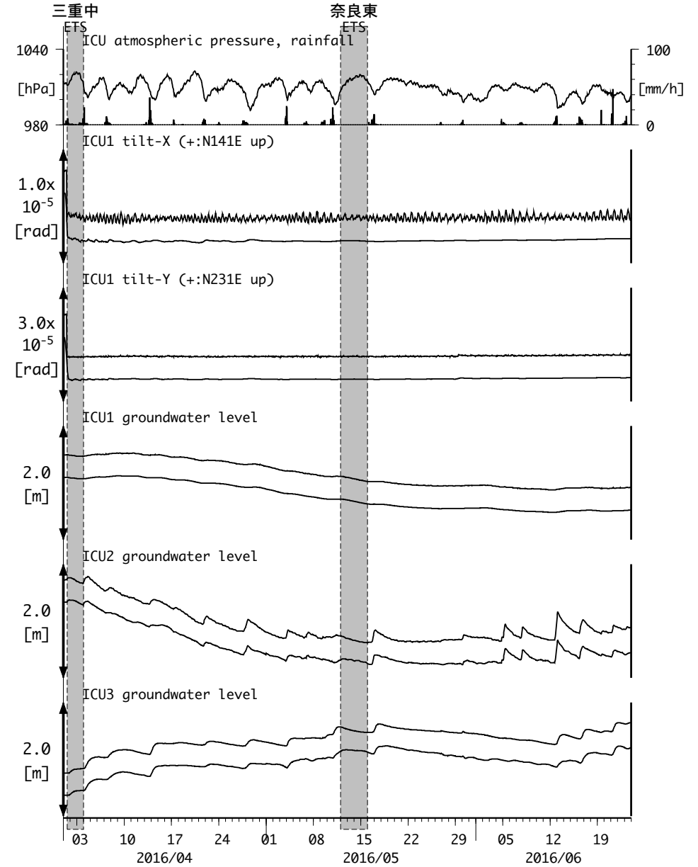
図16 : Tilt and groundwater level changes at ICU 熊野磯崎 (時間値) (2016/04/01 00:00 - 2016/06/24 00:00 (JST))
