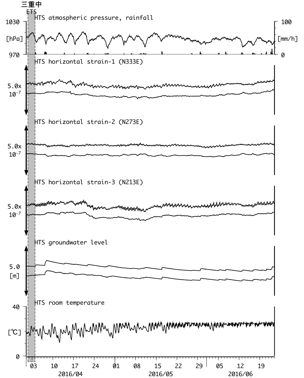
図8: Crustal strain and groundwater level changes at HTS 愛荘香之庄 (2016/04/01 00:00 - 2016/06/24 00:00 (JST))
