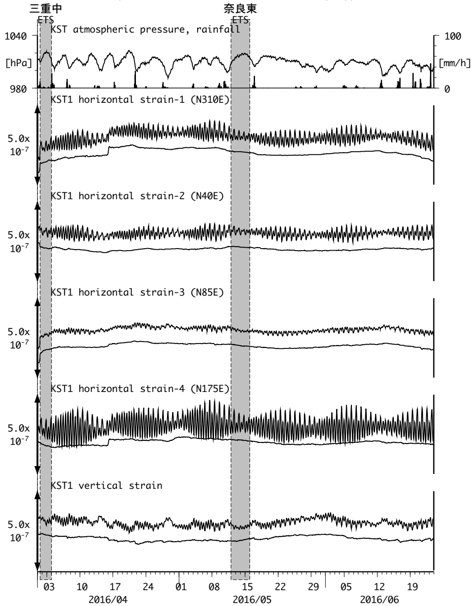
図19 : Crustal strain changes at KST 串本津荷 (時間値) (2016/04/01 00:00 - 2016/06/24 00:00 (JST))
