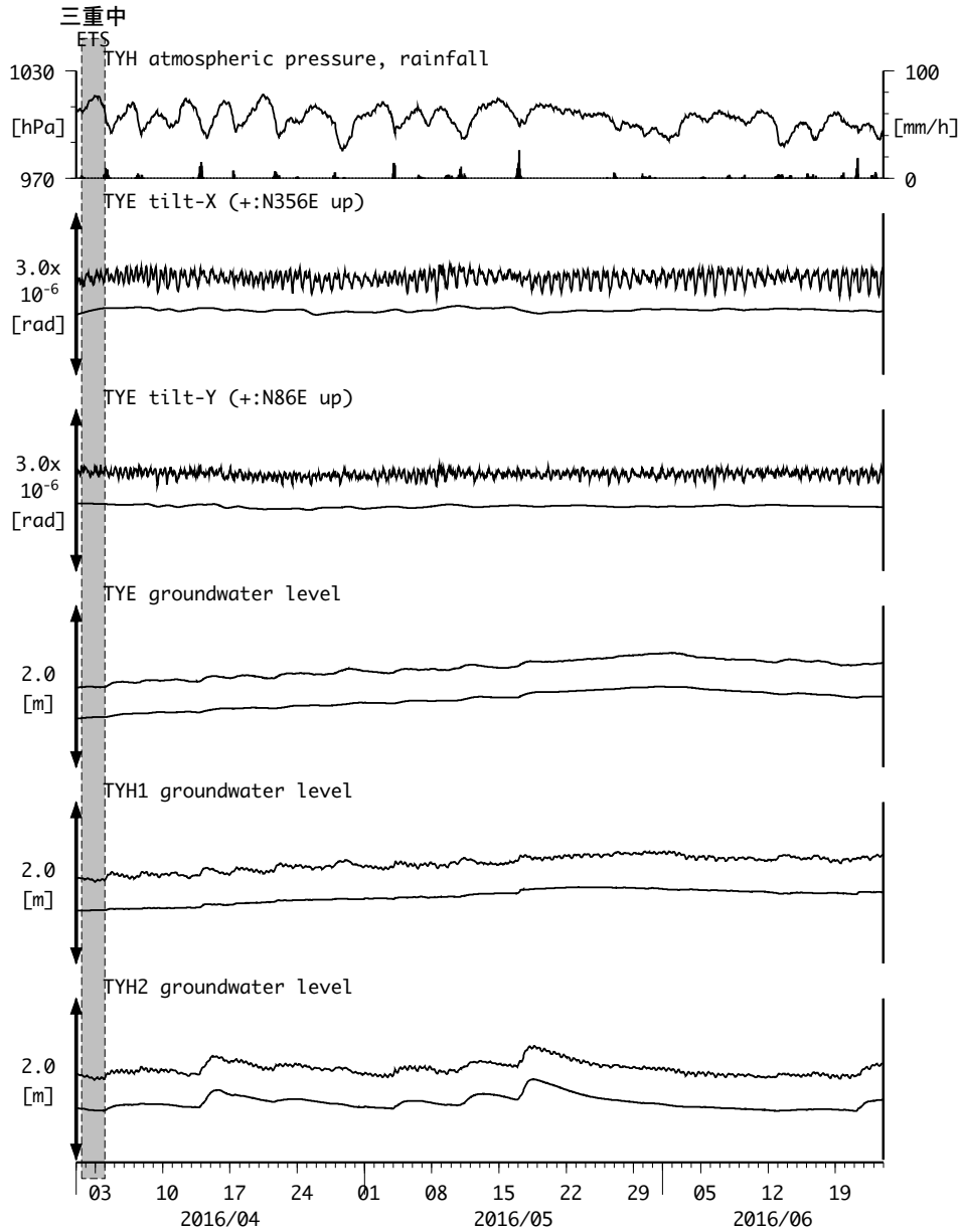
図7: Tilt and groundwater level changes at TYE and TYH 豊橋多米・豊橋 (2016/04/01 00:00 - 2016/06/24 00:00 (JST))
