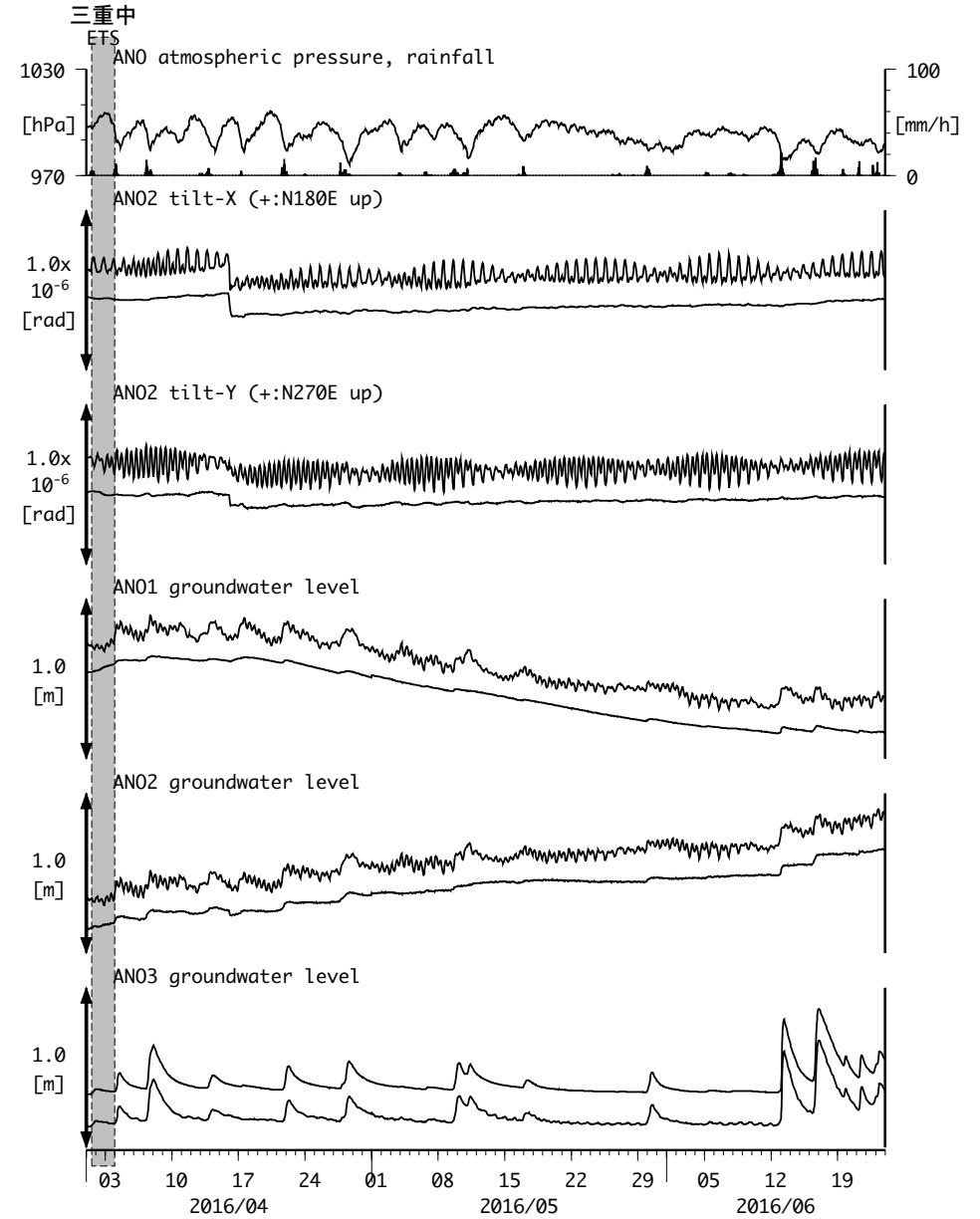
図10 : Tilt and groundwater level changes at ANO 津安濃 (時間値) (2016/04/01 00:00 - 2016/06/24 00:00 (JST))
