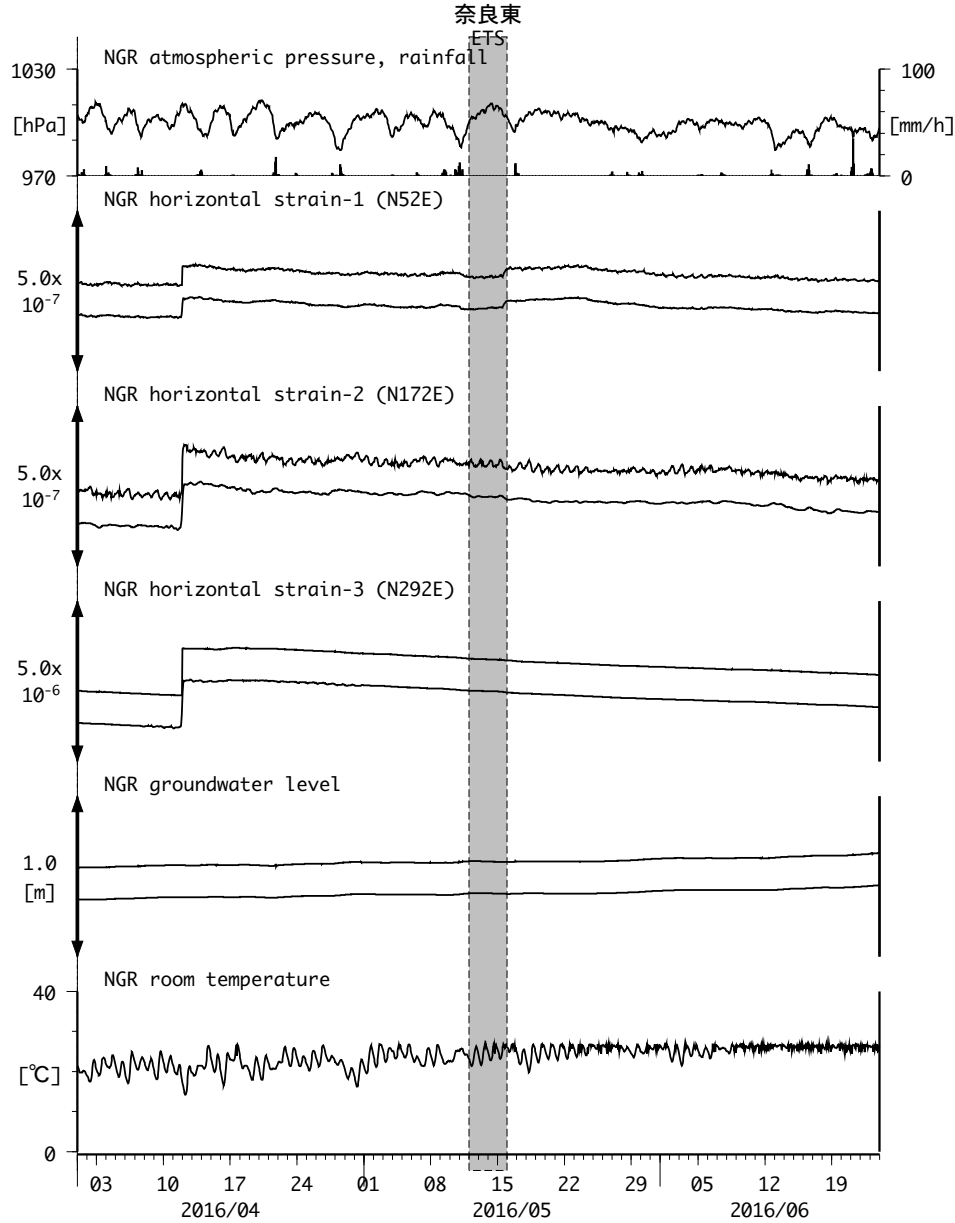
図21: Crustal strain and groundwater level changes at 岩出東坂本 (時間値) (2016/04/01 00:00 - 2016/06/24 00:00 (JST))
