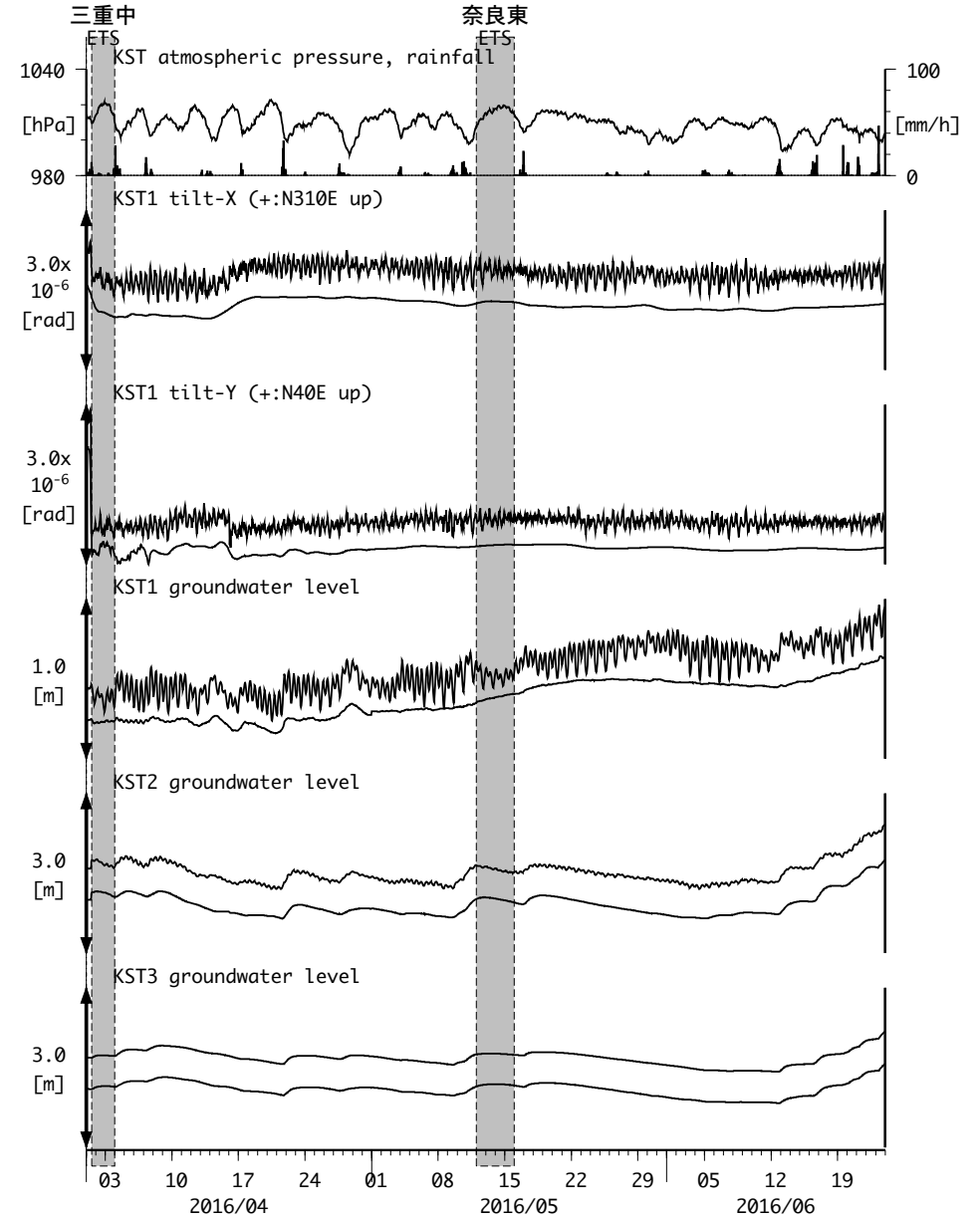
図20 : Tilt and groundwater level changes at KST 串本津荷 (時間値) (2016/04/01 00:00 - 2016/06/24 00:00 (JST))
