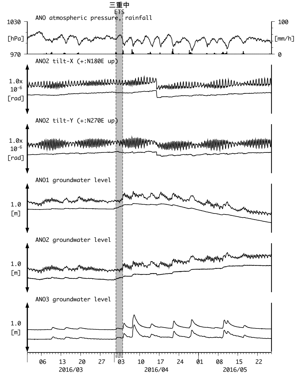
図10 : Tilt and groundwater level changes at ANO 津安濃 (時間値) (2016/03/01 00:00 - 2016/05/27 00:00 (JST))
