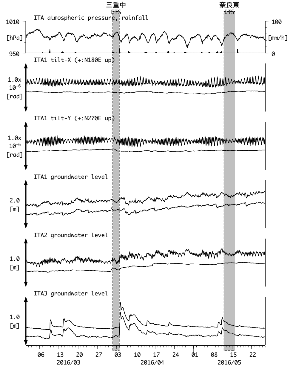
図12: Tilt and groundwater level changes at ITA 松阪飯高 (時間値) (2016/03/01 00:00 - 2016/05/27 00:00 (JST))
