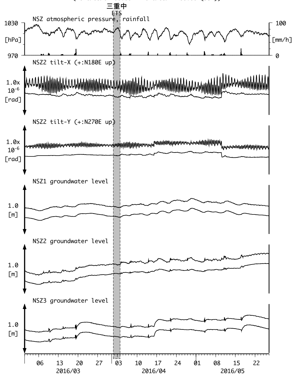
図5: Tilt and groundwater level changes at NSZ 西尾善明 (時間値) (2016/03/01 00:00 - 2016/05/27 00:00 (JST))
