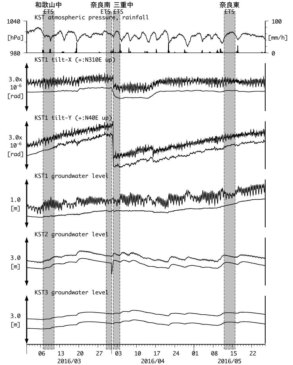
図20 : Tilt and groundwater level changes at KST 串本津荷 (時間値) (2016/03/01 00:00 - 2016/05/27 00:00 (JST))
