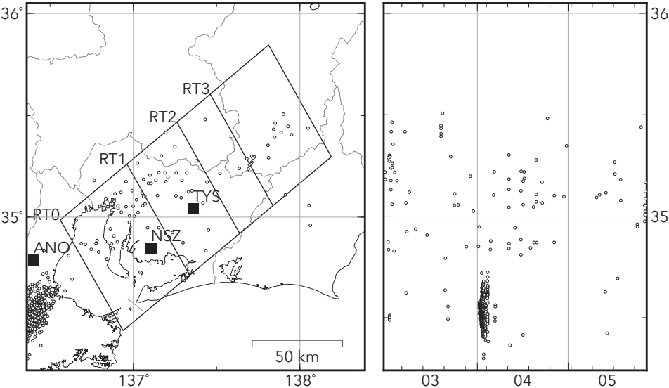
2016/03/01 00:00:00 - 2016/05/27 00:00:00 Total = 680 Deep low-frequency tremors in Tokai (日値) (2016/03/01 00:00 - 2016/05/27 00:00 (JST))
