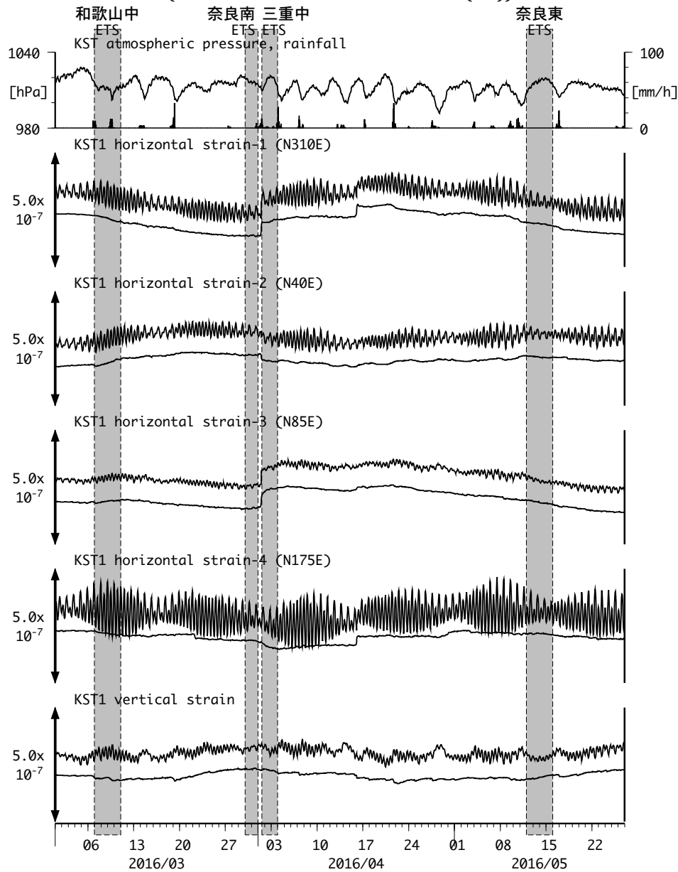
図19 : Crustal strain changes at KST 串本津荷 (時間値) (2016/03/01 00:00 - 2016/05/27 00:00 (JST))
