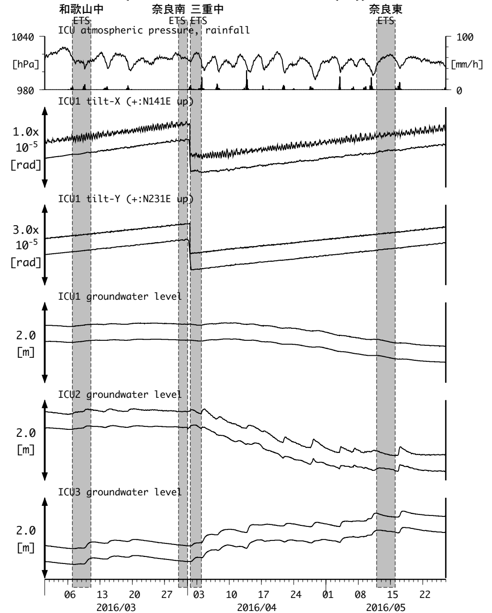
図16 : Tilt and groundwater level changes at ICU 熊野磯崎 (時間値) (2016/03/01 00:00 - 2016/05/27 00:00 (JST))
