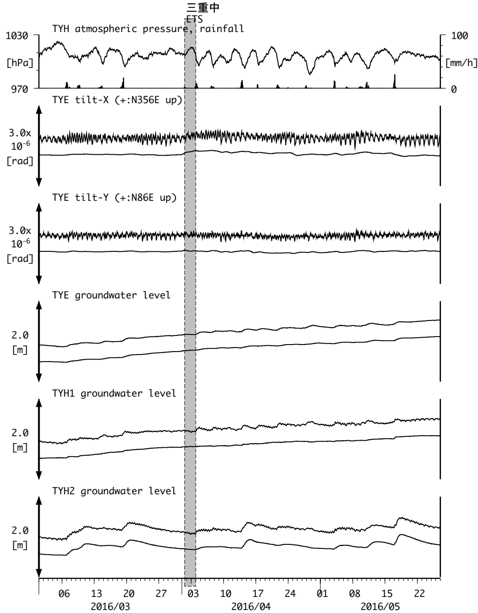
図7: Tilt and groundwater level changes at TYE and TYH 豊橋多米・豊橋 (2016/03/01 00:00 - 2016/05/27 00:00 (JST))
