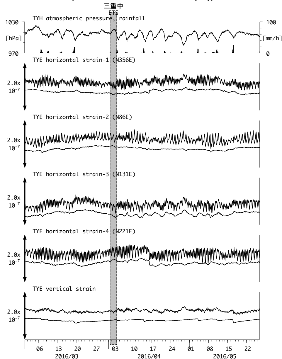
図6: Crustal strain changes at TYE 豊橋多米 (時間値) (2016/03/01 00:00 - 2016/05/27 00:00 (JST))
