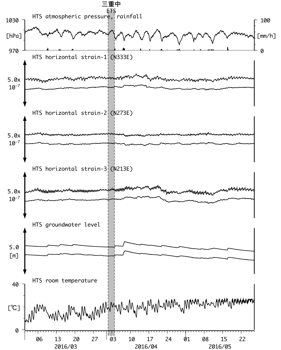
図8: Crustal strain and groundwater level changes at HTS 愛荘香之庄 (2016/03/01 00:00 - 2016/05/27 00:00 (JST))
