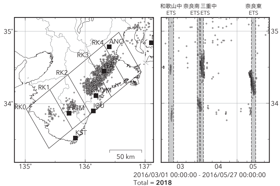
Deep low-frequency tremor activities in Kii Peninsula (日値) (2016/03/01 00:00 - 2016/05/27 00:00 (JST))
