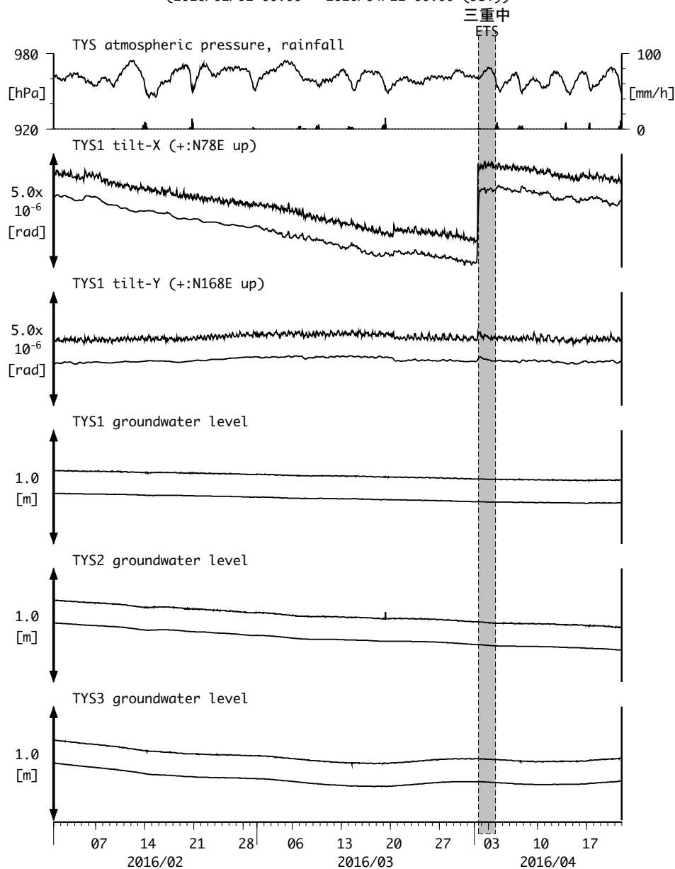
図3: Tilt and groundwater level changes at TYS 豊田神殿 (時間値)
