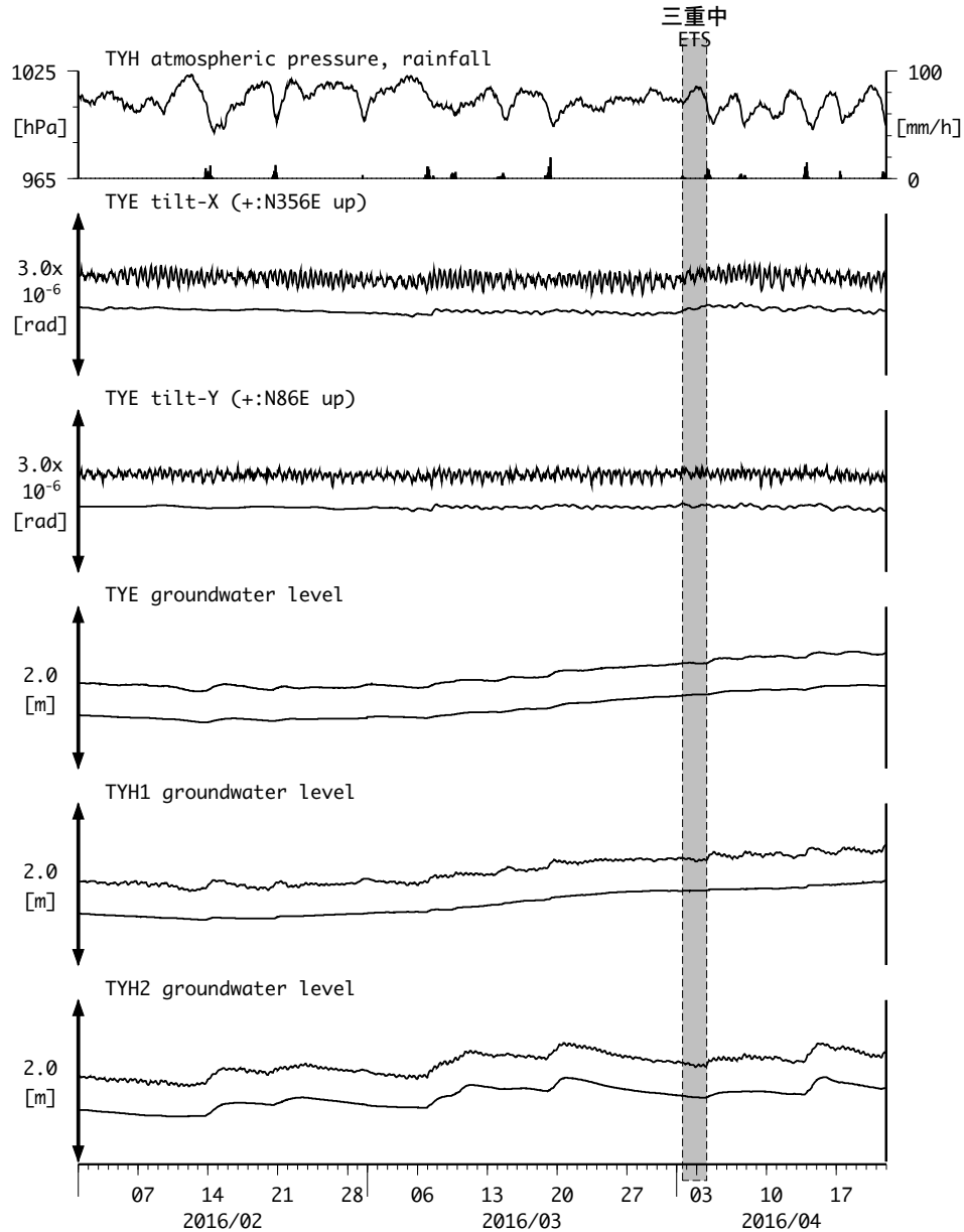
図7: Tilt and groundwater level changes at TYE and TYH 豊橋多米・豊橋 (2016/02/01 00:00 - 2016/04/22 00:00 (JST))
