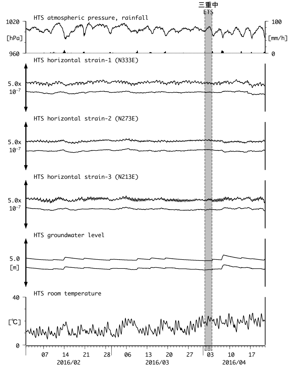
図8: Crustal strain and groundwater level changes at HTS 愛荘香之庄 (2016/02/01 00:00 - 2016/04/22 00:00 (JST))
