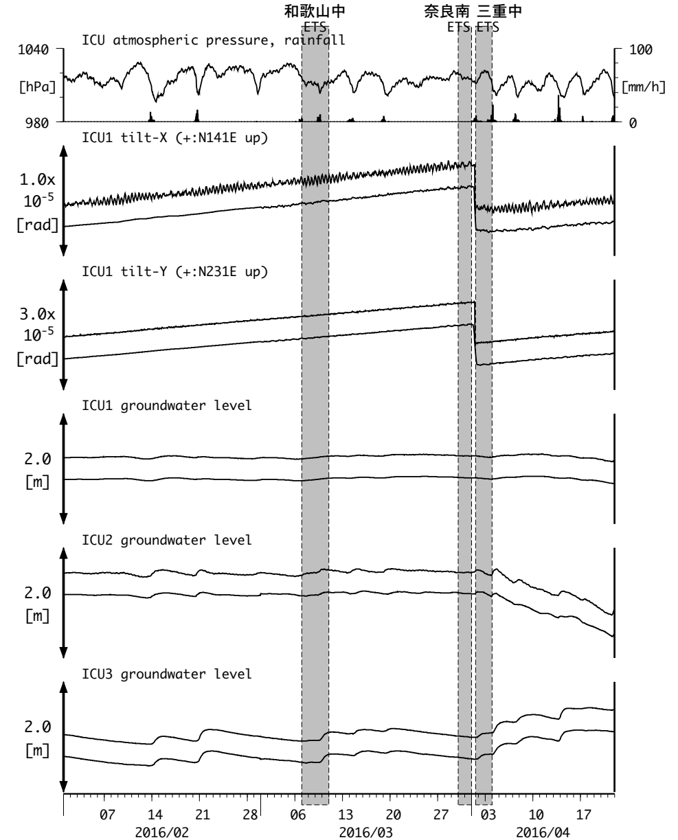
図16 : Tilt and groundwater level changes at ICU 熊野磯崎 (時間値) (2016/02/01 00:00 - 2016/04/22 00:00 (JST))
