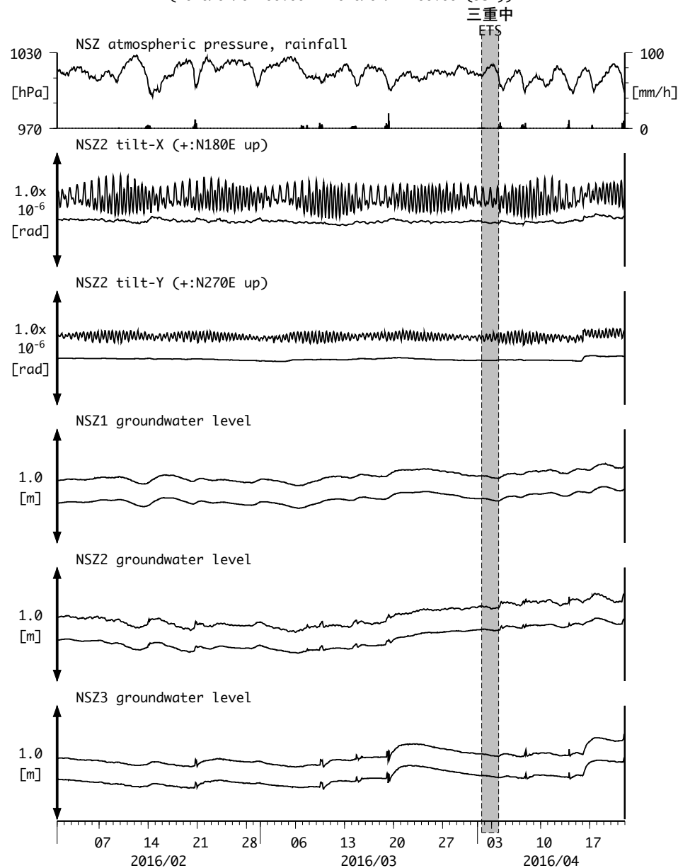
図5: Tilt and groundwater level changes at NSZ 西尾善明 (時間値) (2016/02/01 00:00 - 2016/04/22 00:00 (JST))
