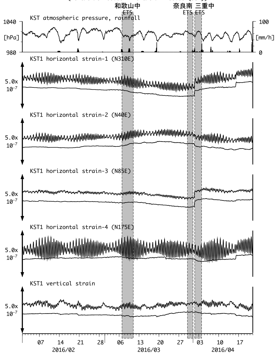
図19 : Crustal strain changes at KST 串本津荷 (時間値) (2016/02/01 00:00 - 2016/04/22 00:00 (JST))
