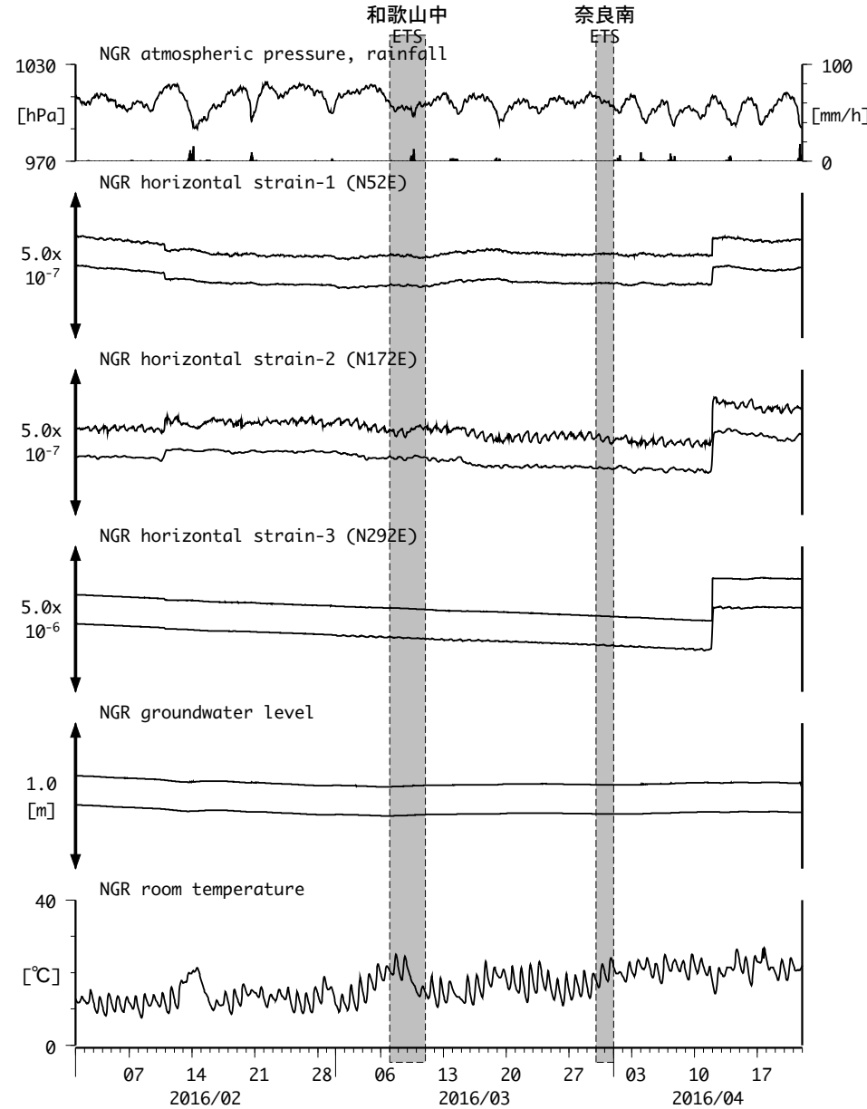
図21: Crustal strain and groundwater level changes at 岩出東坂本 (時間値) (2016/02/01 00:00 - 2016/04/22 00:00 (JST))
