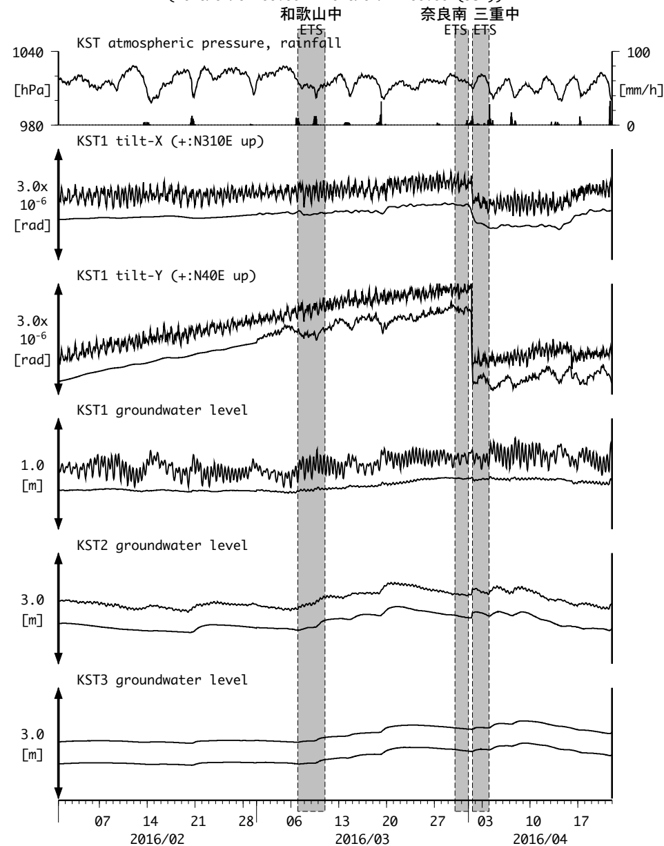
図20 : Tilt and groundwater level changes at KST 串本津荷 (時間値) (2016/02/01 00:00 - 2016/04/22 00:00 (JST))
