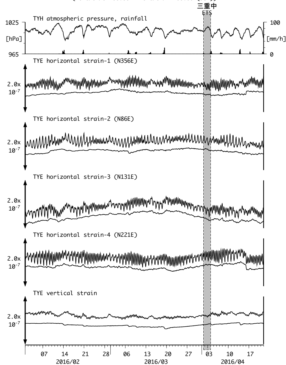
図6: Crustal strain changes at TYE 豊橋多米 (時間値) (2016/02/01 00:00 - 2016/04/22 00:00 (JST))
