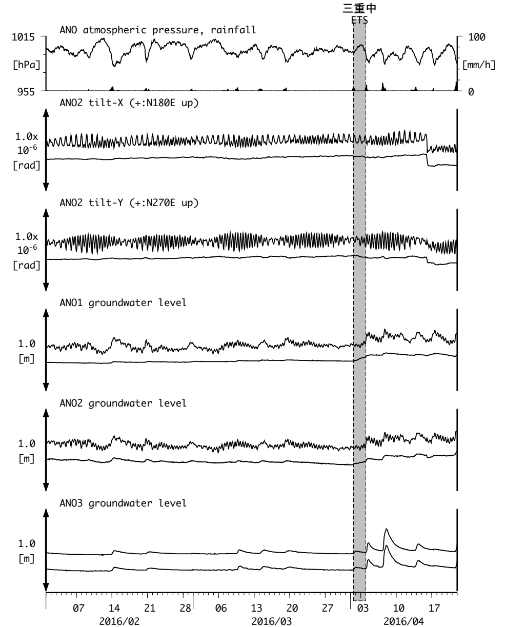
図10 : Tilt and groundwater level changes at ANO 津安濃 (時間値) (2016/02/01 00:00 - 2016/04/22 00:00 (JST))
