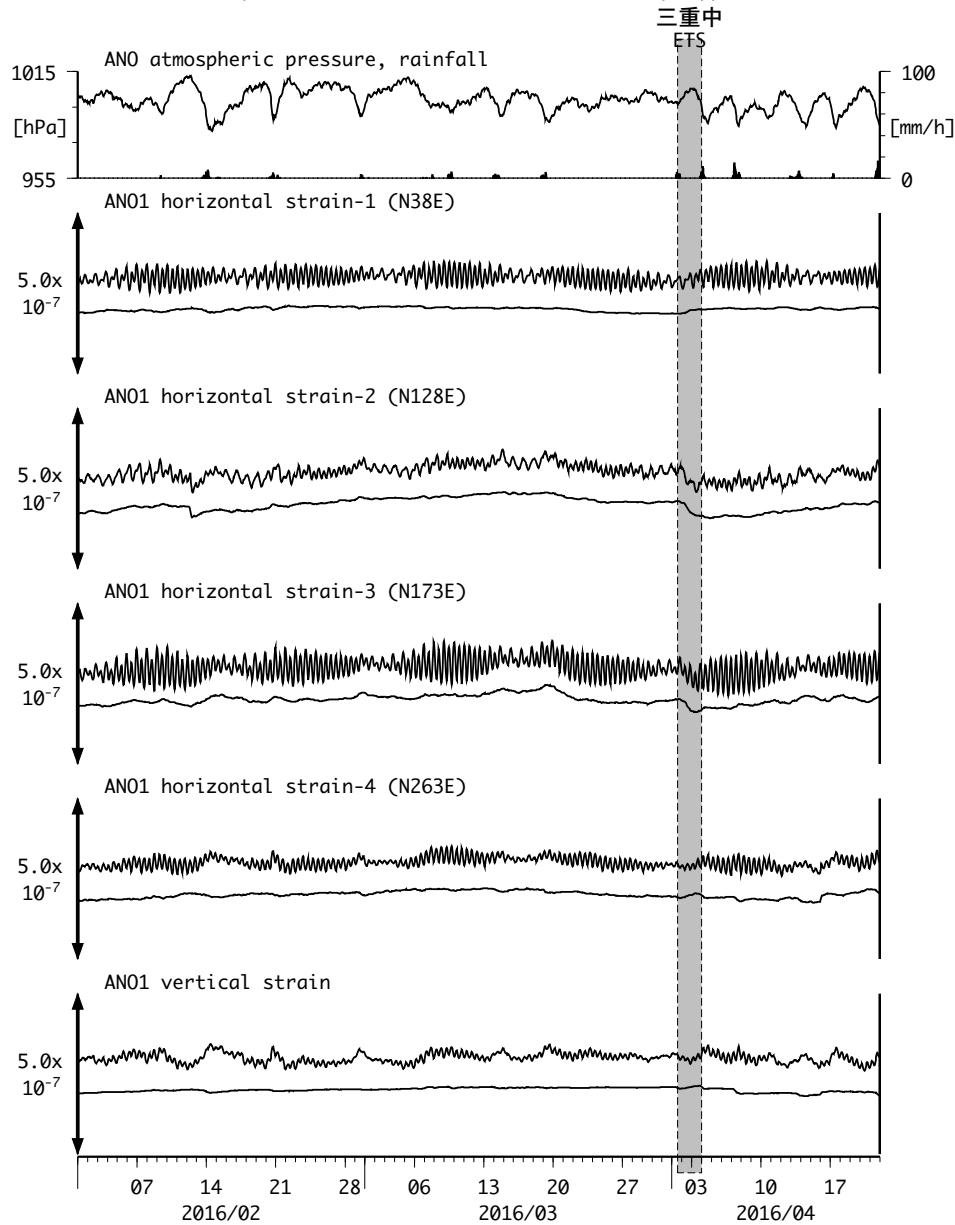
図9 : Crustal strains changes at ANO 津安濃 (時間値) (2016/02/01 00:00 - 2016/04/22 00:00 (JST))
