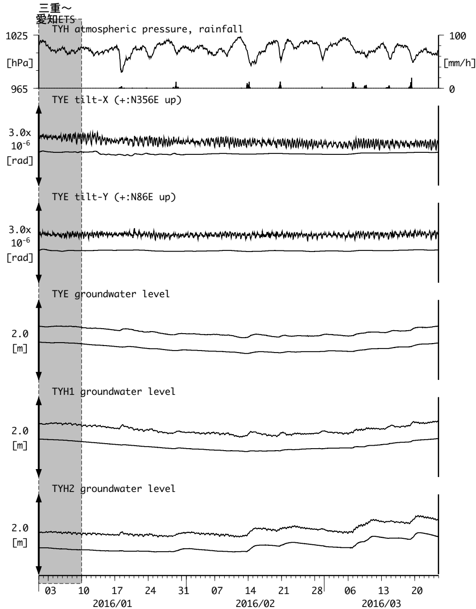
図7: Tilt and groundwater level changes at TYE and TYH 豊橋多米・豊橋 (2016/01/01 00:00 - 2016/03/25 00:00 (JST))
