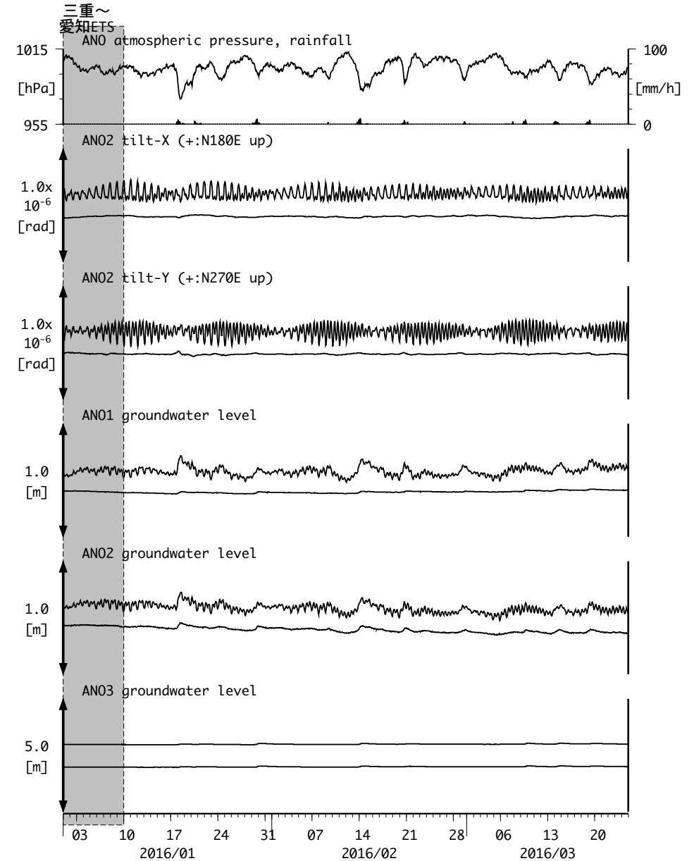
図10 : Tilt and groundwater level changes at ANO 津安濃 (時間値) (2016/01/01 00:00 - 2016/03/25 00:00 (JST))
