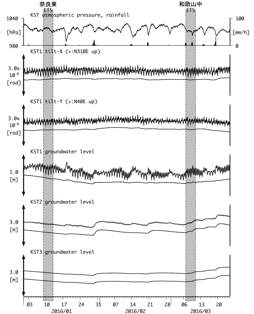
図20 : Tilt and groundwater level changes at KST 串本津荷 (時間値) (2016/01/01 00:00 - 2016/03/25 00:00 (JST))
