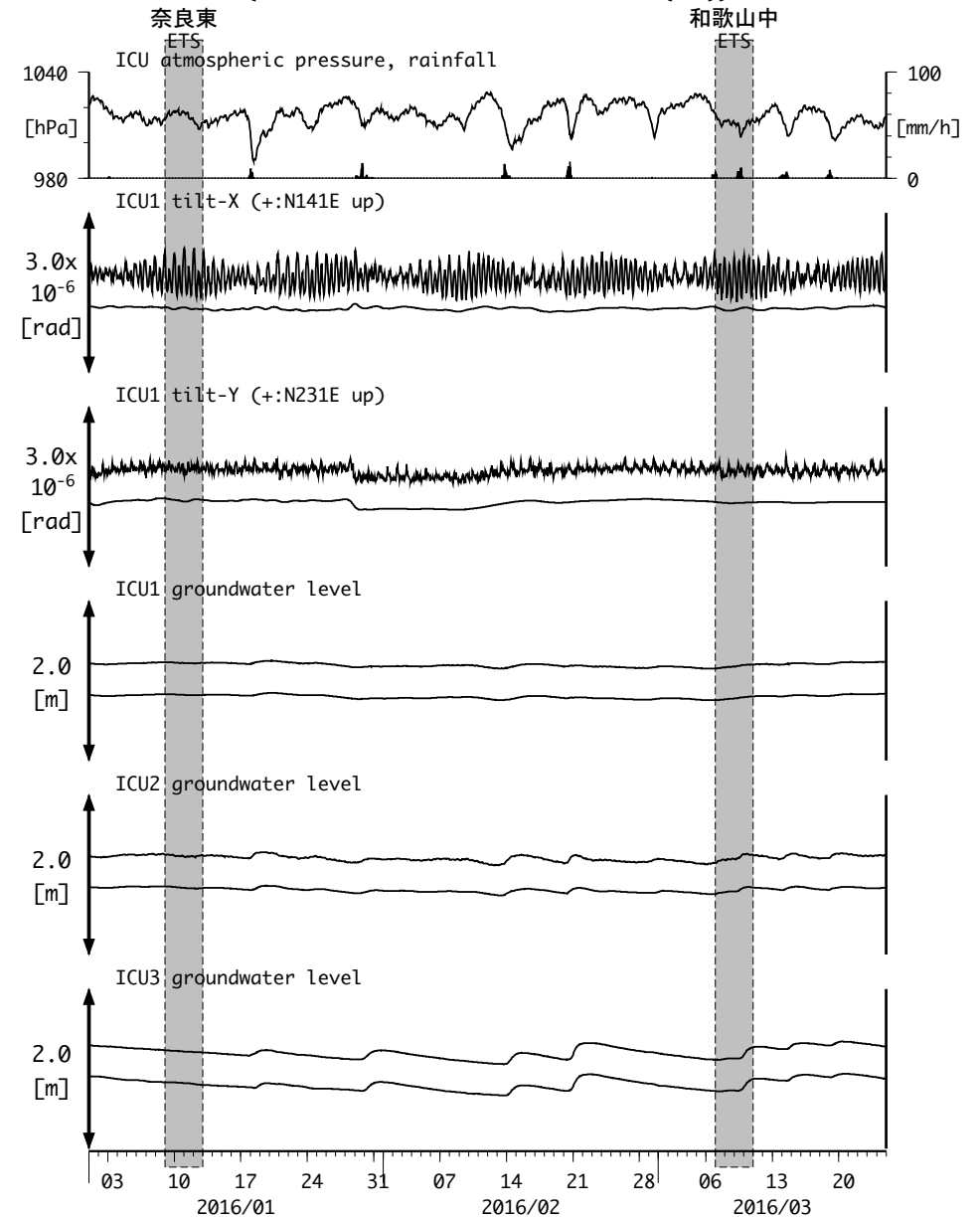
図16 : Tilt and groundwater level changes at ICU 熊野磯崎 (時間値) (2016/01/01 00:00 - 2016/03/25 00:00 (JST))
