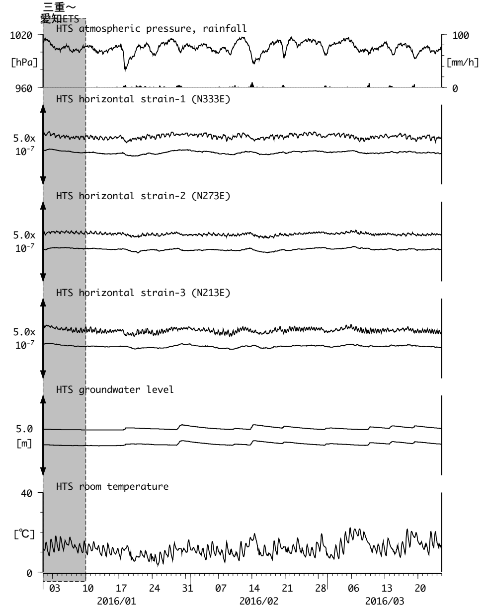
図8: Crustal strain and groundwater level changes at HTS 愛荘香之庄 (2016/01/01 00:00 - 2016/03/25 00:00 (JST))
