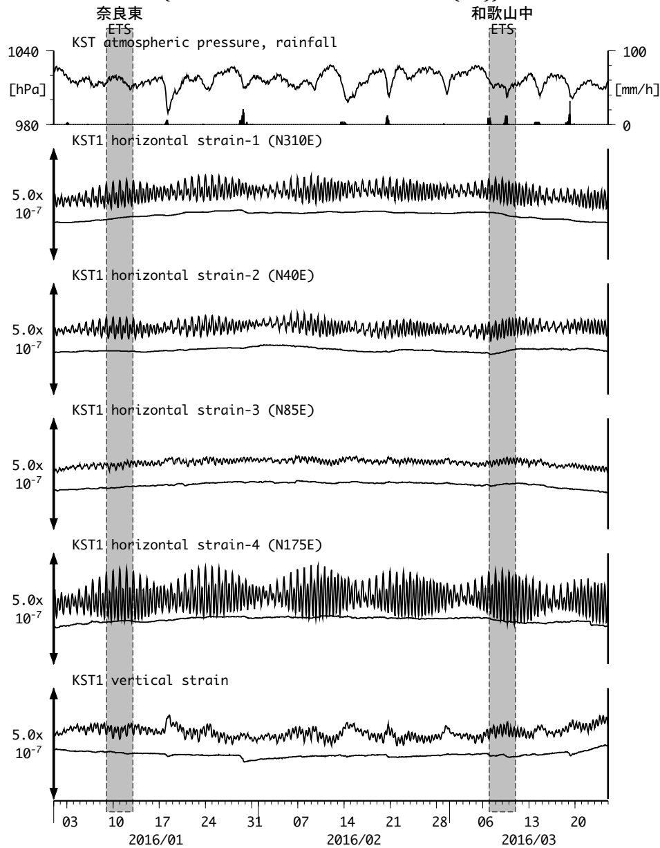
図19 : Crustal strain changes at KST 串本津荷 (時間値) (2016/01/01 00:00 - 2016/03/25 00:00 (JST))
