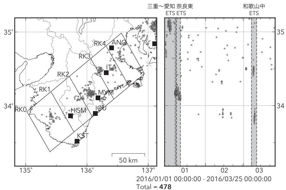
Deep low-frequency tremor activities in Kii Peninsula (日値) (2016/01/01 00:00 - 2016/03/25 00:00 (JST))
