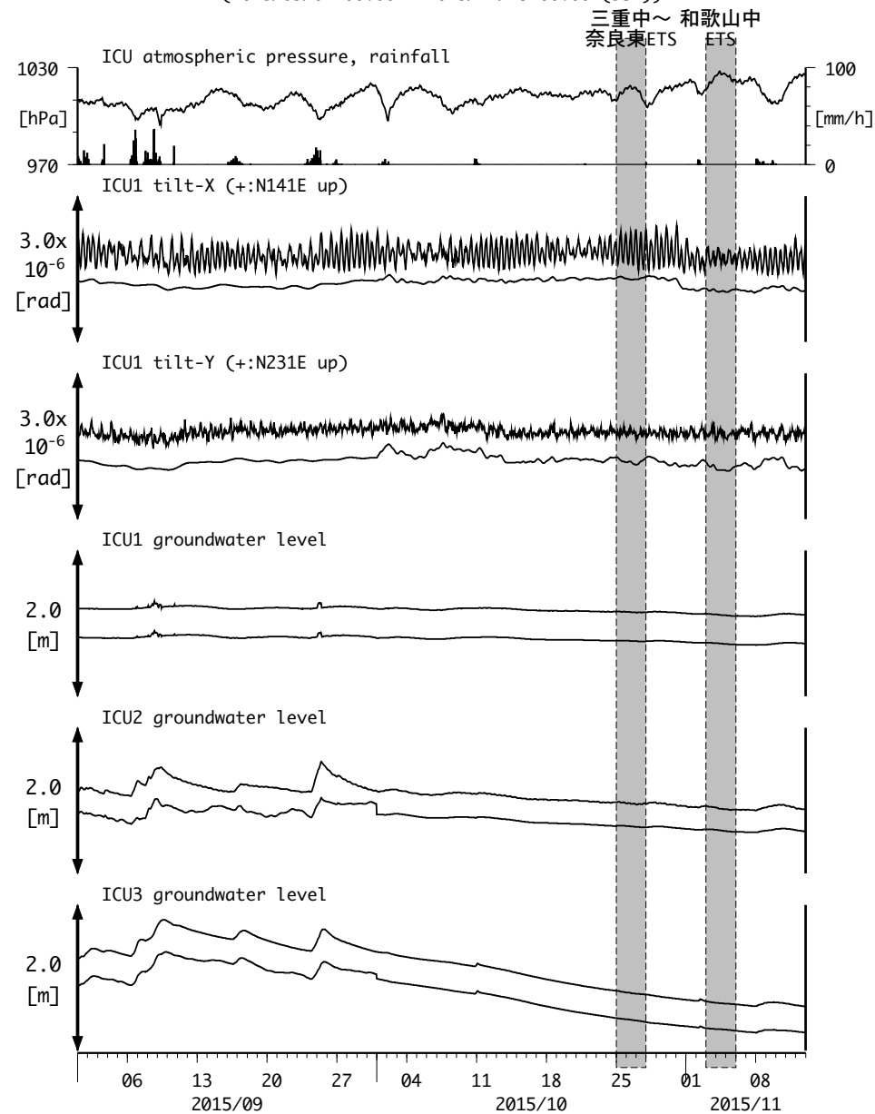
図16 : Tilt and groundwater level changes at ICU 熊野磯崎 (時間値) (2015/09/01 00:00 - 2015/11/13 00:00 (JST))
