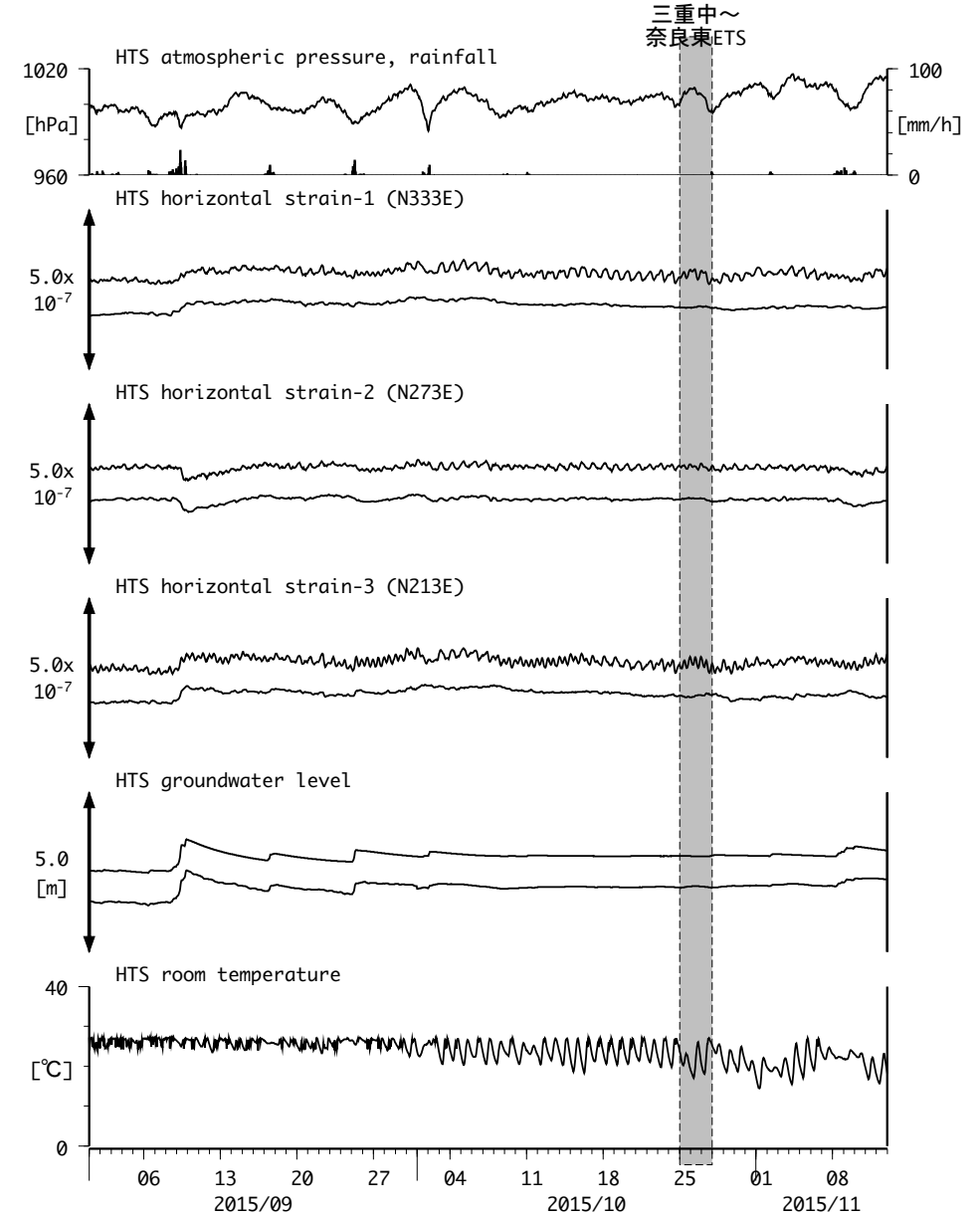
図8: Crustal strain and groundwater level changes at HTS 愛荘香之庄 (2015/09/01 00:00 - 2015/11/13 00:00 (JST))
