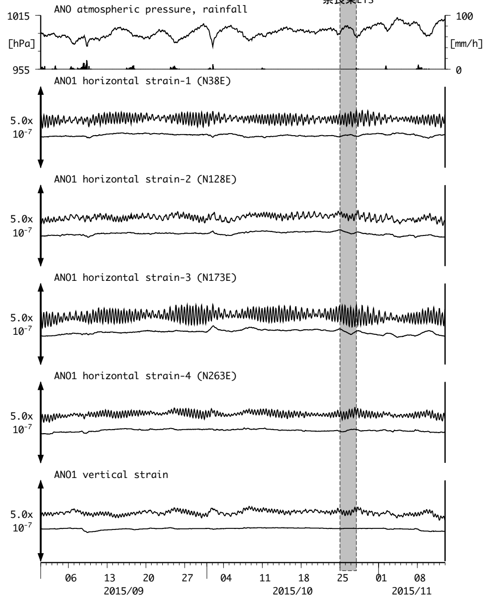
図9 : Crustal strains changes at ANO 津安濃 (時間値) (2015/09/01 00:00 - 2015/11/13 00:00 (JST))
