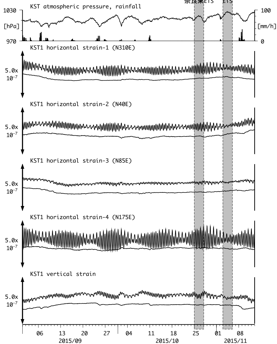
図19 : Crustal strain changes at KST 串本津荷 (時間値) (2015/09/01 00:00 - 2015/11/13 00:00 (JST))
