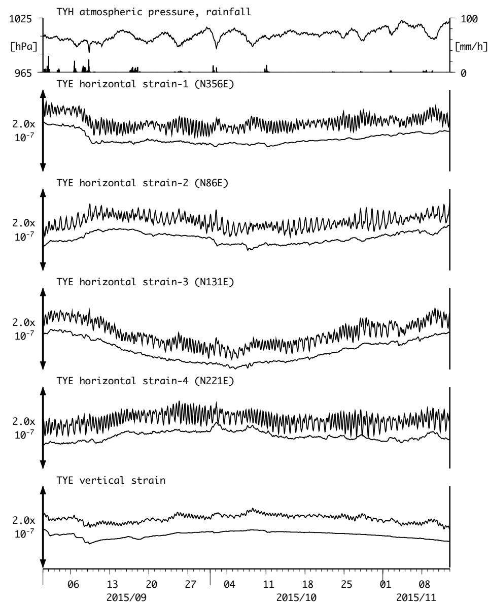
図6: Crustal strain changes at TYE 豊橋多米 (時間値) (2015/09/01 00:00 - 2015/11/13 00:00 (JST))
