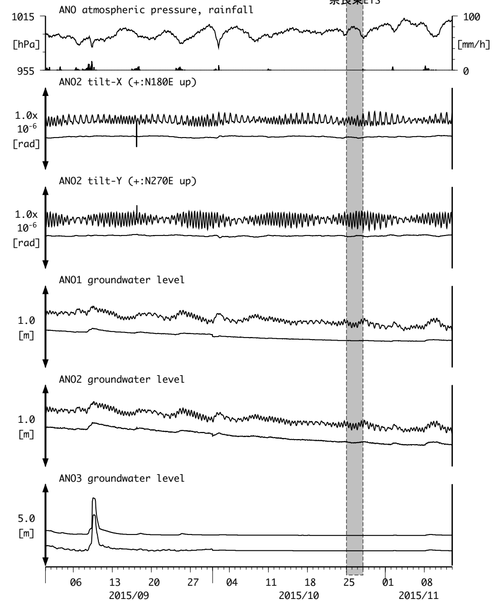
図10 : Tilt and groundwater level changes at ANO 津安濃 (時間値) (2015/09/01 00:00 - 2015/11/13 00:00 (JST))
