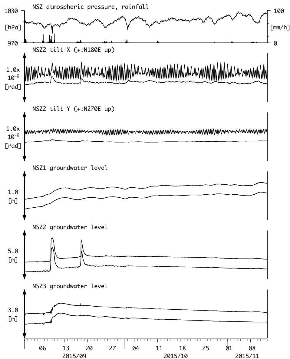
図5: Tilt and groundwater level changes at NSZ 西尾善明 (時間値) (2015/09/01 00:00 - 2015/11/13 00:00 (JST))
