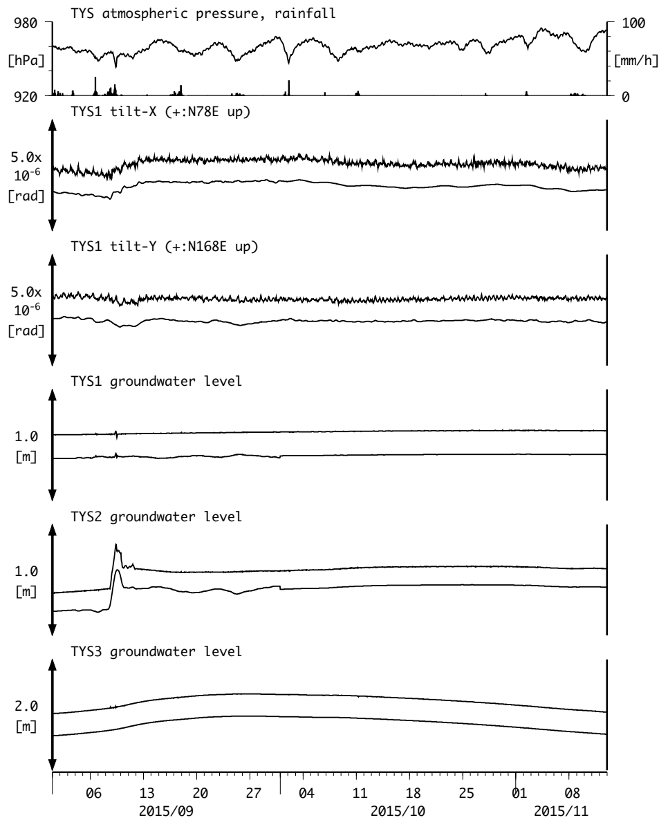
図3: Tilt and groundwater level changes at TYS 豊田神殿 (時間値) (2015/09/01 00:00 - 2015/11/13 00:00 (JST))
