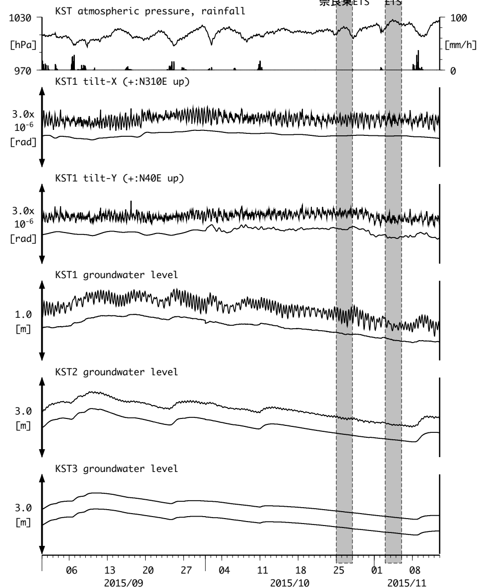
図20 : Tilt and groundwater level changes at KST 串本津荷 (時間値) (2015/09/01 00:00 - 2015/11/13 00:00 (JST))
