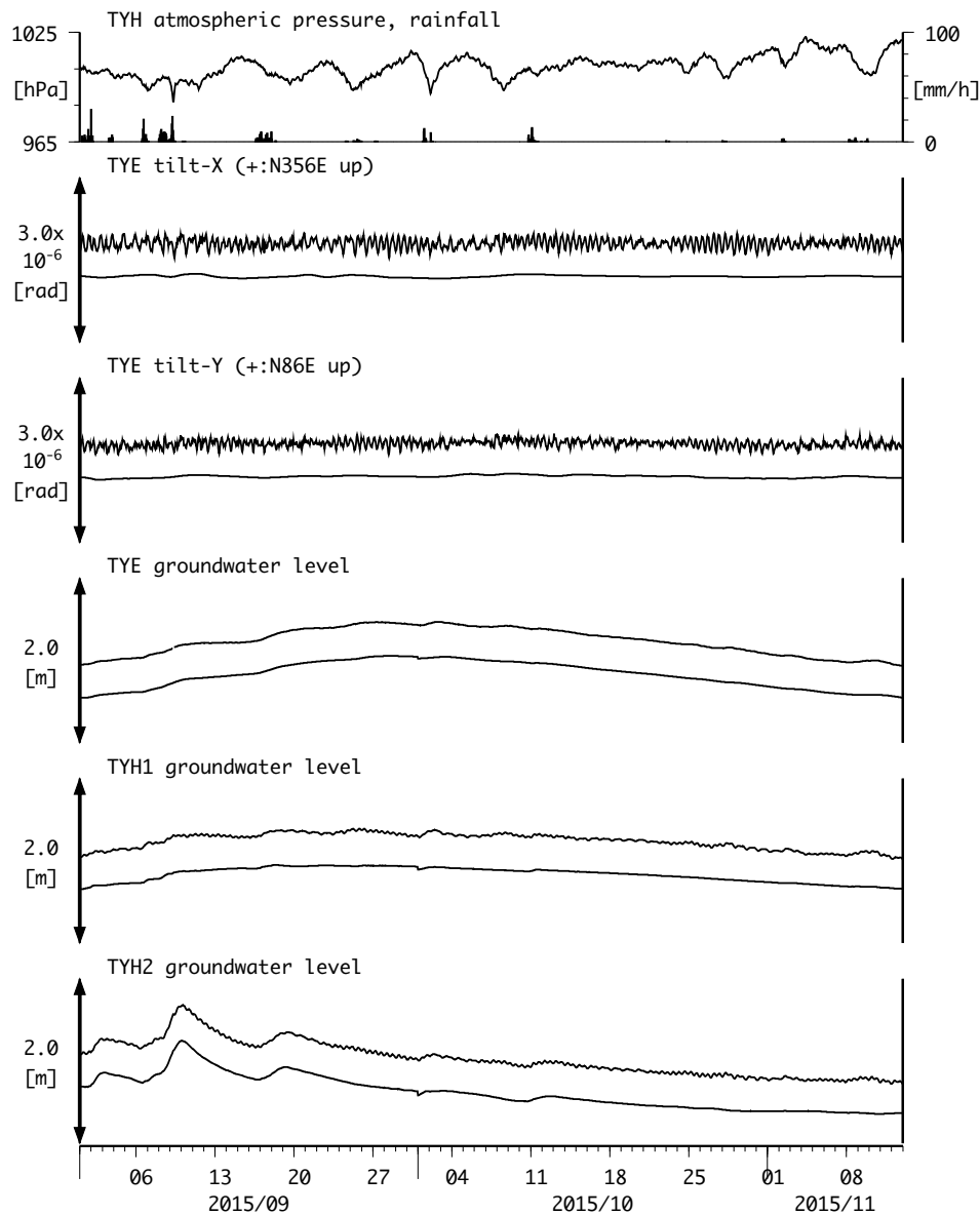
図7: Tilt and groundwater level changes at TYE and TYH 豊橋多米・豊橋 (2015/09/01 00:00 - 2015/11/13 00:00 (JST))
