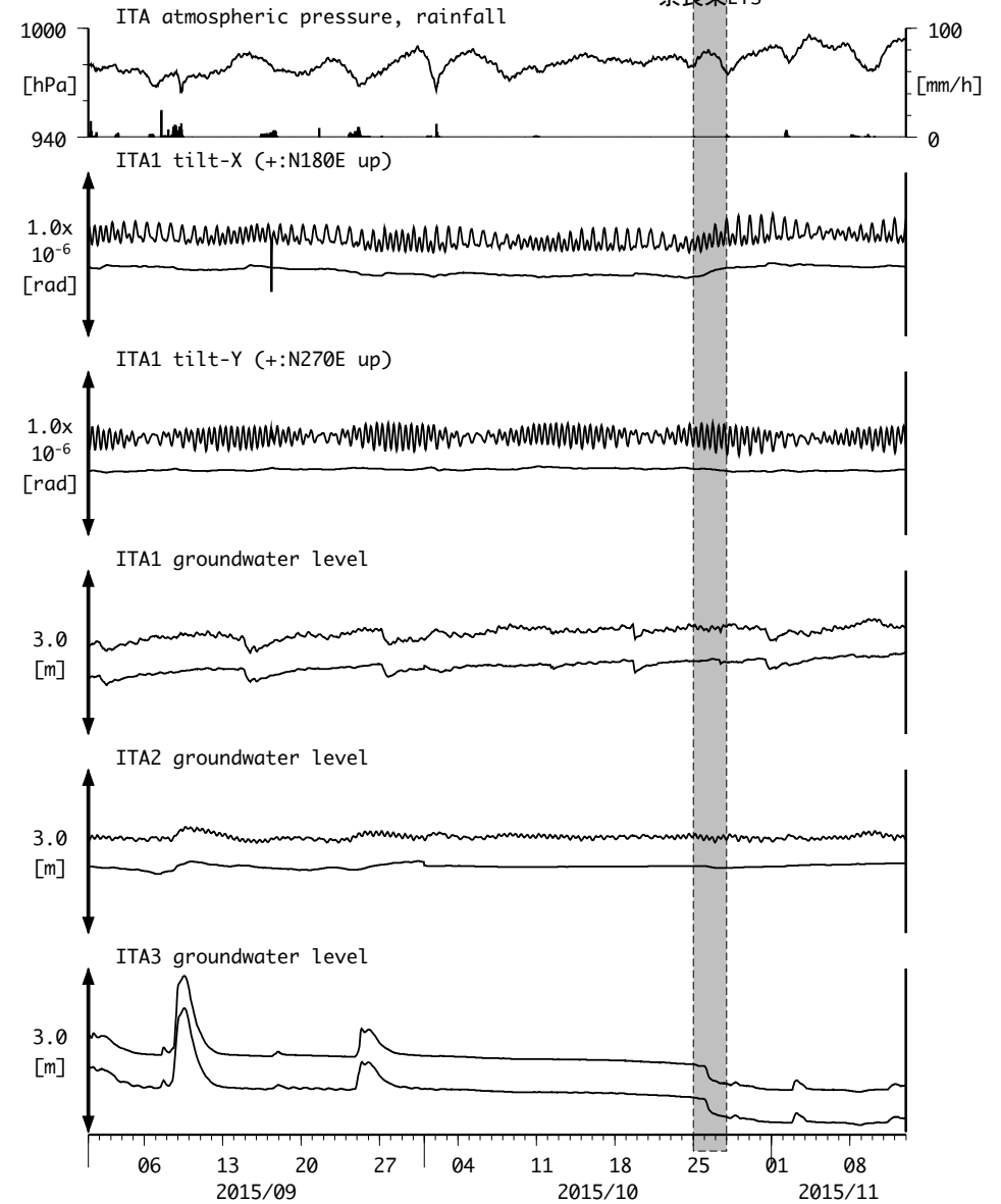
図12: Tilt and groundwater level changes at ITA 松阪飯高 (時間値) (2015/09/01 00:00 - 2015/11/13 00:00 (JST))
