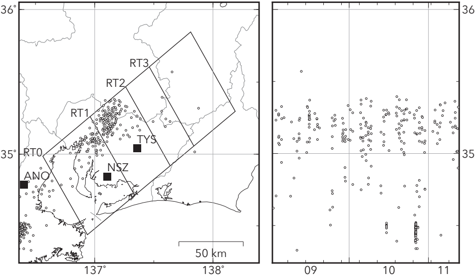
2015/09/01 00:00:00 - 2015/11/13 00:00:00 Total = 312 Deep low-frequency tremors in Tokai (日値) (2015/09/01 00:00 - 2015/11/13 00:00 (JST))
