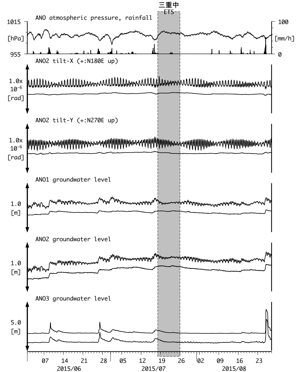
図10 : Tilt and groundwater level changes at ANO 津安濃 (時間値) (2015/06/01 00:00 - 2015/08/28 00:00 (JST))
