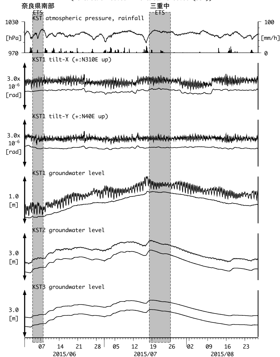
図20 : Tilt and groundwater level changes at KST 串本津荷 (時間値) (2015/06/01 00:00 - 2015/08/28 00:00 (JST))
