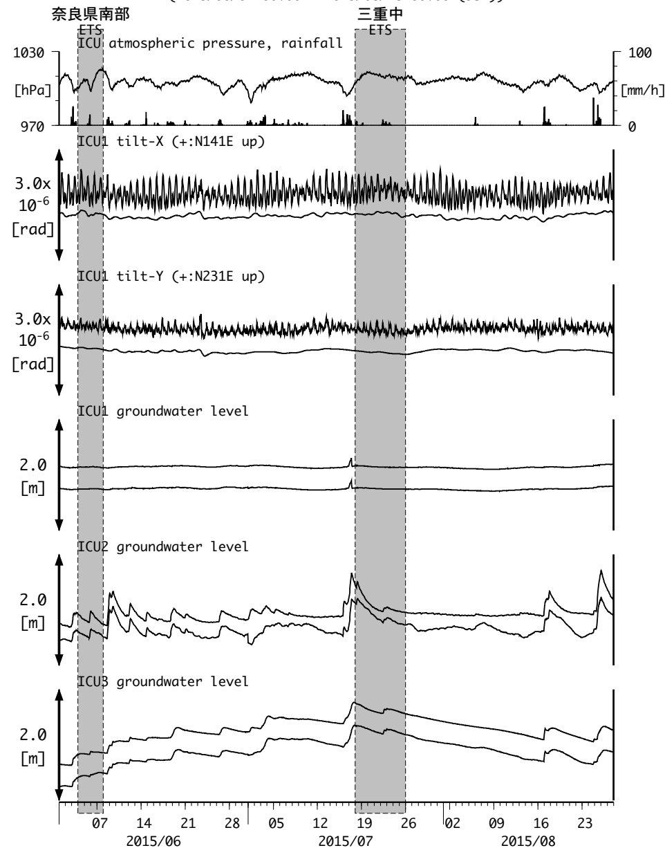
図16 : Tilt and groundwater level changes at ICU 熊野磯崎 (時間値) (2015/06/01 00:00 - 2015/08/28 00:00 (JST))
