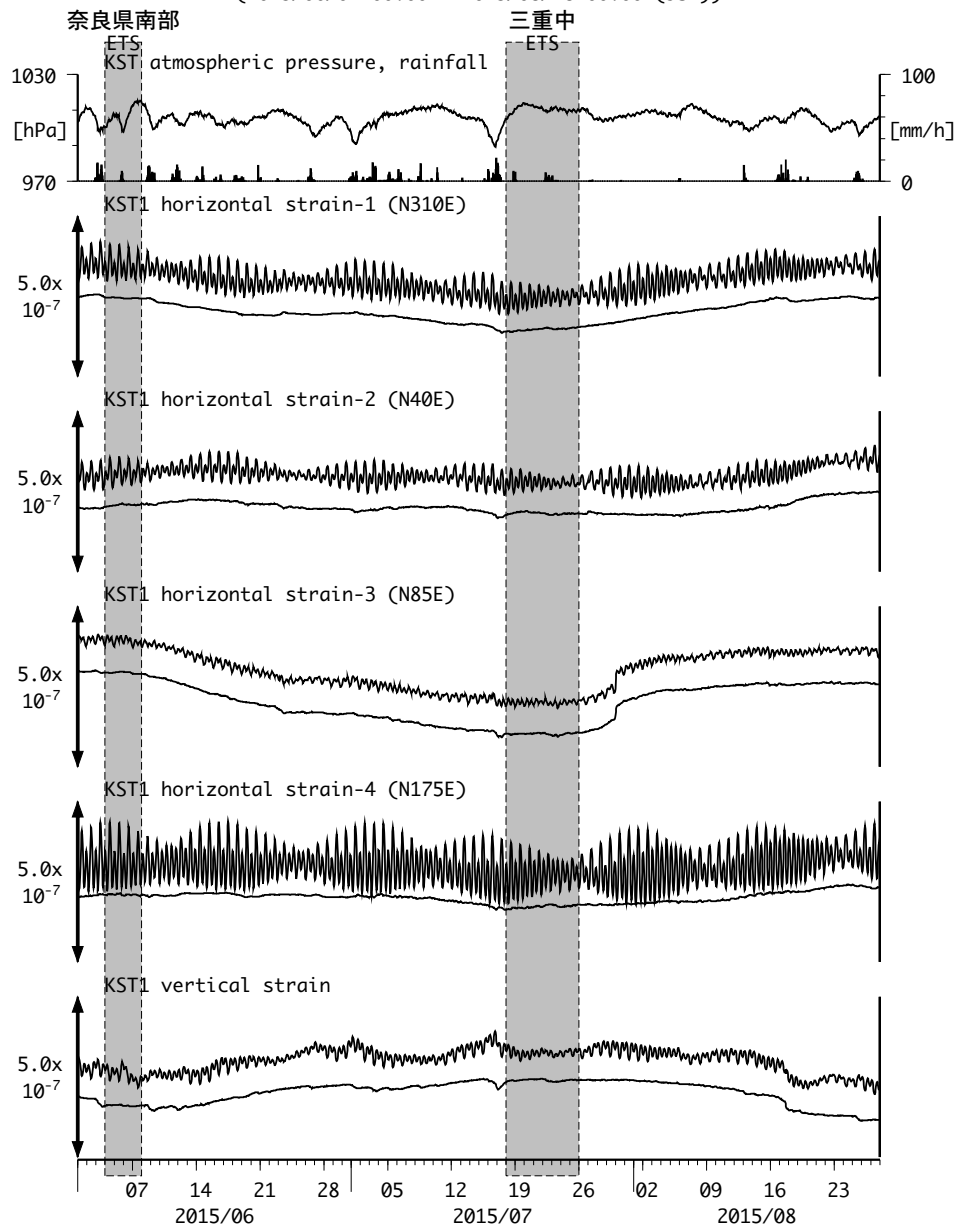
図19 : Crustal strain changes at KST 串本津荷 (時間値) (2015/06/01 00:00 - 2015/08/28 00:00 (JST))
