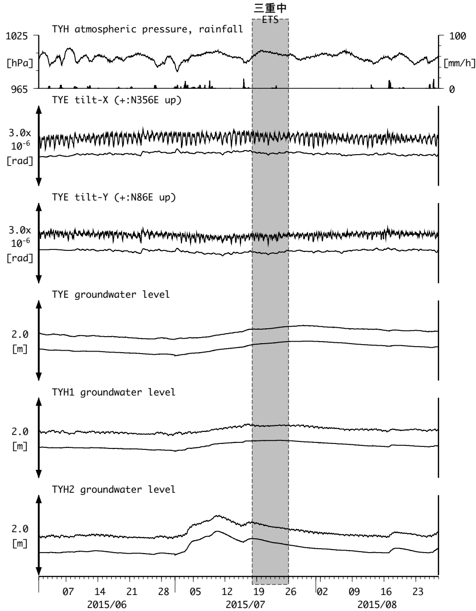
図7: Tilt and groundwater level changes at TYE and TYH 豊橋多米・豊橋 (2015/06/01 00:00 - 2015/08/28 00:00 (JST))
