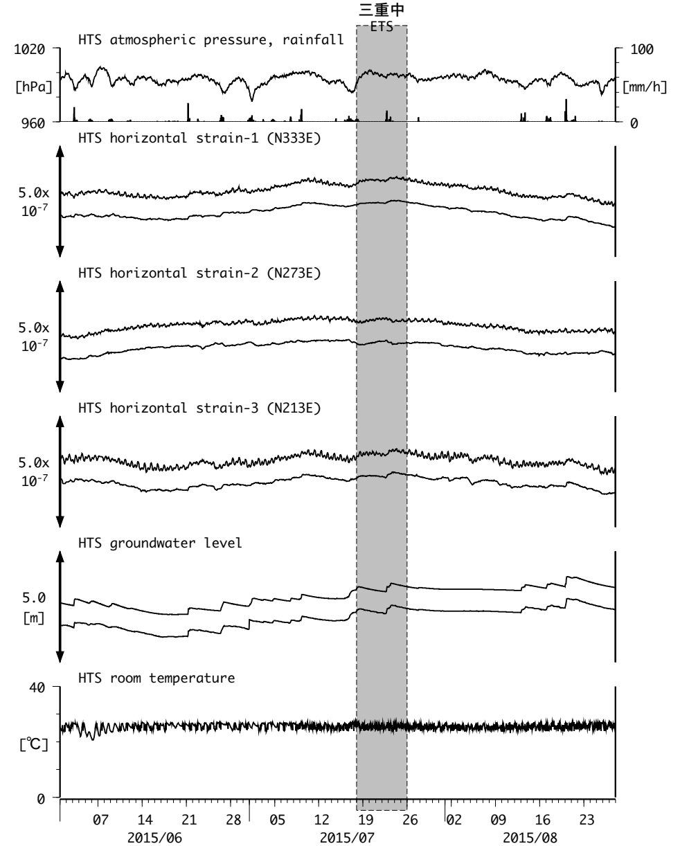
図8: Crustal strain and groundwater level changes at HTS 愛荘香之庄 (2015/06/01 00:00 - 2015/08/28 00:00 (JST))
