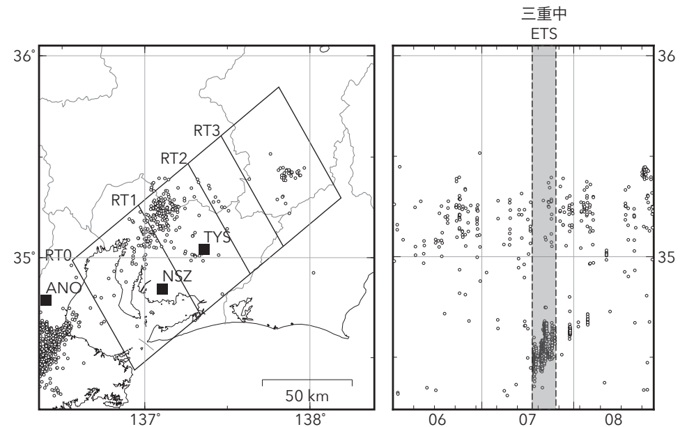
2015/06/01 00:00:00 - 2015/08/28 00:00:00 Total = 884 Deep low-frequency tremors in Tokai (日値) (2015/06/01 00:00 - 2015/08/28 00:00 (JST))
