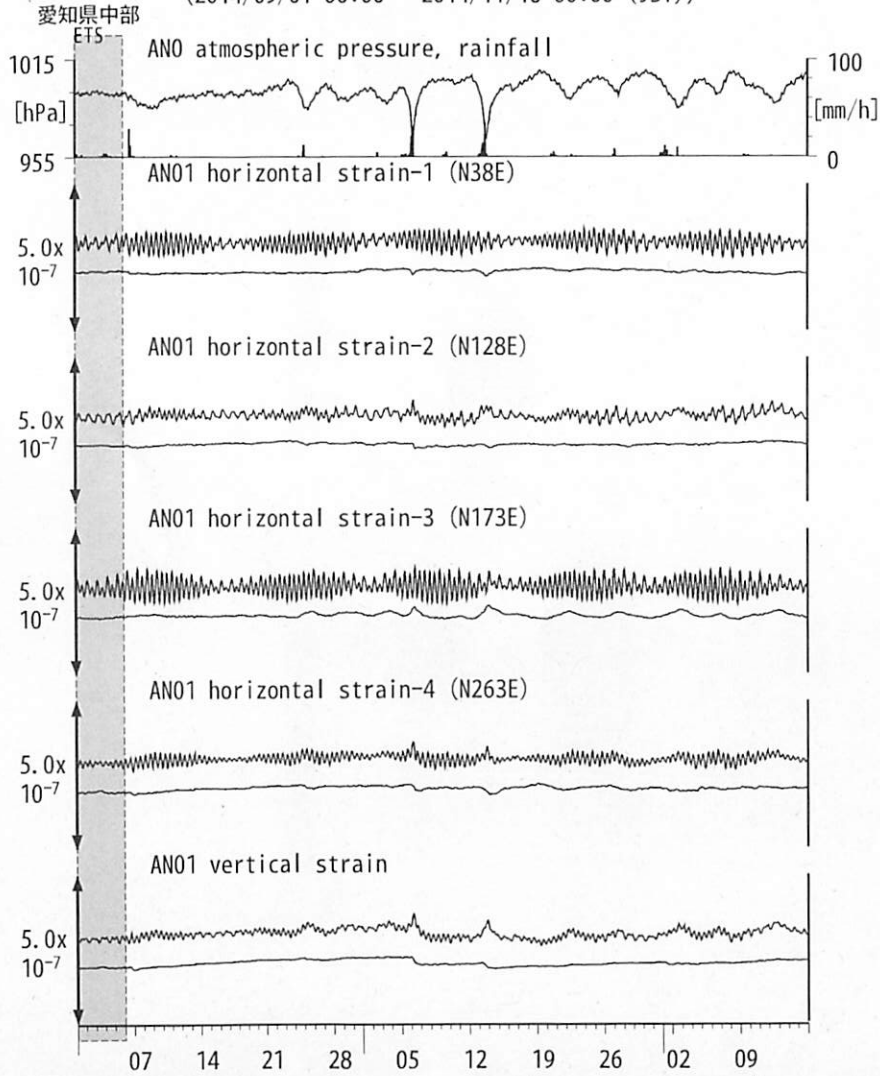
図9: Crustal strains changes at ANO 津安濃 (時間値) (2014/09/01 00:00 - 2014/11/16 00:00 (JST))
