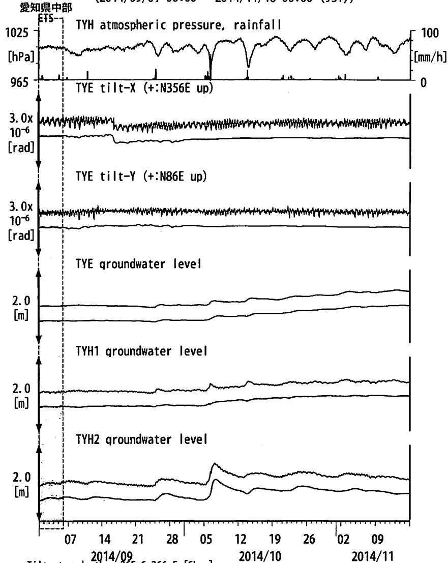
図7: Tilt and groundwater level changes at TYE and TYH 豊橋多米・豊橋 (2014/09/01 00:00 - 2014/11/16 00:00 (JST))
