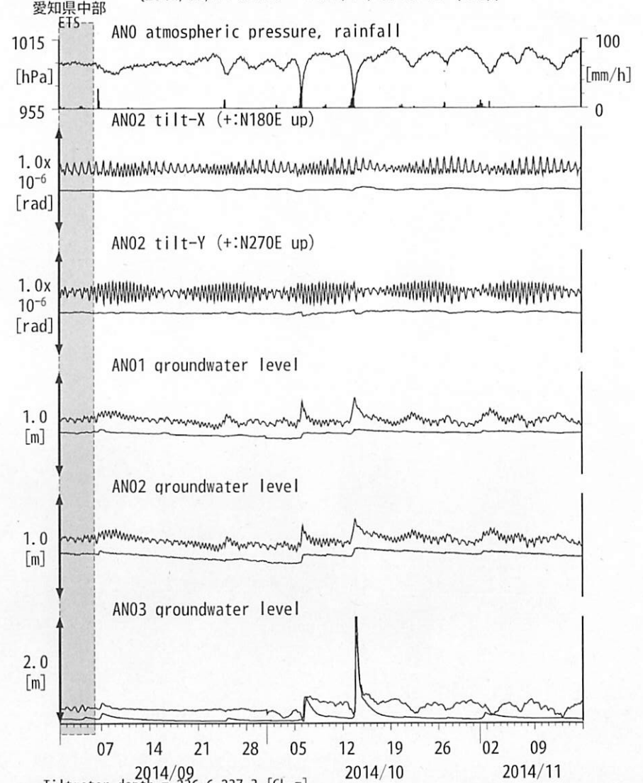
図10: Tilt and groundwater level changes at ANO 津安濃 (時間値) (2014/09/01 00:00 - 2014/11/16 00:00 (JST))
