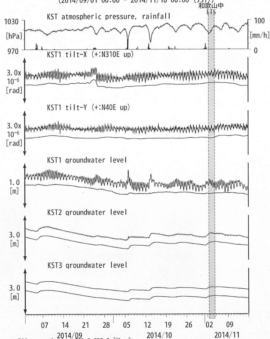
図20: Tilt and groundwater level changes at KST 串本津荷 (時間値) (2014/09/01 00:00 - 2014/11/16 00:00 (JST))
