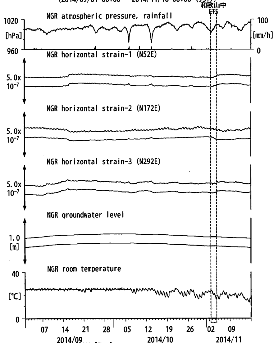
図21: Crustal strain and groundwater level changes at 岩出東坂本 (時間値) (2014/09/01 00:00 - 2014/11/16 00:00 (JST))
