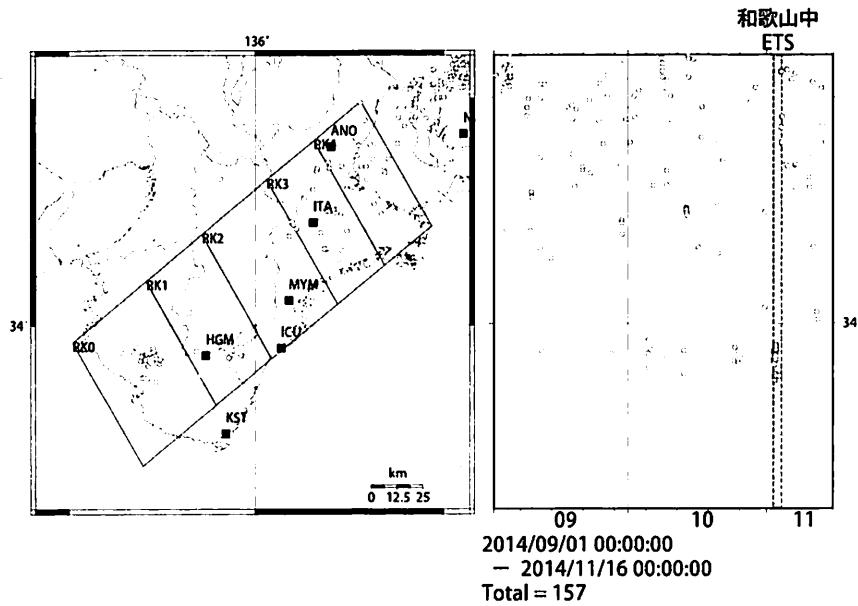
Deep low-frequency tremor activities in Kii Peninsula (日値) (2014/09/01 00:00 - 2014/11/16 00:00 (JST))
