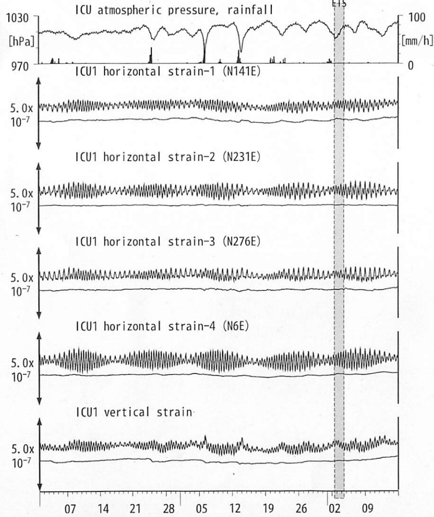
図15: Crustal strain changes at ICU 熊野磯崎 (時間値) (2014/09/01 00:00 - 2014/11/16 00:00 (JST))
