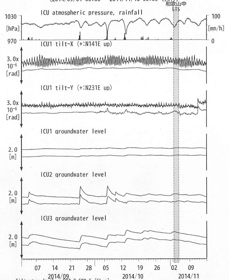
図16: Tilt and groundwater level changes at ICU 熊野磯崎 (時間値) (2014/09/01 00:00 - 2014/11/16 00:00 (JST))
