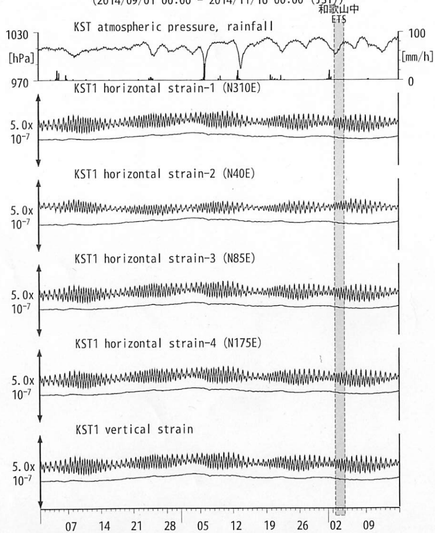
図19: Crustal strain changes at KST 串本津荷 (時間値) (2014/09/01 00:00 - 2014/11/16 00:00 (JST))
