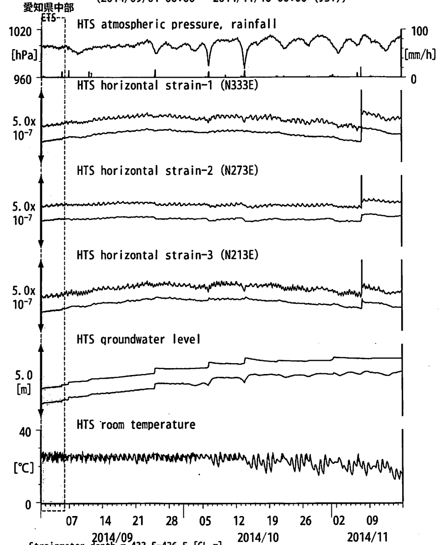
図8: Crustal strain and groundwater level changes at HTS 愛荘香之庄 (2014/09/01 00:00 - 2014/11/16 00:00 (JST))
