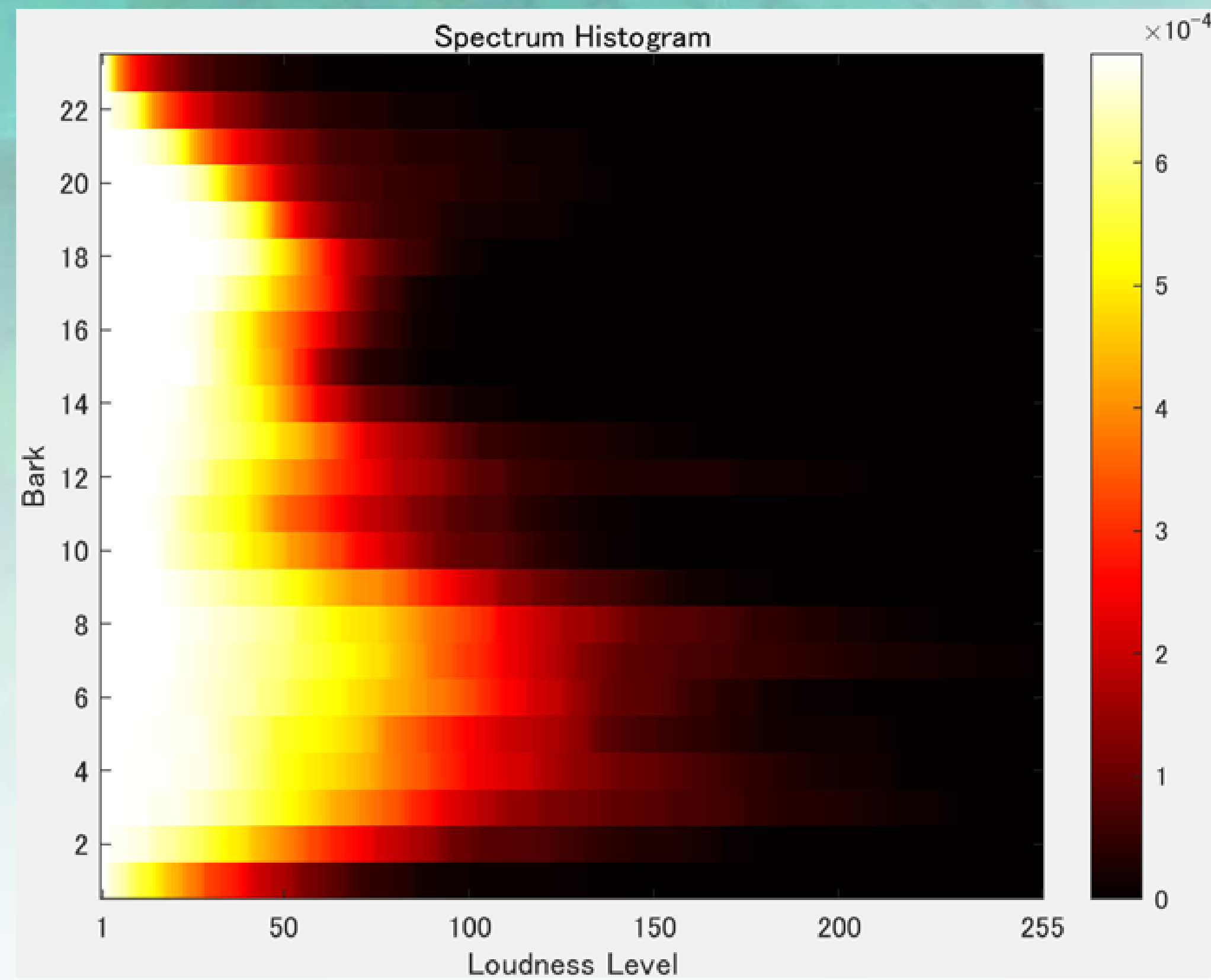
Spectrum histogram of a sonogram with Bark scale.
